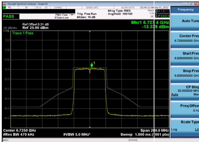
Plot 7-592. In-Band Emission Plot SDM Antenna 4a (40MHz 802.11ax RU2484 (UNII Band 7) – Ch. 155)
