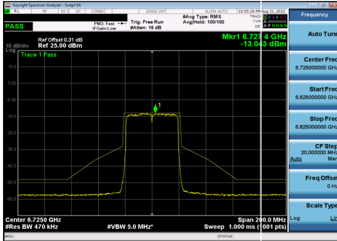
Plot 7-591. In-Band Emission Plot SDM Antenna 5b (40MHz 802.11ax RU2484 (UNII Band 7) – Ch. 155)
