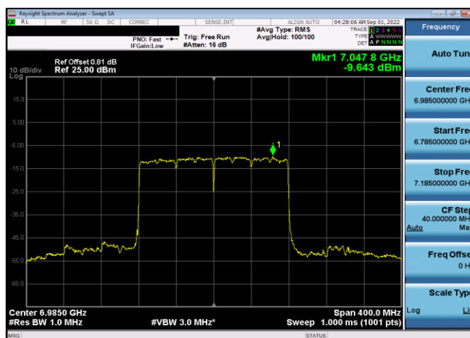
Plot 7-384. Power Spectral Density Plot SDM Antenna 4a (160MHz 802.11ax RU484 (UNII Band 8) – Ch. 207)
