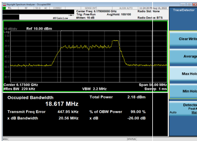
Plot 7-3. 26dB & 99% Bandwidth Plot Antenna 5b (20MHz 802.11ax RU26 (UNII Band 5) – Ch. 45)
