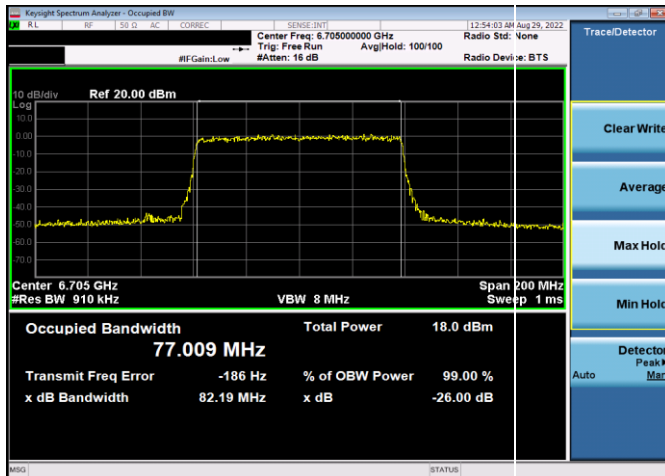
Plot 7-44. 26dB & 99% Bandwidth Plot Antenna 5b (80MHz 802.11ax RU996 (UNII Band 7) – Ch. 151)
