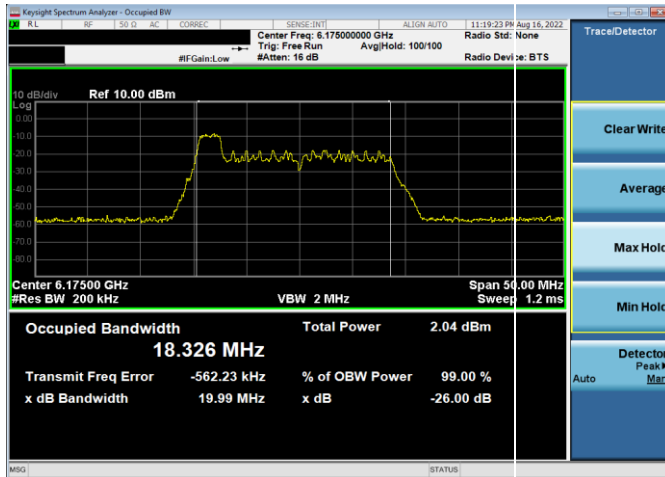
Plot 7-1. 26dB & 99% Bandwidth Plot Antenna 5b (20MHz 802.11ax RU26 (UNII Band 5) – Ch. 45)
