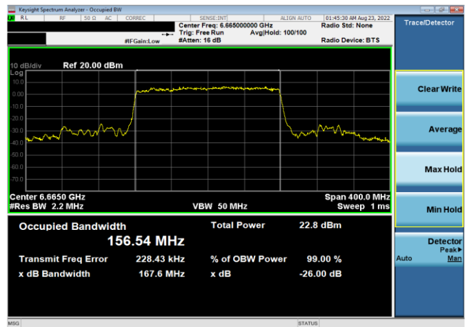
Plot 7-48. 26dB & 99% Bandwidth Plot Antenna 5b (160MHz 802.11ax RU484 (UNII Band 7) – Ch. 143)
