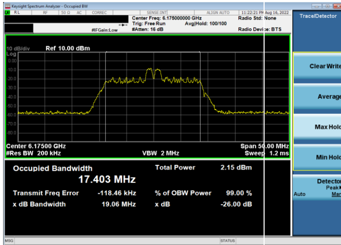
Plot 7-2. 26dB & 99% Bandwidth Plot Antenna 5b (20MHz 802.11ax RU26 (UNII Band 5) – Ch. 45)
