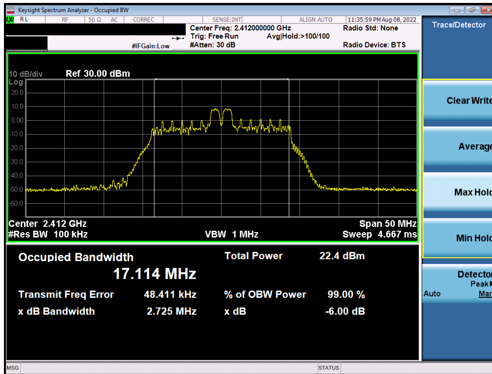
Plot 7-14. 6dB BW & 99% OBW Plot Antenna 2a (802.11ax OFDMA – RU26 Index 4 – Ch. 1)
