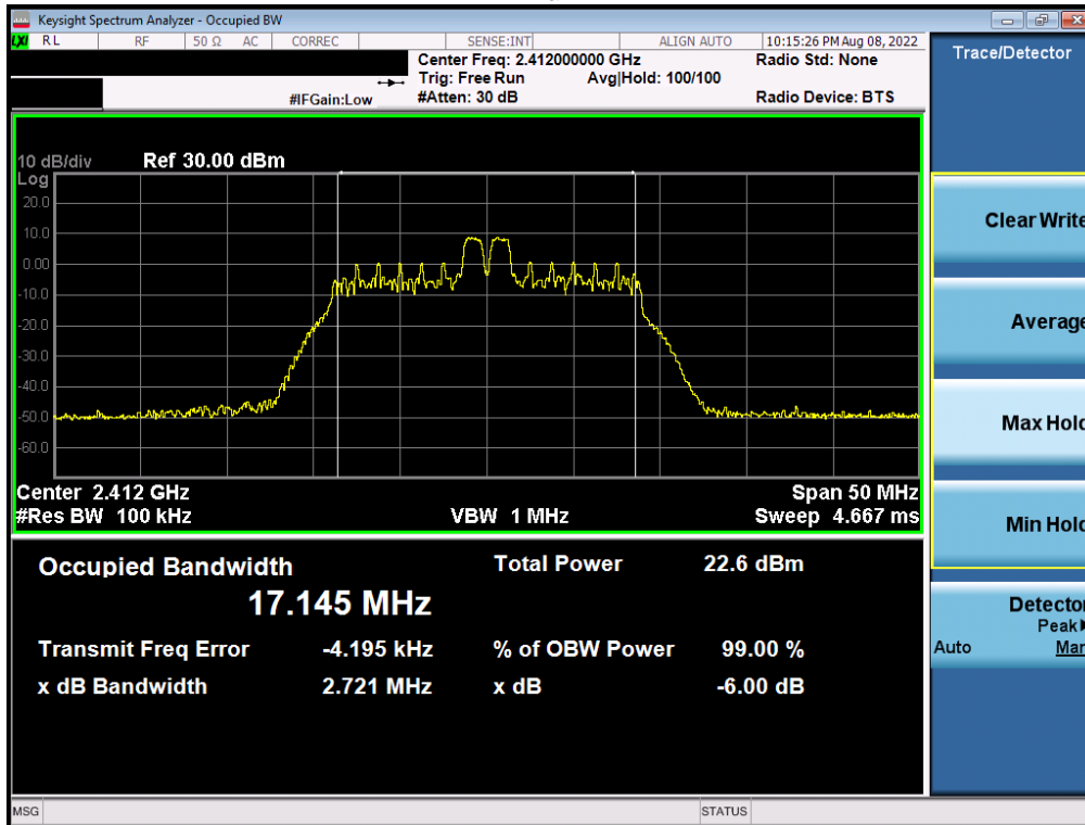
Plot 7-2. 6dB BW & 99% OBW Plot Antenna 4a (802.11ax OFDMA – RU26 Index 4 – Ch. 1)
