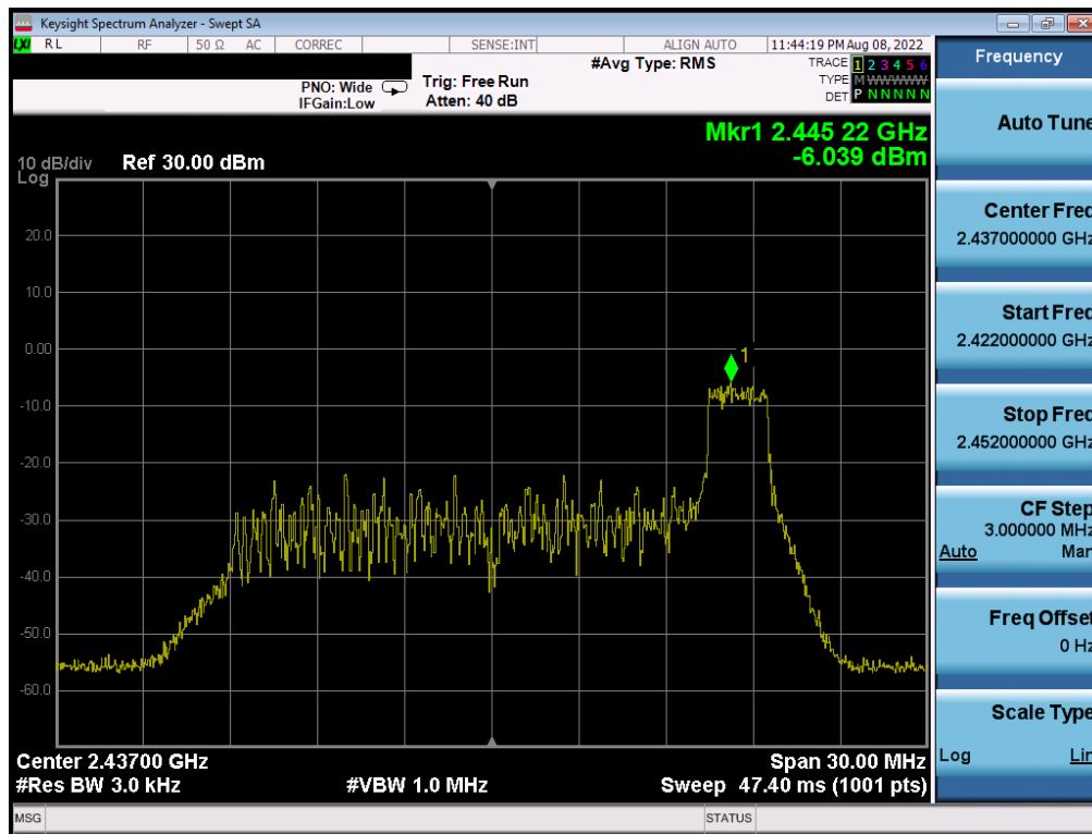
Plot 7-42. Power Spectral Density Plot Antenna 2a (802.11ax OFDMA – RU26 Index 8 – Ch. 6)
