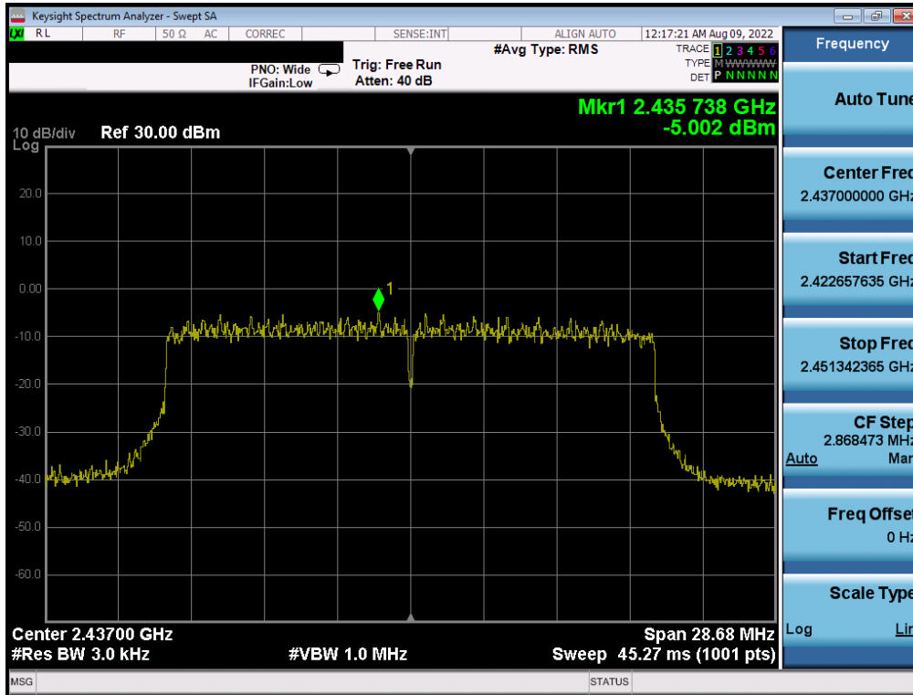
Plot 7-47. Power Spectral Density Plot Antenna 2a (802.11ax OFDMA – RU242 – Ch. 6)
