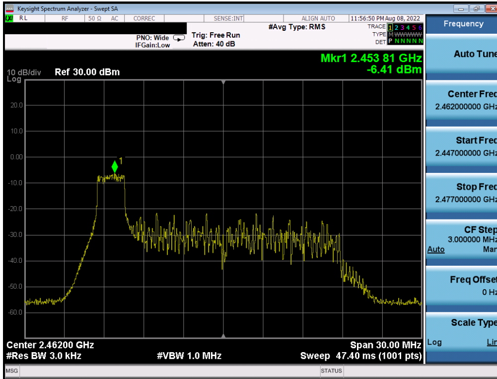
Plot 7-43. Power Spectral Density Plot Antenna 2a (802.11ax OFDMA – RU26 Index 0 – Ch. 11)
