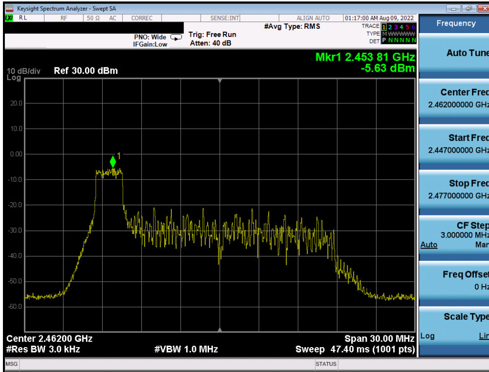
Plot 7-61. Power Spectral Density Plot CDD Antenna 4a (802.11ax OFDMA – RU26 Index 0 – Ch. 11)
