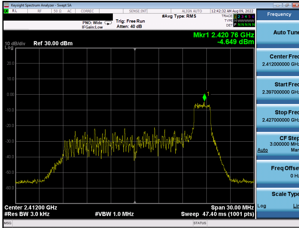
Plot 7-53. Power Spectral Density Plot CDD Antenna 4a (802.11ax OFDMA – RU26 Index 8 – Ch. 1)
