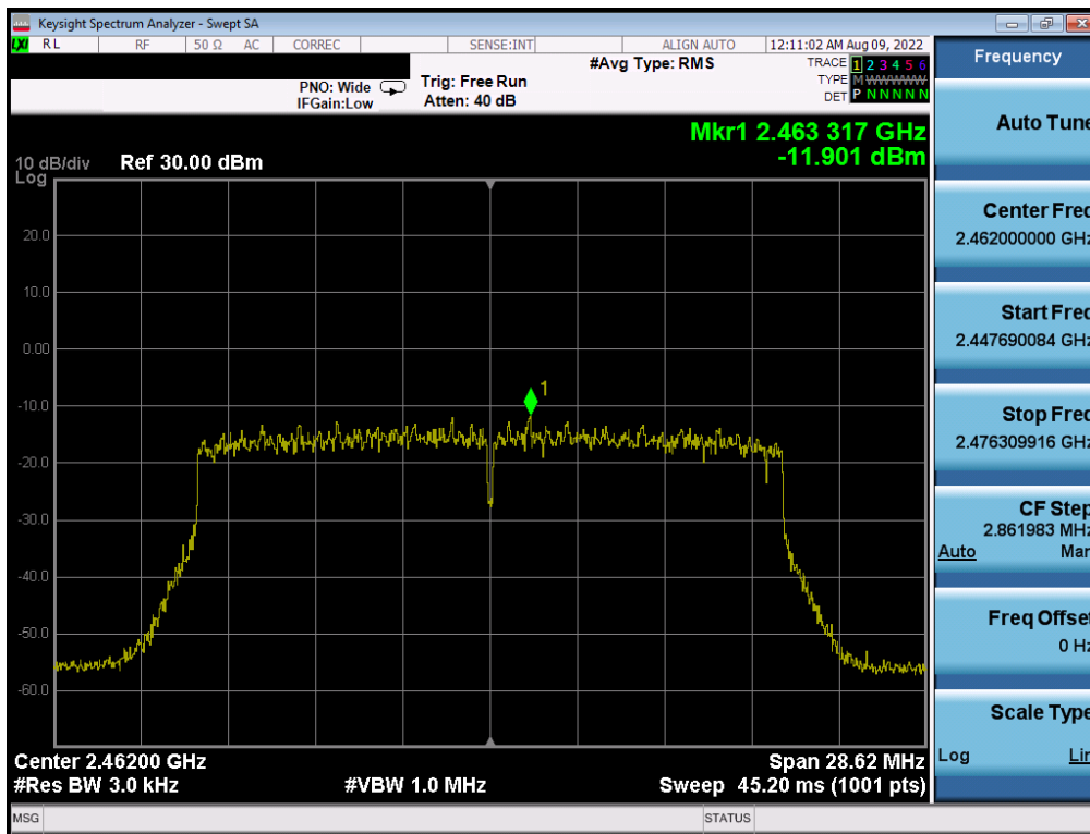
Plot 7-48. Power Spectral Density Plot Antenna 2a (802.11ax OFDMA – RU242 – Ch. 11)
