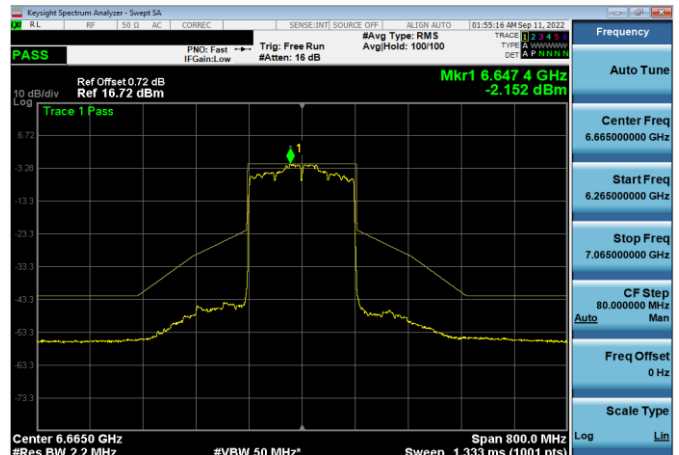
Plot 7-411. In-Band Emission Plot Antenna WF5b (160MHz 802.11ax (UNII Band 7) – Ch. 143, MCS2)
