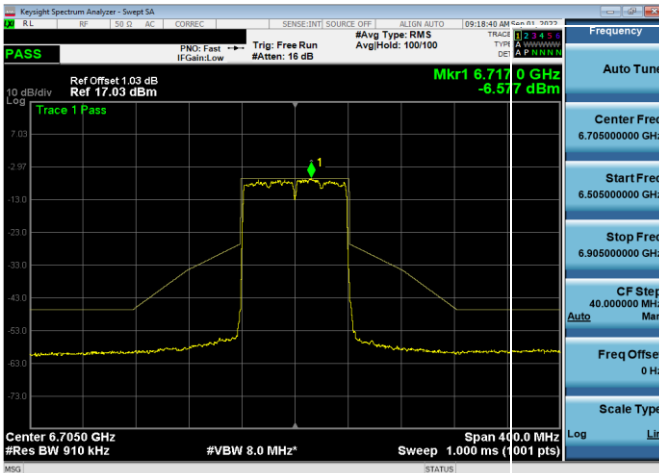
Plot 7-386. In-Band Emission Plot Antenna WF5t (80MHz 802.11ax (UNII Band 7) – Ch. 151, MCS11)
