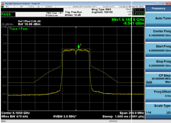
Plot 7-375. In-Band Emission Plot Antenna WF5t (40MHz 802.11ax (UNII Band 5) – Ch. 43, MCS11)
