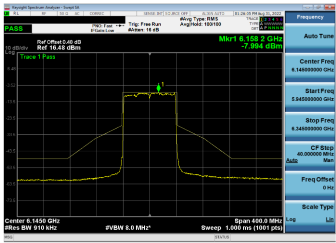
Plot 7-400. In-Band Emission Plot Antenna WF5b (80MHz 802.11ax (UNII Band 5) – Ch. 39, MCS2)
