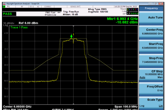
Plot 7-412. In-Band Emission Plot Antenna WF5b (20MHz 802.11a (UNII Band 8) – Ch. 209, MCS2)
