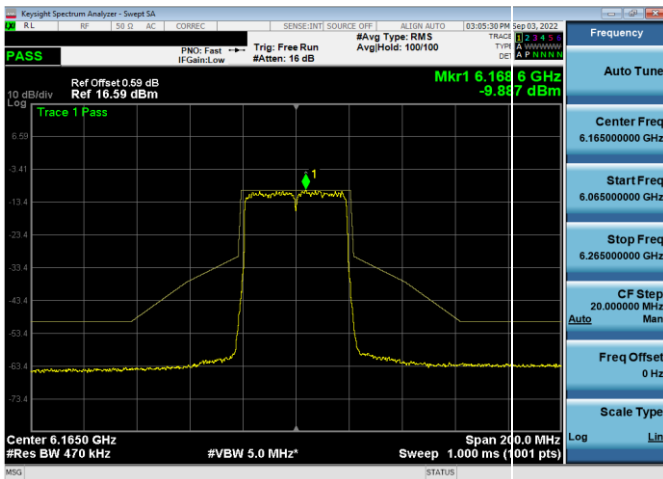
Plot 7-419. In-Band Emission Plot Antenna WF5b (40MHz 802.11ax (UNII Band 5) – Ch. 43, MCS4)
