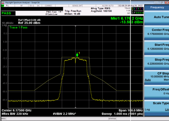
Plot 7-337. In-Band Emission Plot Antenna WF5t (20MHz 802.11a (UNII Band 5) – Ch. 45, MCS2)
