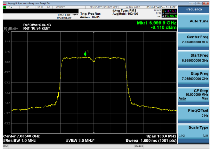
Plot 7-332. Power Spectral Density Plot SDM Antenna WF5t (40MHz 802.11ax (UNII Band 8) – Ch. 211, MCS11)
