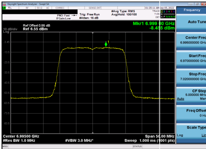
Plot 7-330. Power Spectral Density Plot SDM Antenna WF5t (20MHz 802.11ax (UNII Band 8) – Ch. 209, MCS11)
