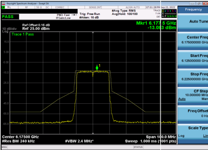
Plot 7-338. In-Band Emission Plot Antenna WF5t (20MHz 802.11ax (UNII Band 5) – Ch. 45, MCS2)
