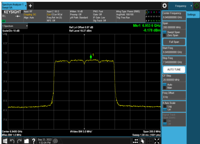
Plot 7-334. Power Spectral Density Plot SDM Antenna WF5t (80MHz 802.11ax (UNII Band 8) – Ch. 199, MCS11)
