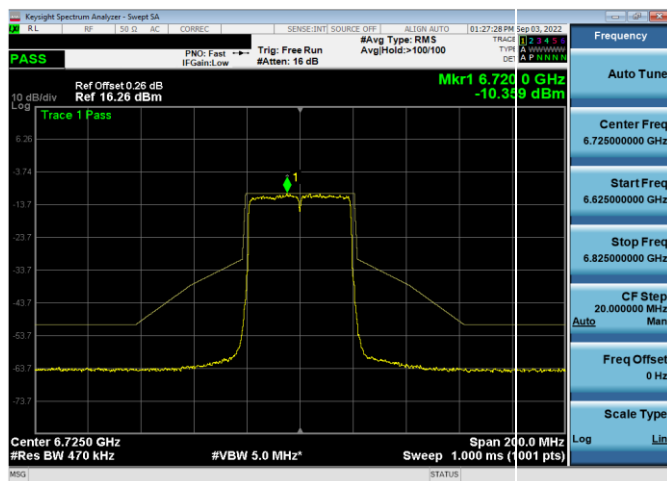
Plot 7-349. In-Band Emission Plot Antenna WF5t (40MHz 802.11ax (UNII Band 7) – Ch. 155, MCS2)
