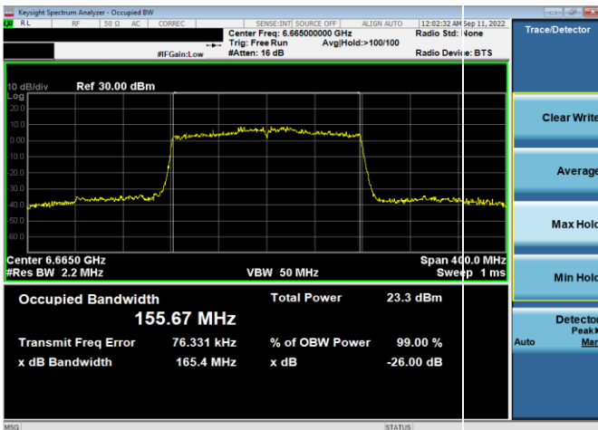
Plot 7-35. 26dB & 99% Bandwidth Plot Antenna WF5t (160MHz 802.11ax (UNII Band 7) – Ch. 143, MCS4)
