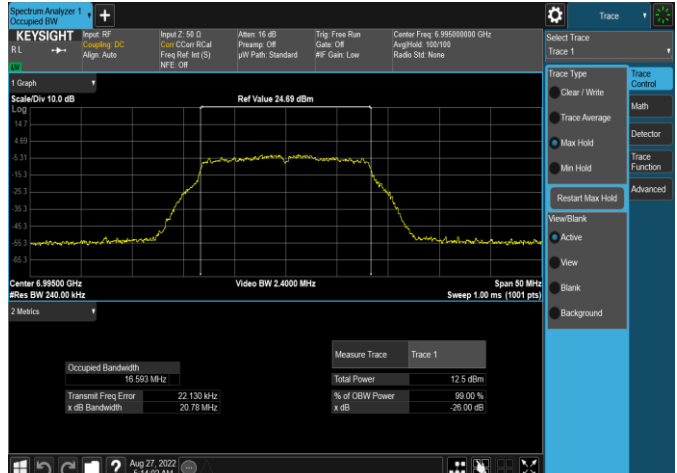
Plot 7-16. 26dB & 99% Bandwidth Plot Antenna WF5t (20MHz 802.11a (UNII Band 8) – Ch. 209, 12Mbps)
