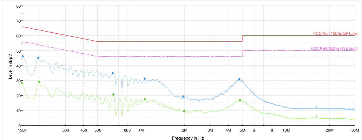
Plot 7-745. AC Line Conducted Plot with 802.11ax SDM – Ch. 56 (N), with AC/DC adapter
