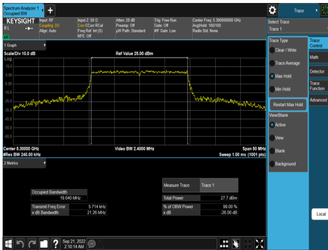
Plot 7-20. 26dB BW & 99% OBW Antenna WF5T (20MHz BW 11ax – RU242 – Ch.60)
