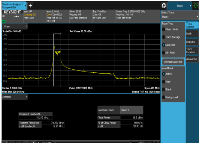
Plot 7-41. 26dB BW & 99% OBW Antenna WF5T (160MHz BW 11ax Index 0 – RU26 – Ch.114(L))
