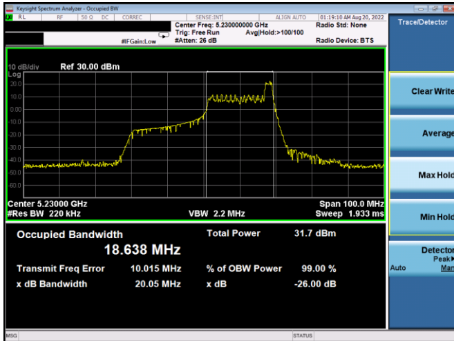
Plot 7-51. 26dB BW & 99% OBW Antenna WF5B (40MHz BW 11ax Index 17 - RU26 - Ch.46)
