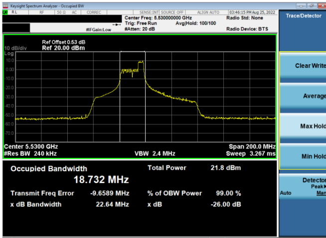
Plot 7-38. 26dB BW & 99% OBW Antenna WF5T (80MHz BW 11ax Index 44 – RU52 – Ch.106)
