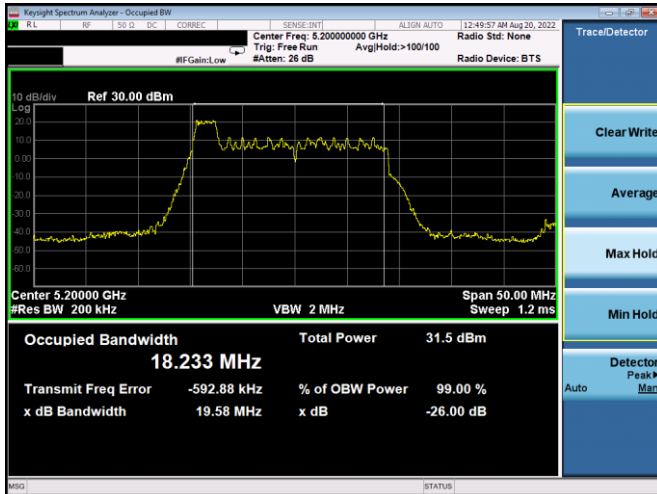
Plot 7-45. 26dB BW & 99% OBW Antenna WF5B (20MHz BW 11ax Index 0 – RU26 – Ch.40)
