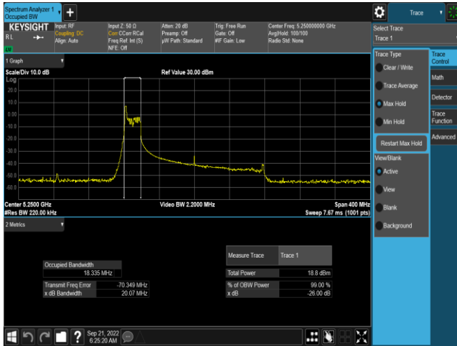
Plot 7-13. 26dB BW & 99% OBW Antenna WF5T (160MHz BW 11ax Index 0 – RU26 – Ch.50(L))
