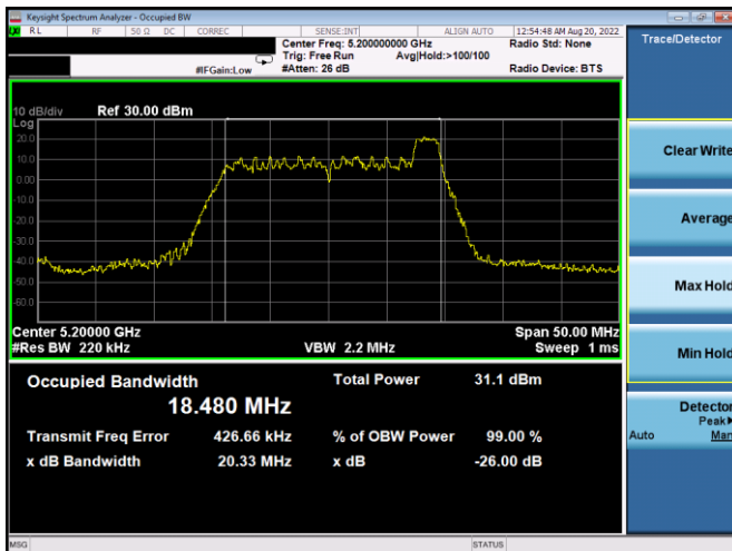
Plot 7-47. 26dB BW & 99% OBW Antenna WF5B (20MHz BW 11ax Index 8 – RU26 – Ch.40)
