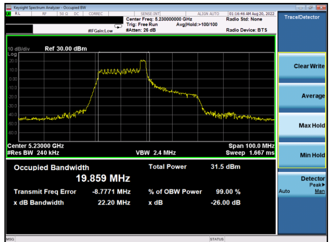
Plot 7-50. 26dB BW & 99% OBW Antenna WF5B (40MHz BW 11ax Index 8 – RU26 – Ch.46)
