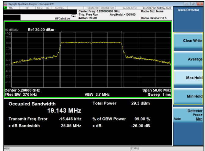
Plot 7-48. 26dB BW & 99% OBW Antenna WF5B (20MHz BW 11ax – RU242 – Ch.40)
