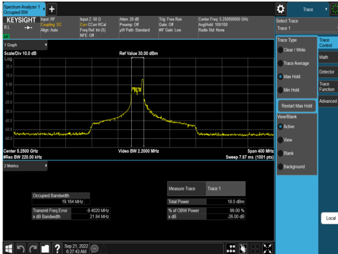
Plot 7-14. 26dB BW & 99% OBW Antenna WF5T (160MHz BW 11ax Index 36 – RU26 – Ch.50(L))
