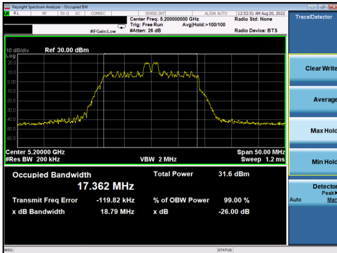
Plot 7-46. 26dB BW & 99% OBW Antenna WF5B (20MHz BW 11ax Index 4 – RU26 – Ch.40)
