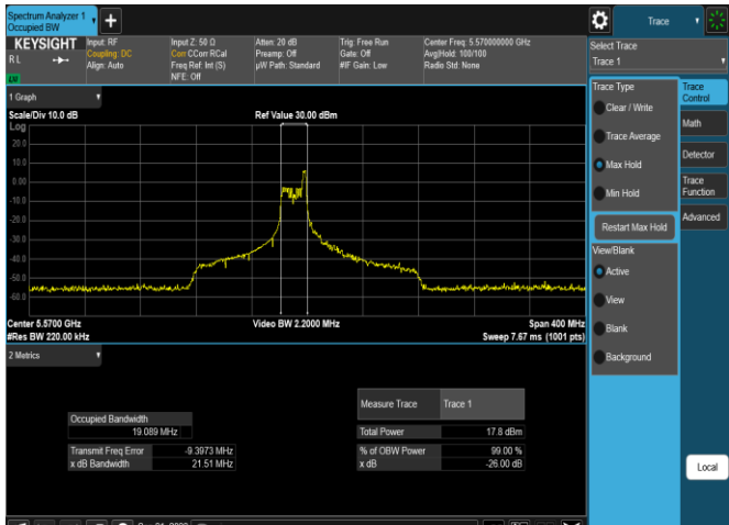
Plot 7-42. 26dB BW & 99% OBW Antenna WF5T (160MHz BW 11ax Index 36 – RU26 – Ch.114(L))
