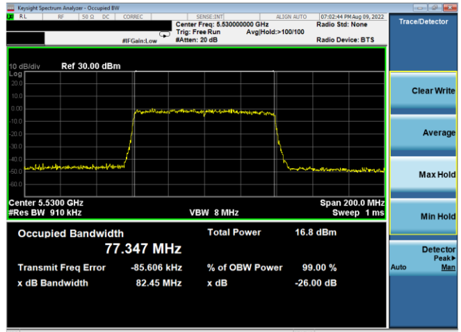
Plot 7-40. 26dB BW & 99% OBW Antenna WF5T (80MHz BW 11ax – RU996 – Ch.106)
