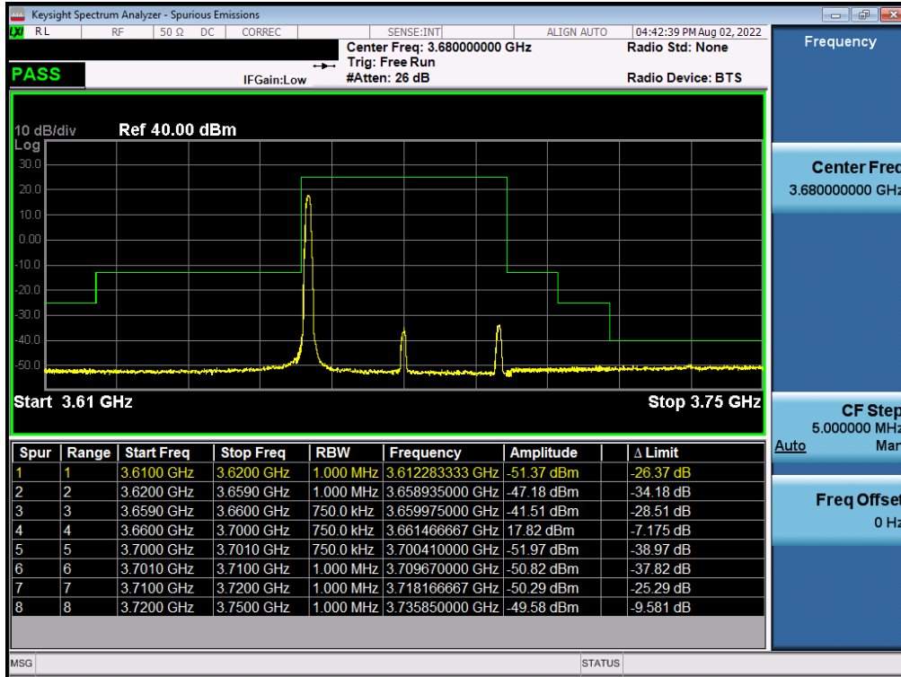
Plot 7-36. Channel Edge Plot (NR Band n48 - 40MHz QPSK - High Channel)
