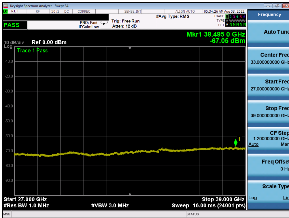
Plot 7-27. Conducted Spurious Plot (NR Band n48 - 40MHz QPSK - High Channel)
