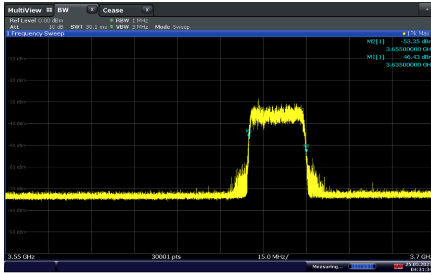
Plot 7-57. Run#2 End User Device Frequency of Operations
