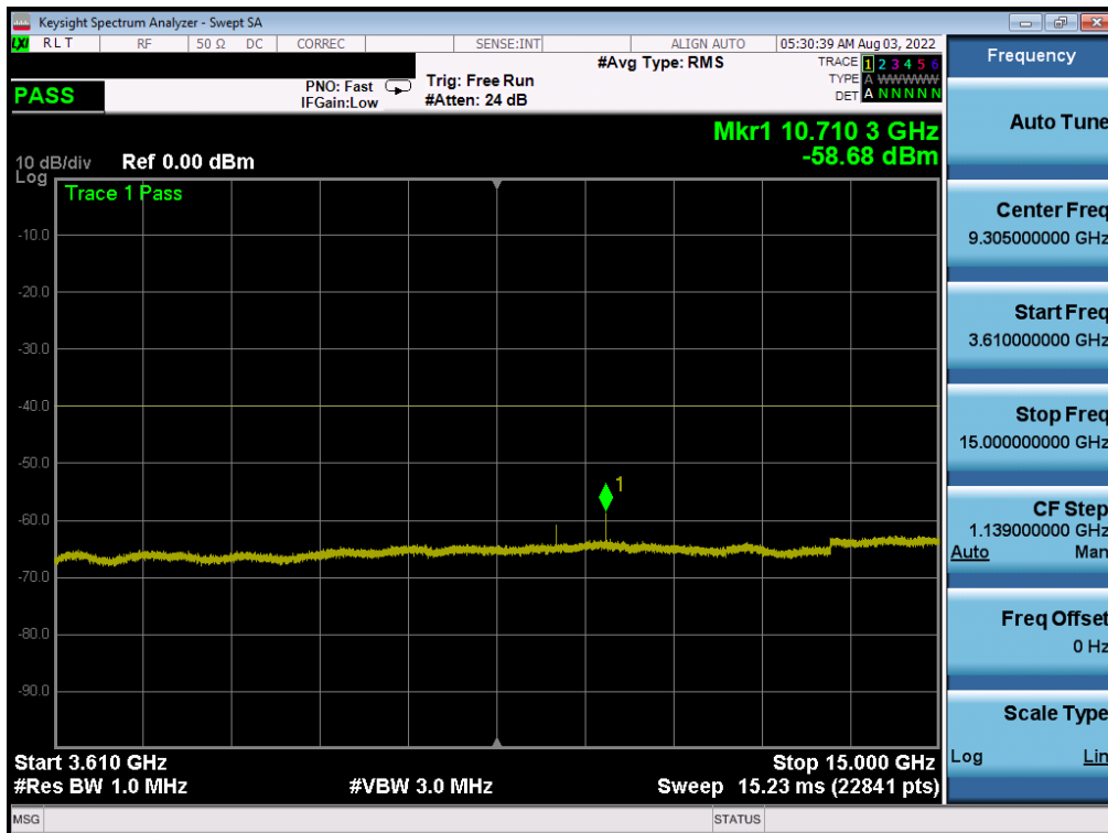
Plot 7-17. Conducted Spurious Plot (NR Band n48 - 40MHz QPSK - Low Channel)
