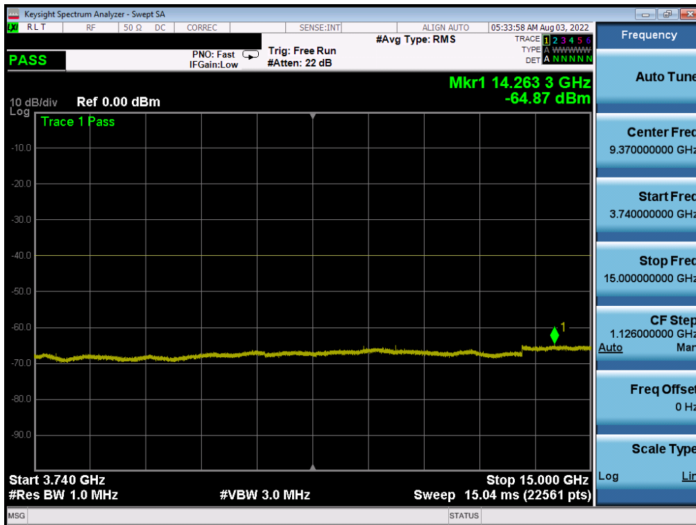
Plot 7-25. Conducted Spurious Plot (NR Band n48 - 40MHz QPSK - High Channel)
