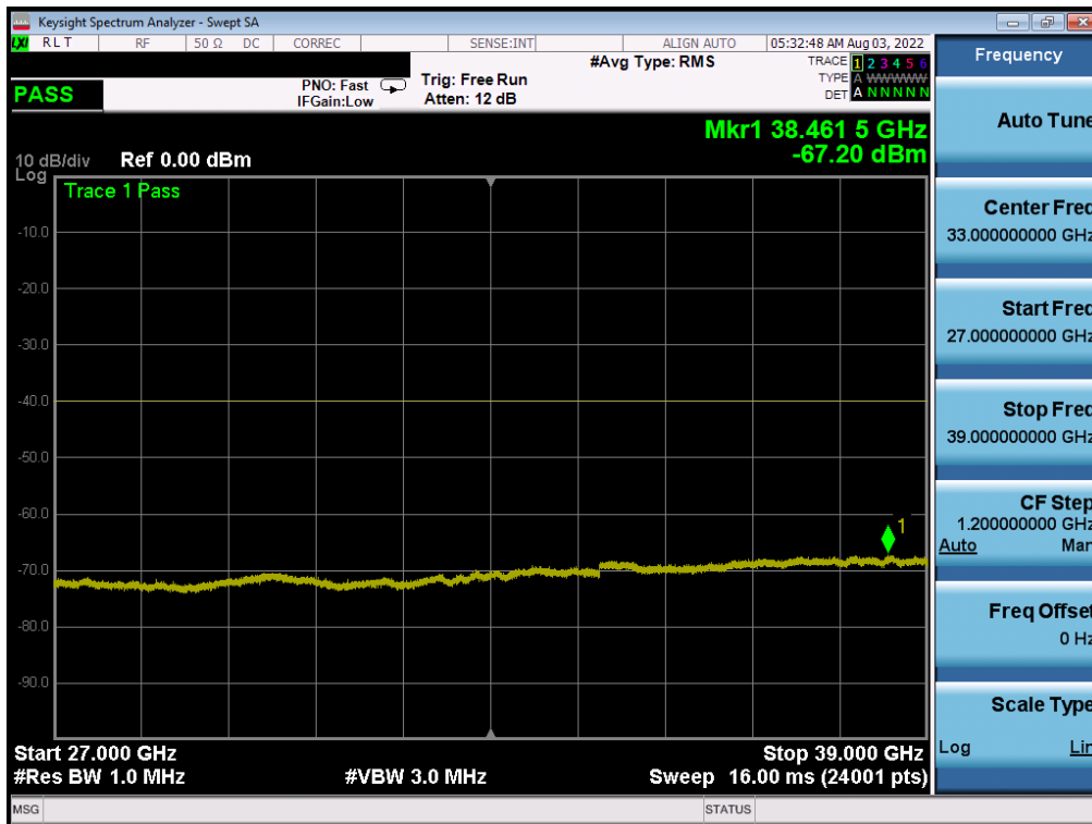
Plot 7-23. Conducted Spurious Plot (NR Band n48 - 40MHz QPSK - Mid Channel)
