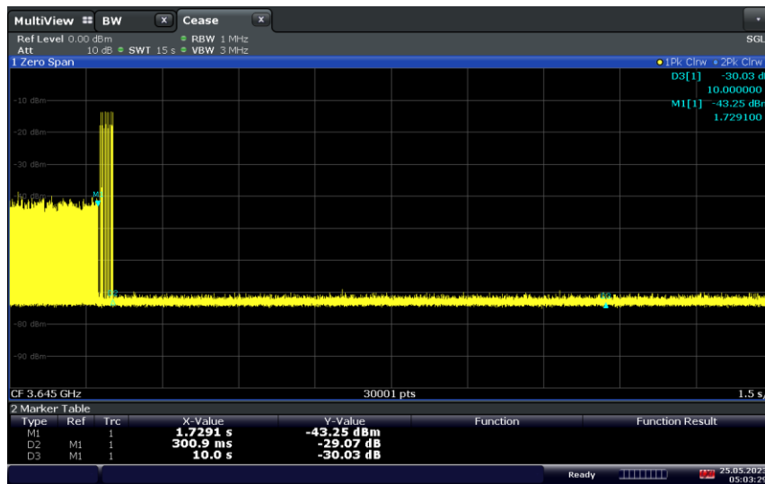
Plot 7-58. Run#2 End User Device Discontinues Operations within 10s
