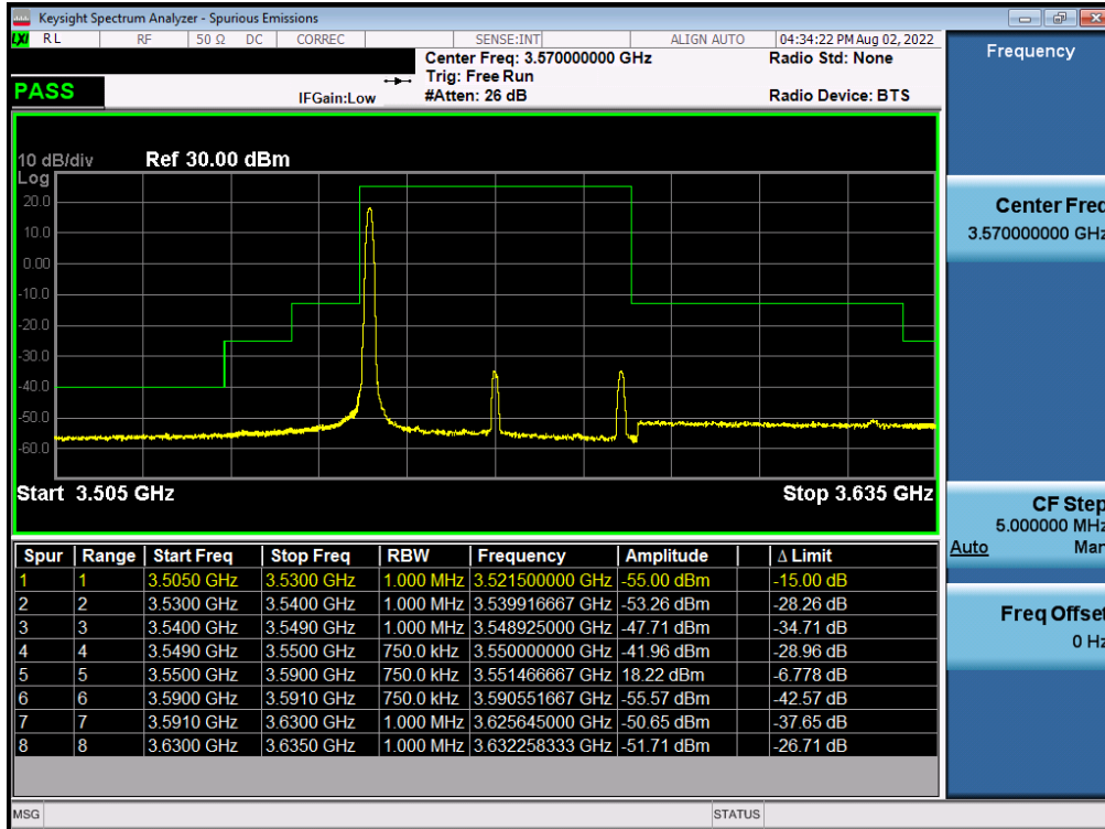
Plot 7-34. Channel Edge Plot (NR Band n48 - 40MHz QPSK - Low Channel)
