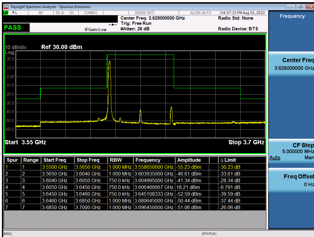
Plot 7-35. Channel Edge Plot (NR Band n48 - 40MHz QPSK - Mid Channel)
