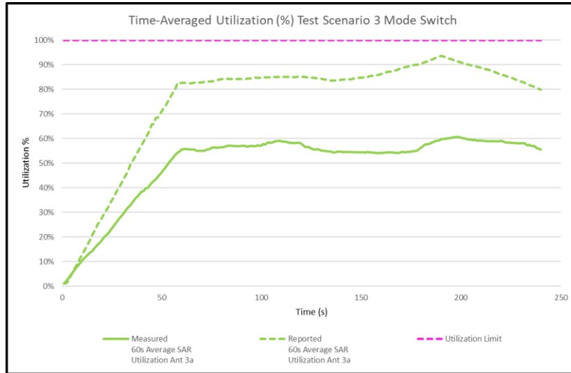
Figure J-7 60s Average Utilization vs. Time during Mode Switch
