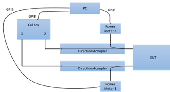
(b) Appendix D – Test Setup Photo 4
