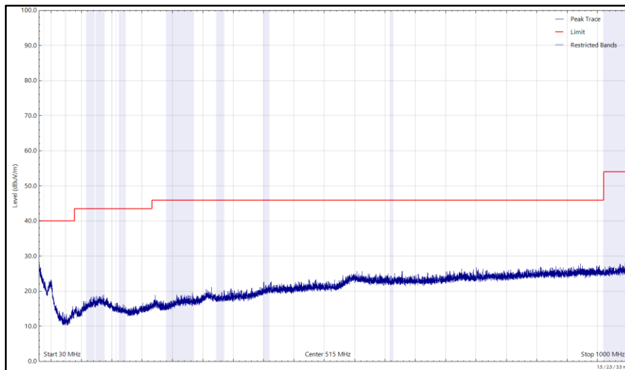
Figure 288 - U-NII-3 - 5825 MHz (CH165), 802.11a, Core 0, 30 MHz to 1 GHz, Vertical (Peak)
