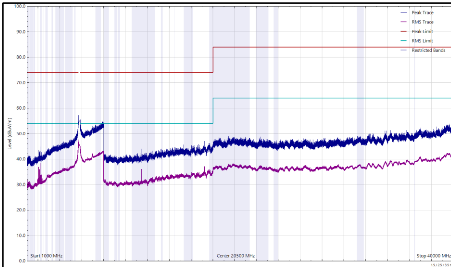
Figure 333 - U-NII-3 - 5745 MHz (CH149), HE20, RU26-0, CDD, Core 0 + Core 1, 1 GHz to 40 GHz, Vertical
