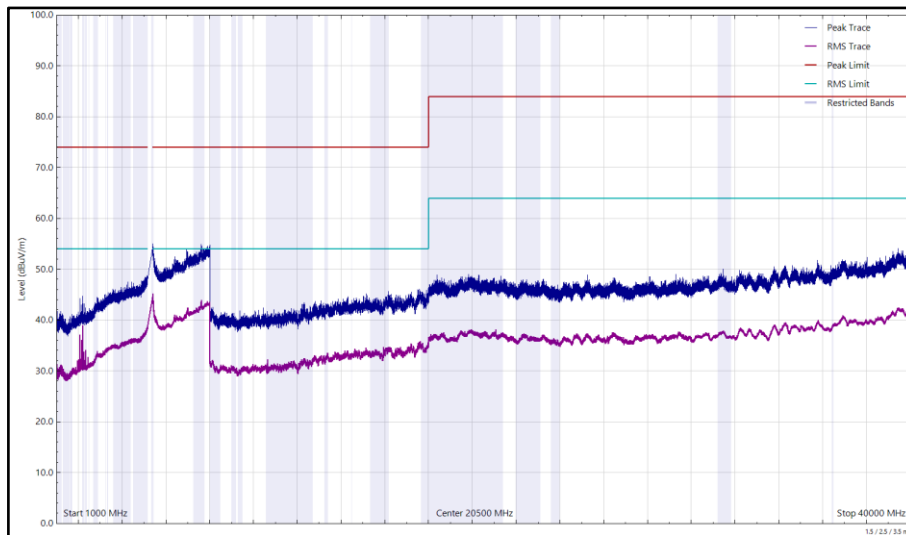
Figure 327 - U-NII-2A - 5320 MHz (CH64), HE20, RU52-37, CDD, Core 0 + Core 1, 1 GHz to 40 GHz, Vertical
