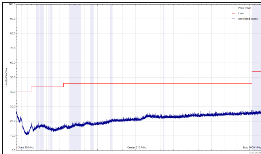
Figure 320 - U-NII-3 - 5825 MHz (CH165), VHT20, CDD, Core 0 + Core 1, 30 MHz to 1 GHz, Vertical (Peak)
