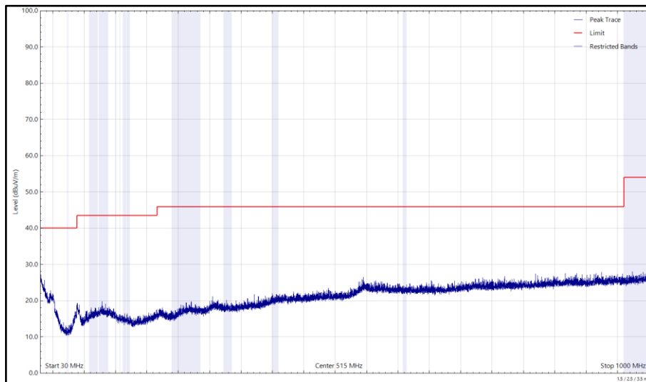
Figure 324 - U-NII-1 - 5180 MHz (CH36), HE20, RU26-0, CDD, Core 0 + Core 1, 30 MHz to 1 GHz, Vertical (Peak)
