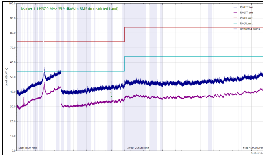
Figure 326 - U-NII-2A - 5320 MHz (CH64), HE20, RU52-37, CDD, Core 0 + Core 1, 1 GHz to 40 GHz, Horizontal
