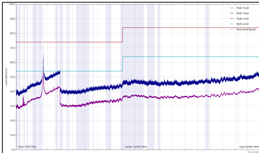
Figure 275 - U-NII-1 - 5180 MHz (CH36), 802.11a, Core 0, 1 GHz to 40 GHz, Horizontal
