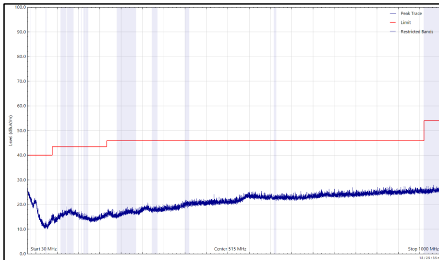
Figure 304 - U-NII-3 - 5825 MHz (CH165), 802.11a, Core 1, 30 MHz to 1 GHz, Vertical (Peak)
