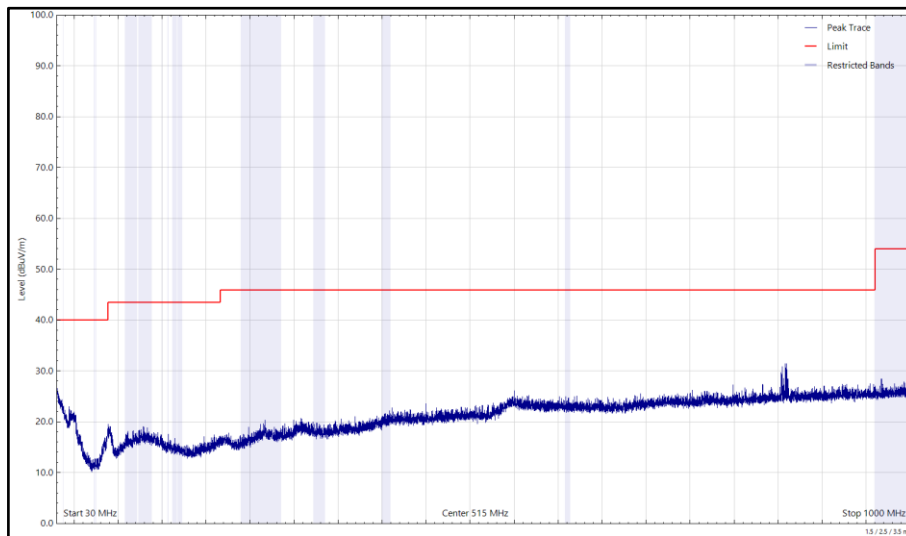
Figure 336 - U-NII-3 - 5825 MHz (CH165), HE20, RU26-0, CDD, Core 0 + Core 1, 30 MHz to 1 GHz, Vertical (Peak)
