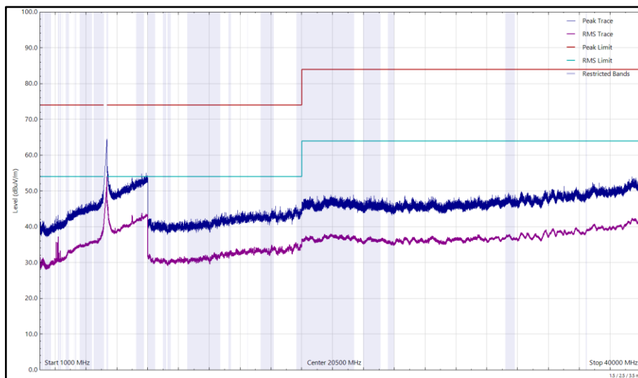
Figure 307 - U-NII-1 - 5180 MHz (CH36), VHT20, CDD, Core 0 + Core 1, 1 GHz to 40 GHz, Horizontal
