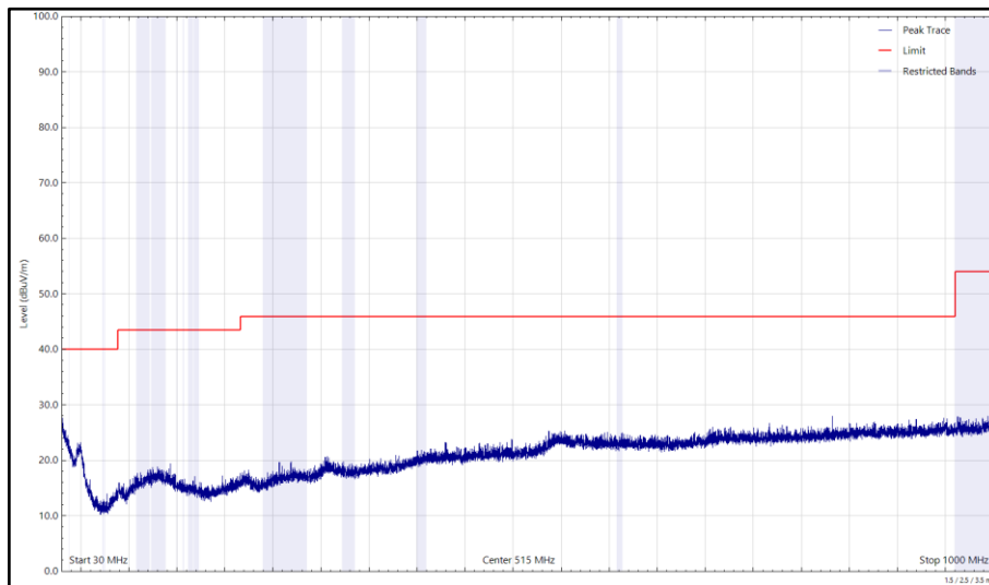
Figure 276 - U-NII-1 - 5180 MHz (CH36), 802.11a, Core 0, 30 MHz to 1 GHz, Vertical (Peak)
