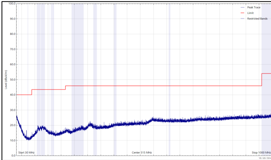
Figure 290 - U-NII-1 - 5180 MHz (CH36), 802.11a, Core 1, 30 MHz to 1 GHz, Horizontal (Peak)
