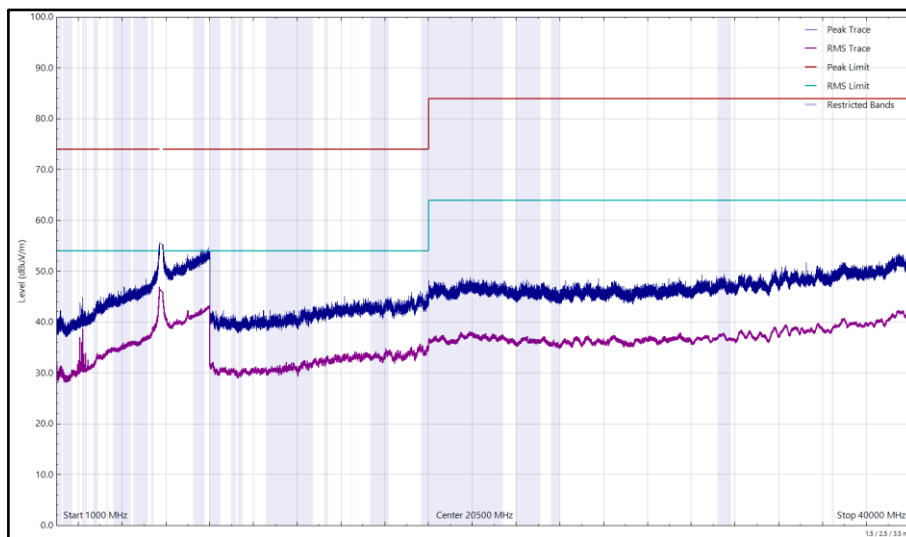
Figure 317 - U-NII-3 - 5745 MHz (CH149), VHT20, CDD, Core 0 + Core 1, 1 GHz to 40 GHz, Vertical
