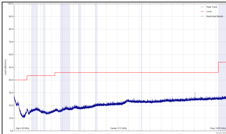
Figure 308 - U-NII-1 - 5180 MHz (CH36), VHT20, CDD, Core 0 + Core 1, 30 MHz to 1 GHz, Vertical (Peak)
