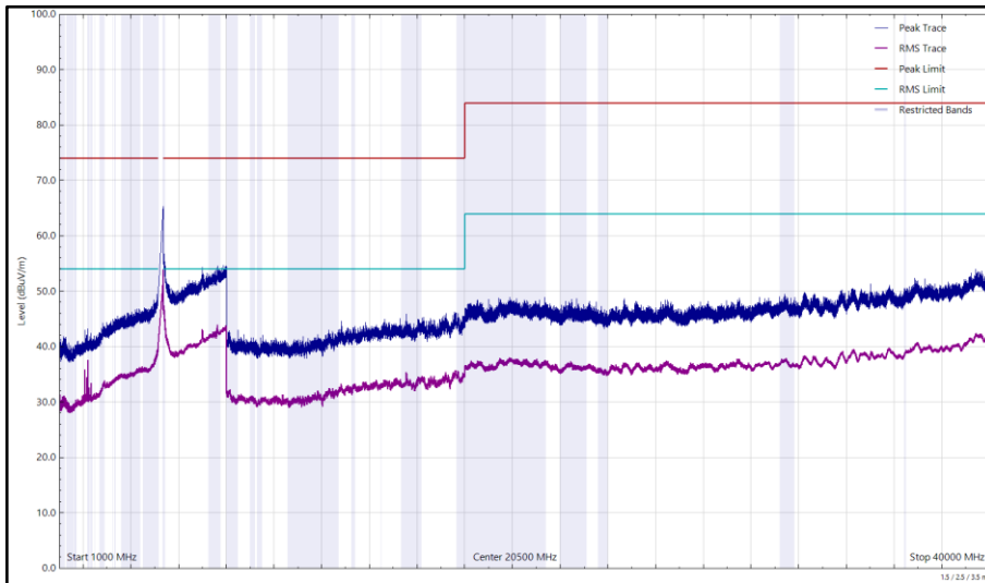
Figure 291 - U-NII-1 - 5180 MHz (CH36), 802.11a, Core 1, 1 GHz to 40 GHz, Horizontal
