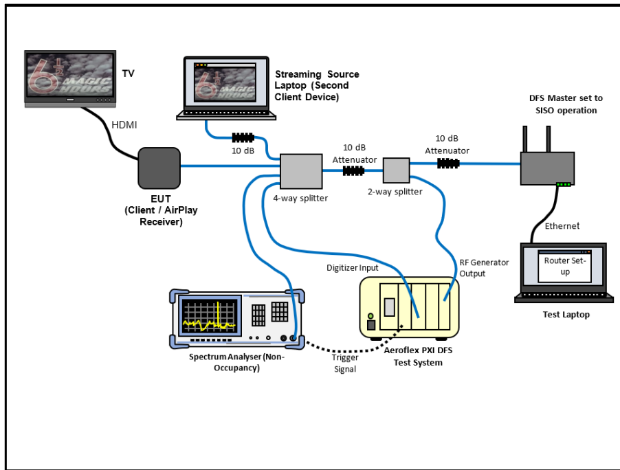
Figure 344 - Test Equipment Setup Diagram for Client without Radar Detection with Injection at the Master
