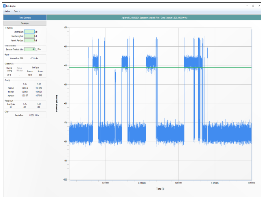
Figure 346 - Channel Loading
