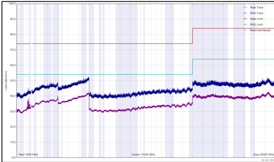
Figure 185 - 2480 MHz (CH39), LE1M, iPA, Core 1, 1 GHz to 26 GHz, Vertical
