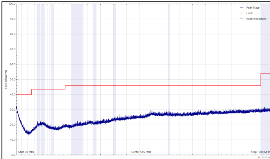
Figure 164 - 2440 MHz (CH17), LE1M, iPA, Core 0, 30 MHz to 1 GHz, Horizontal (Peak)
