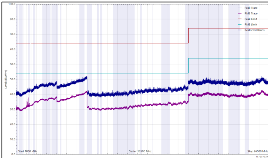
Figure 165 - 2440 MHz (CH17), LE1M, iPA, Core 0, 1 GHz to 26 GHz, Horizontal
