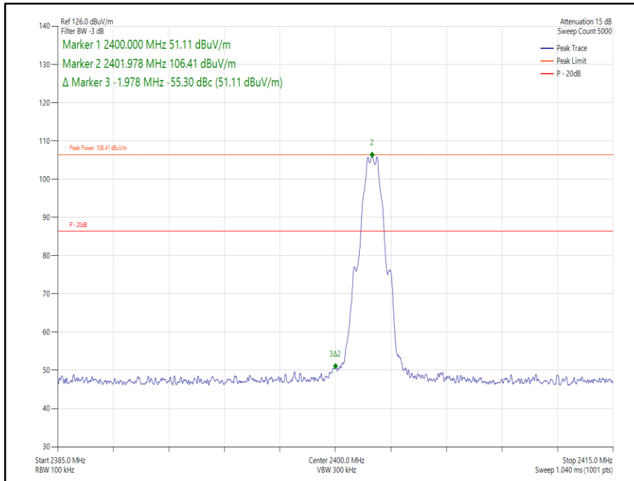
Figure 203 Core 1- GFSK/DH1- Core 1 - 2402 MHz – Band Edge Frequency 2400.0 MHz
