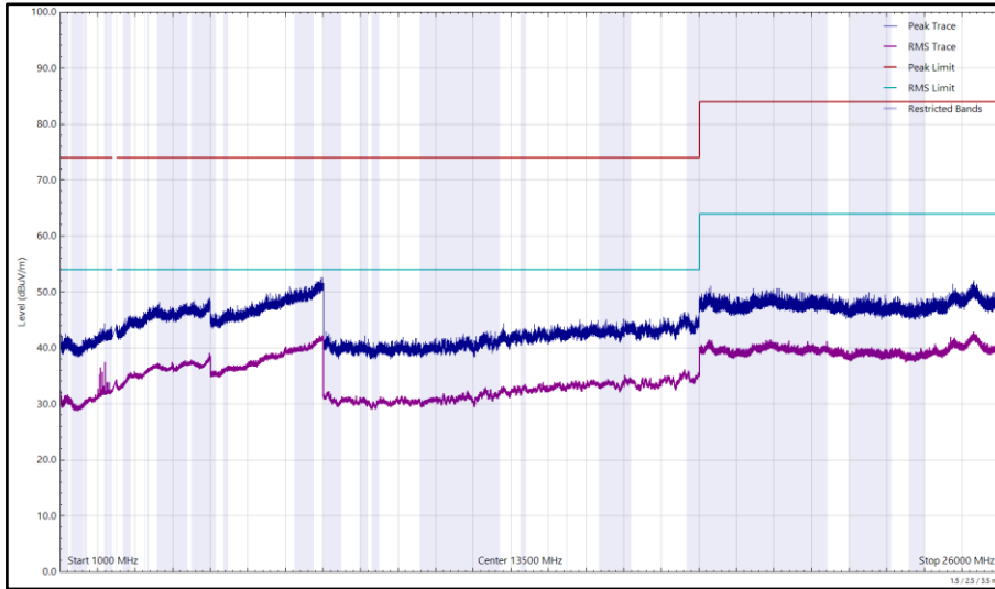
Figure 184 - 2480 MHz (CH39), LE1M, iPA, Core 1, 1 GHz to 26 GHz, Horizontal
