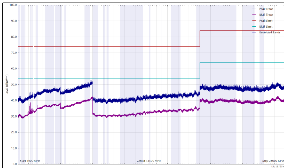
Figure 179 - 2404 MHz (CH0), LE1M, iPA, Core 1, 1 GHz to 26 GHz, Vertical
