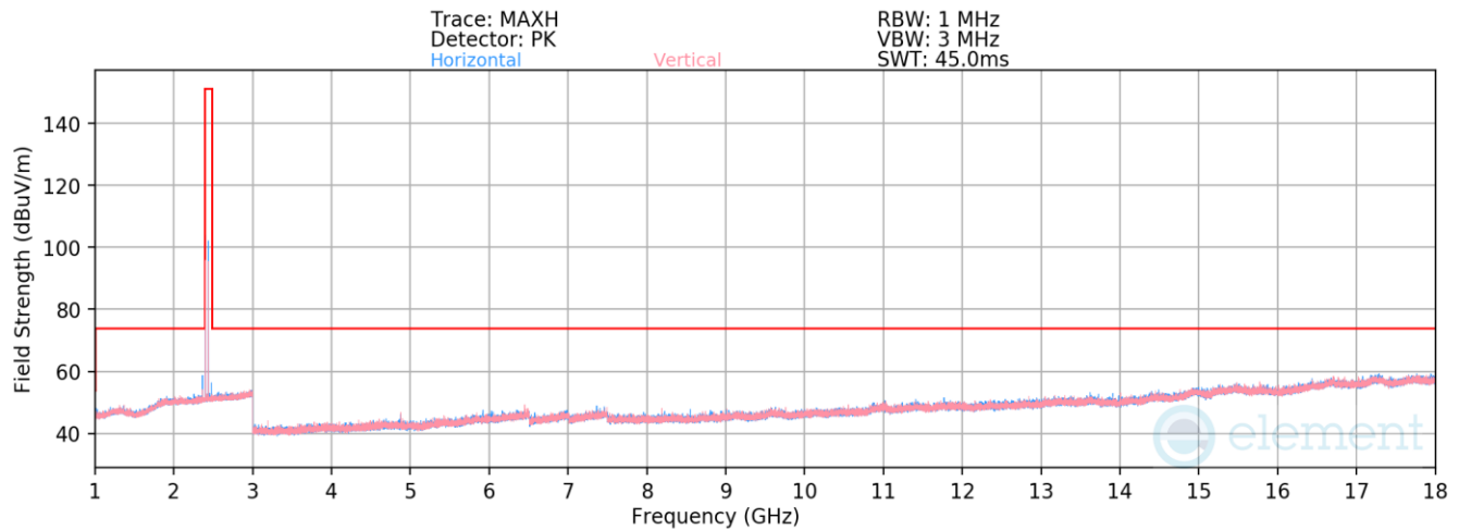
Plot 7-31. Radiated Spurious Emission – Co-Tx 1-18GHz (1Mbps – Ch. 19)
