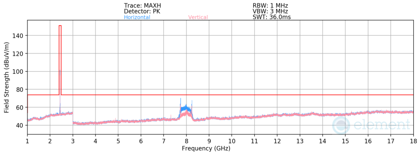
Plot 7-28. Radiated Spurious Simultaneous Transmission 1-18GHz (1Mbps – Ch. 19)
