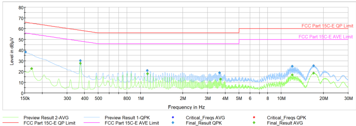
Plot 7-42. AC Line Conducted Plot with Bluetooth LE (N, 1Mbps – Ch.19, with Laptop and AC/DC Adapter)
