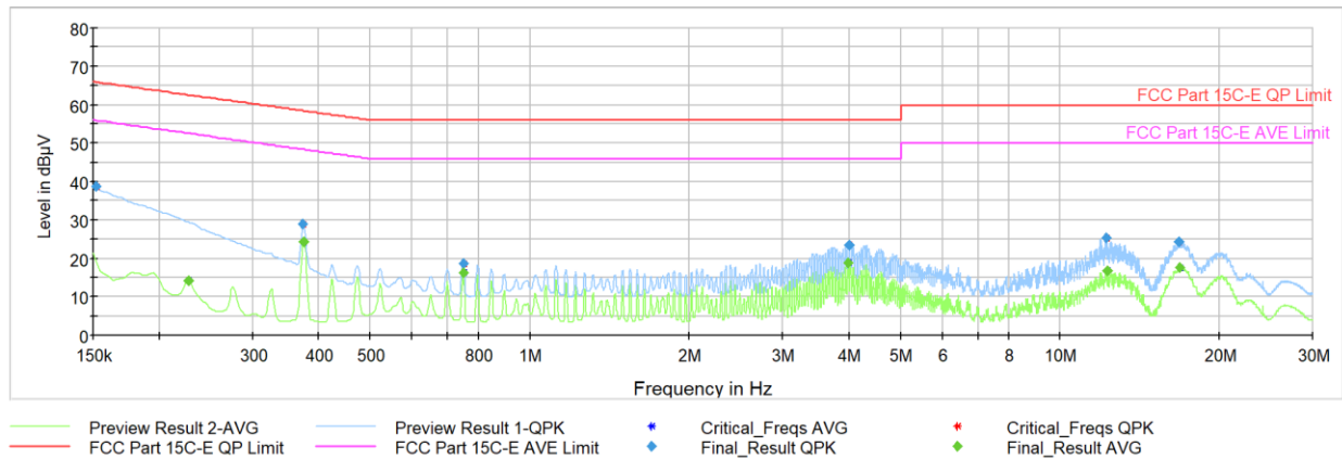
Plot 7-41. AC Line Conducted Plot with Bluetooth LE (L1, 1Mbps – Ch.19 with AC/DC Adapter)
