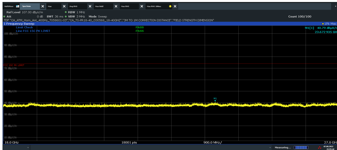
Plot 7-33. Radiated Spurious Emissions – Co-Tx Above 18GHz H Polarity (1Mbps – Ch. 19)
