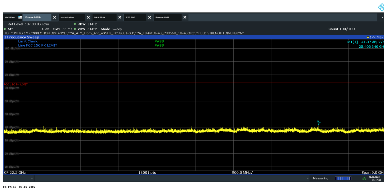
Plot 7-27. Radiated Spurious Emissions Above 18GHz H Polarity (1Mbps – Ch. 19)
