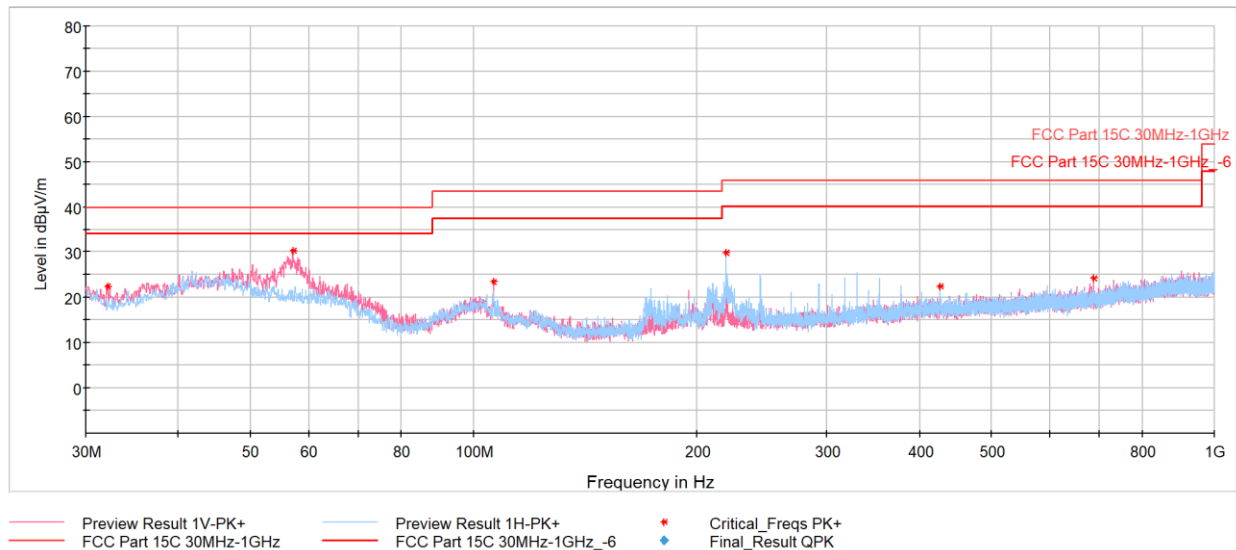
Plot 7-38. Radiated Spurious Emissions Below 1GHz (1Mbps – Ch.19, Pol. H & V, with AC/DC Adapter)
