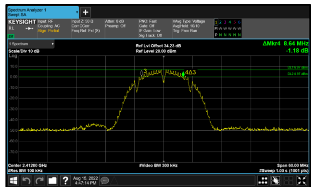
Figure 34 - 802.11b Maximum 6 dB EBW
