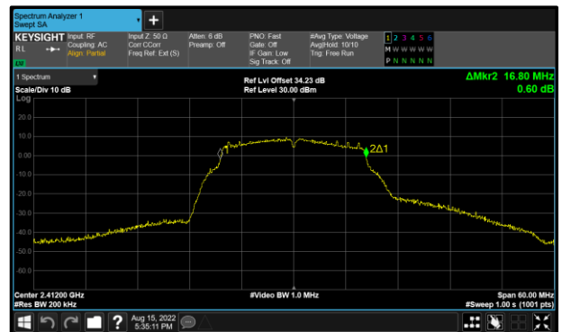
Figure 44 - 802.11g Maximum 99% OBW
