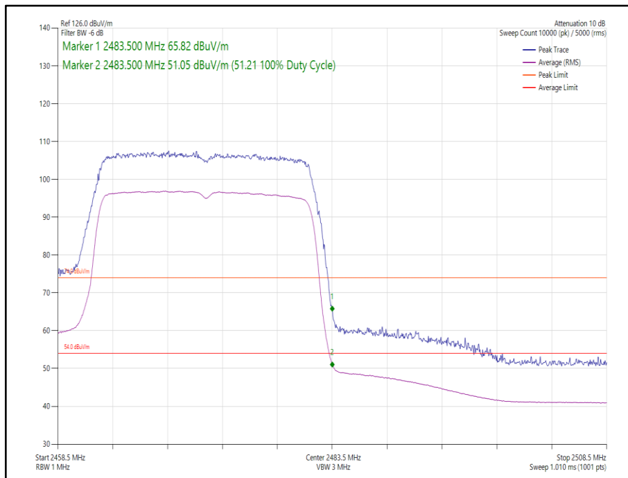
Figure 19 - 802.11ax HE20, Core 1, SU - 2472 MHz, Band Edge Frequency 2483.5 MHz
