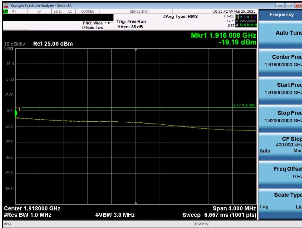
Plot 7-57. Extended Upper Band Edge Plot (LTE Band 25 - 15MHz QPSK – Full RB Configuration)
