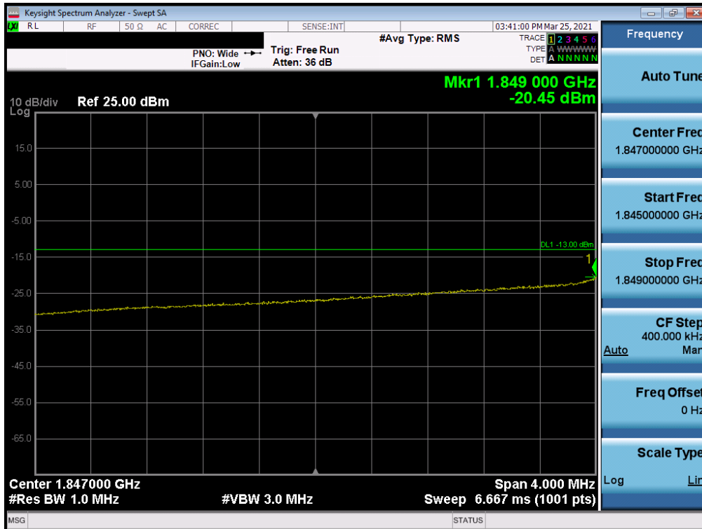
Plot 7-75. Extended Lower Band Edge Plot (LTE Band 2- 10MHz QPSK – Full RB Configuration)
