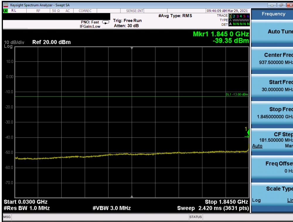
Plot 7-29. CSE (WCDMA Ch. 9262)
