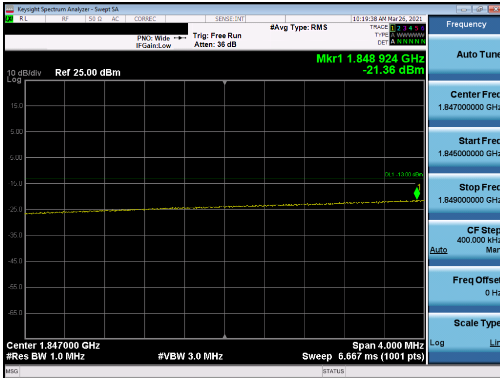
Plot 7-59. Extended Lower Band Edge Plot (LTE Band 25 - 20MHz QPSK – Full RB Configuration)
