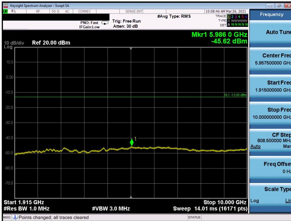
Plot 7-21. CSE (LTE Band 25/2 - 20MHz QPSK - RB Size 1, RB Offset 0 - Low Channel)
