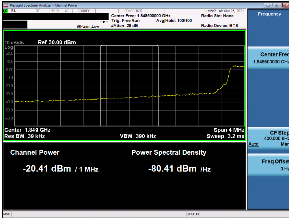
Plot 7-47. Extended Lower Band Edge Plot (LTE Band 25 - 5MHz QPSK – Full RB Configuration)
