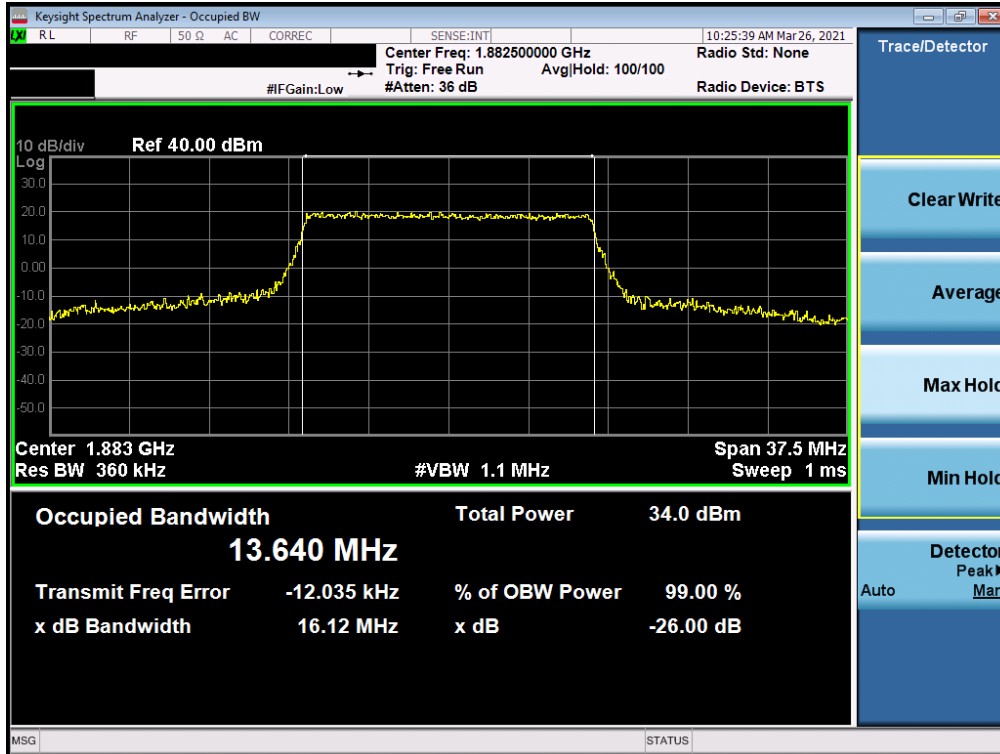
Plot 7-13. Occupied Bandwidth Plot (LTE Band 25/2 - 15MHz QPSK - Full RB Configuration)
