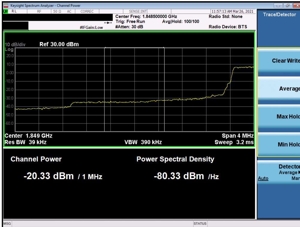
Plot 7-43. Extended Lower Band Edge Plot (LTE Band 25 - 3MHz QPSK – Full RB Configuration)
