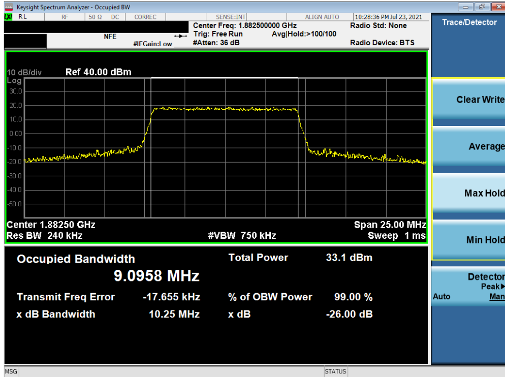
Plot 7-11. Occupied Bandwidth Plot (LTE Band 25/2 - 10MHz 16-QAM - Full RB Configuration)
