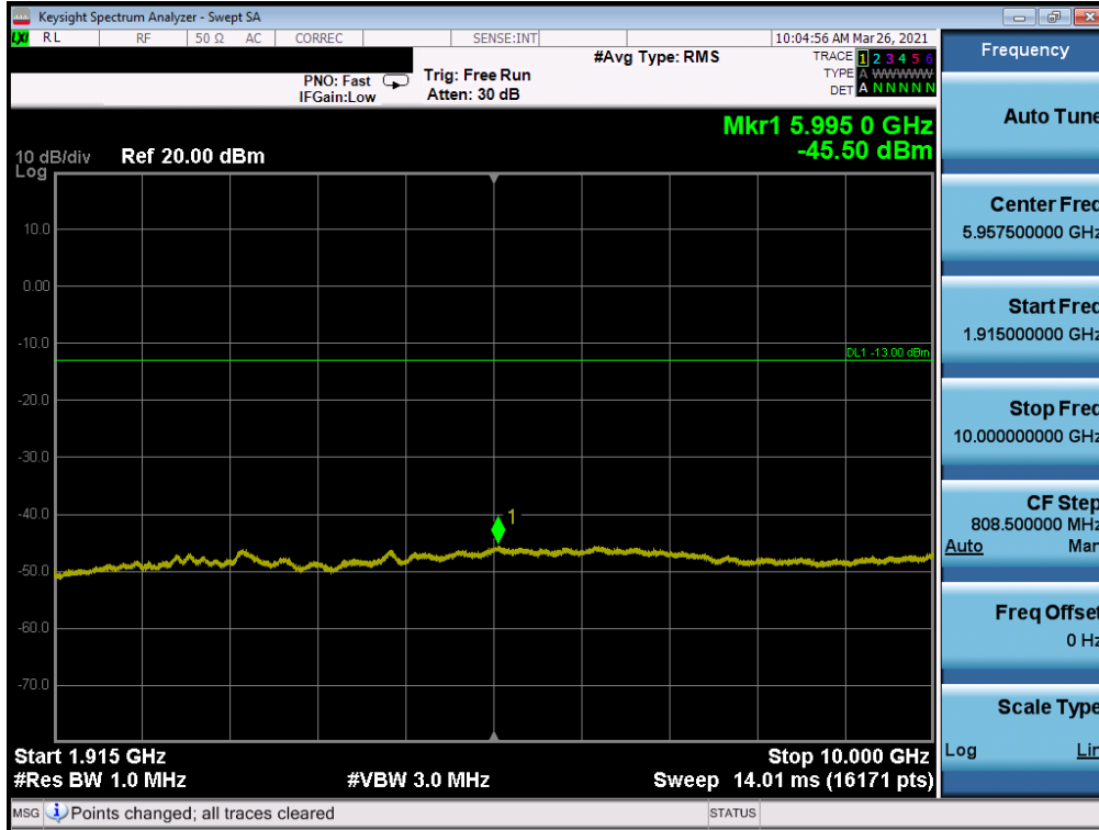
Plot 7-24. CSE (LTE Band 25/2 - 20MHz QPSK - RB Size 1, RB Offset 0 - Mid Channel)
