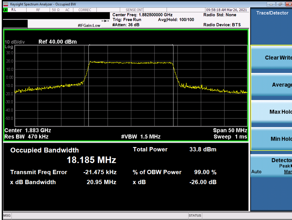
Plot 7-17. Occupied Bandwidth Plot (LTE Band 25/2 - 20MHz 16-QAM - Full RB Configuration)
