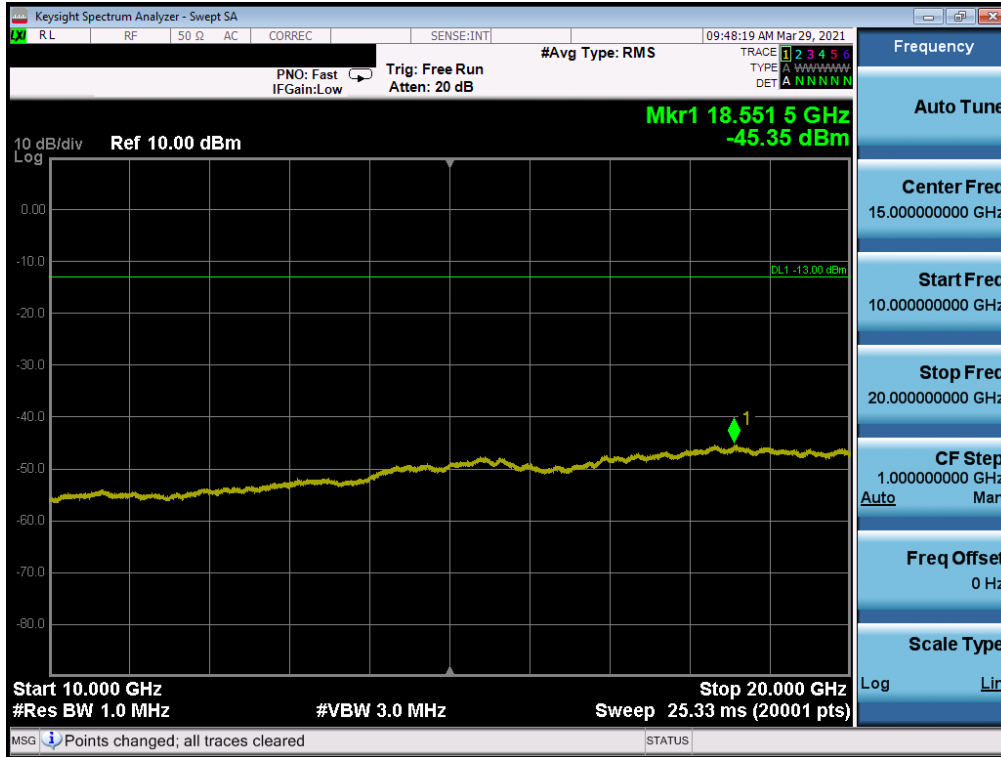
Plot 7-31. CSE (WCDMA Ch. 9262)
