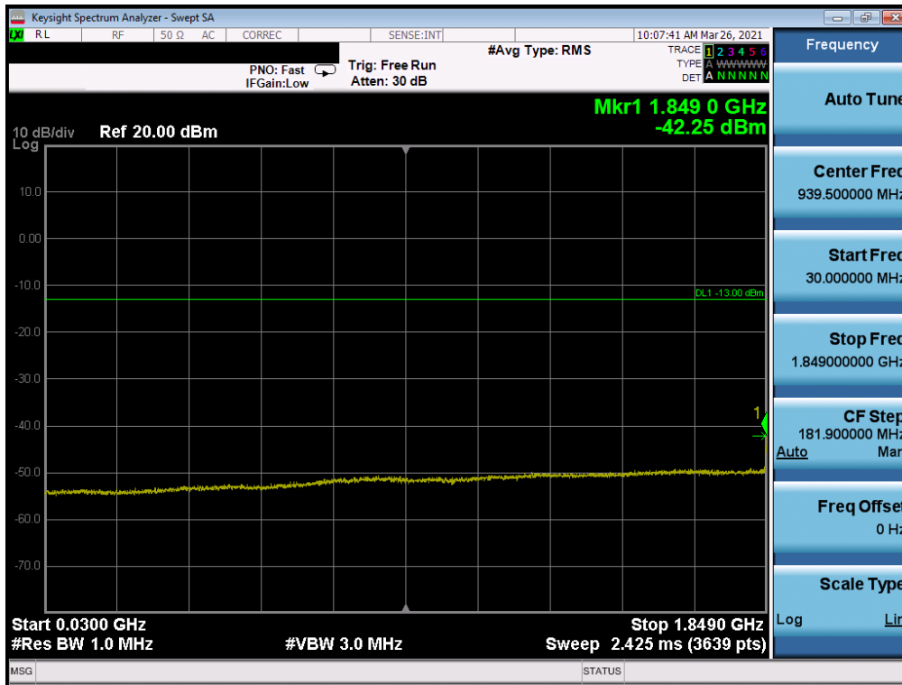
Plot 7-20. CSE (LTE Band 25/2 - 20MHz QPSK - RB Size 1, RB Offset 0 - Low Channel)
