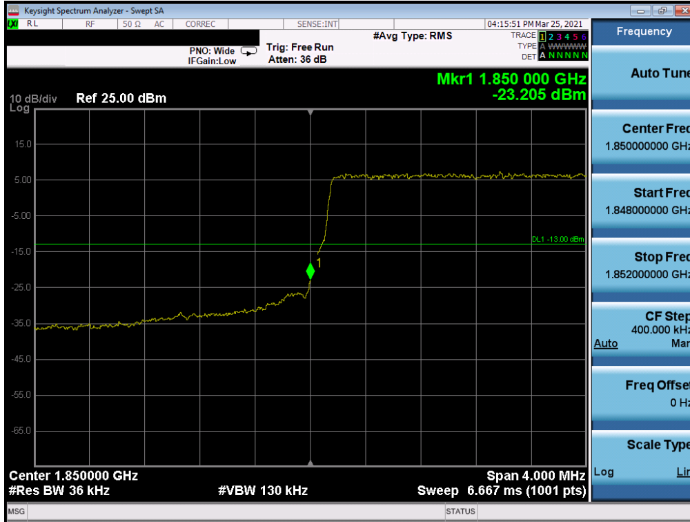
Plot 7-66. Lower Band Edge Plot (LTE Band 2 - 3MHz QPSK – Full RB Configuration)
