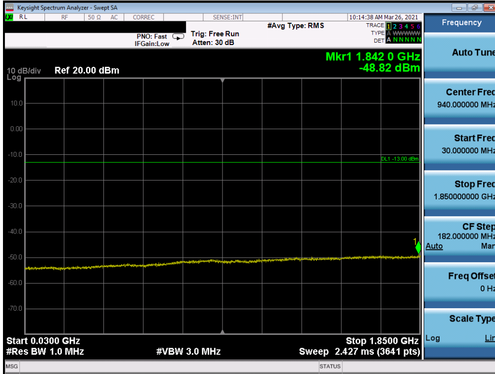
Plot 7-26. CSE (LTE Band 25/2 - 20MHz QPSK - RB Size 1, RB Offset 0 - High Channel)
