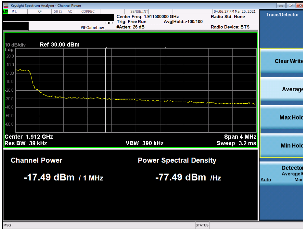
Plot 7-73. Extended Upper Band Edge Plot (LTE Band 2 - 5MHz QPSK – Full RB Configuration)
