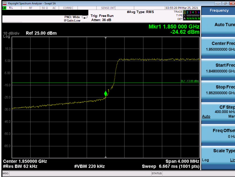
Plot 7-70. Lower Band Edge Plot (LTE Band 2 - 5MHz QPSK – Full RB Configuration)
