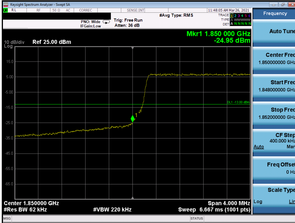
Plot 7-46. Lower Band Edge Plot (LTE Band 25 - 5MHz QPSK – Full RB Configuration)
