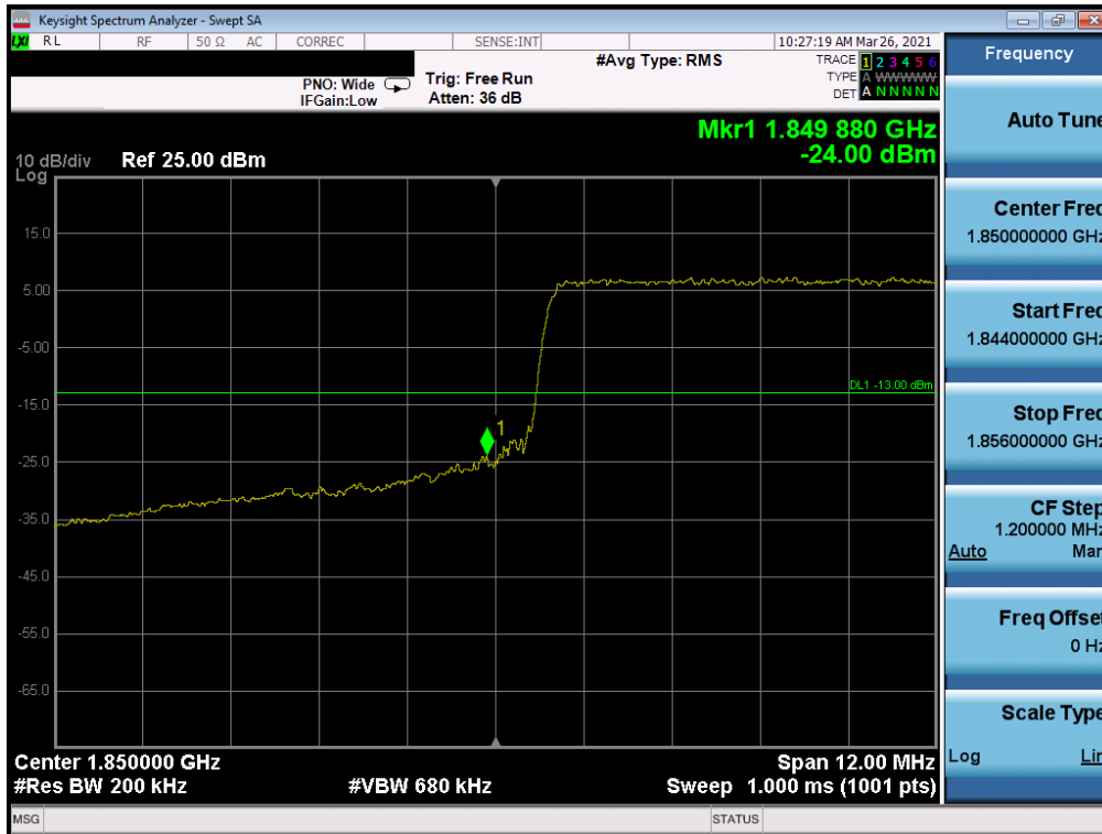
Plot 7-54. Lower Band Edge Plot (LTE Band 25 - 15MHz QPSK – Full RB Configuration)
