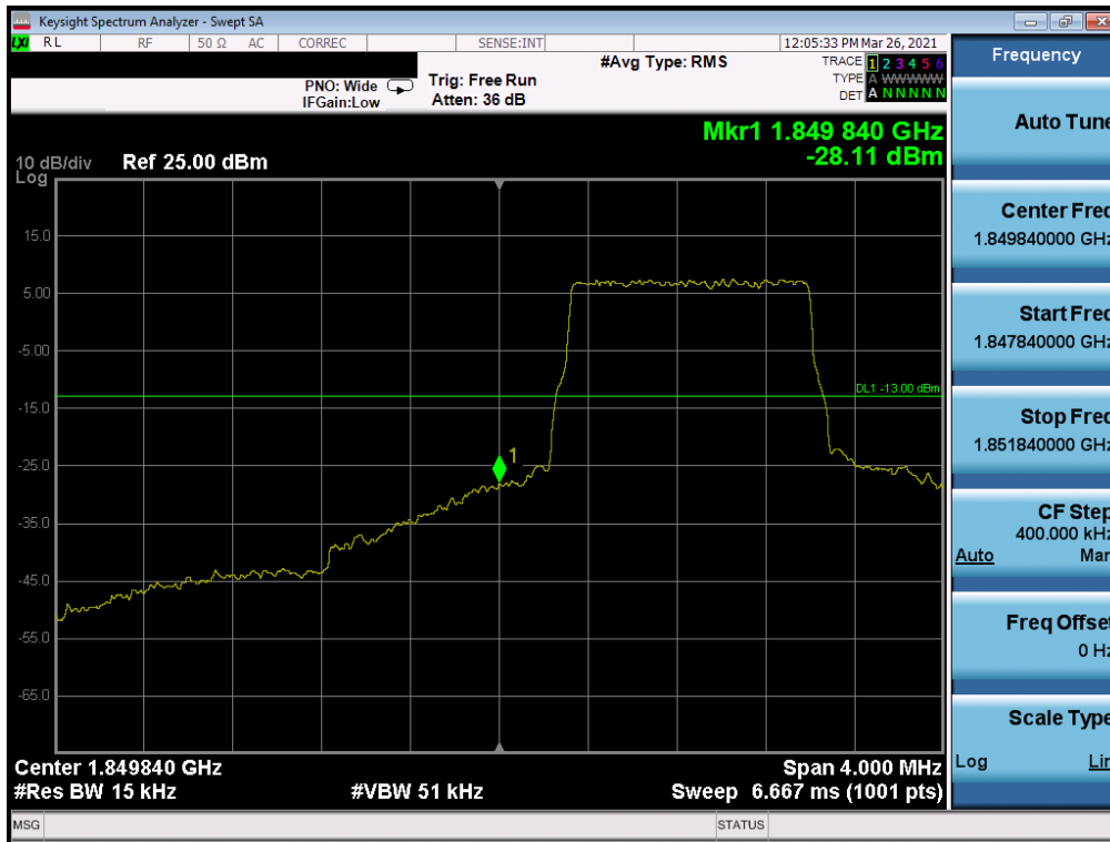
Plot 7-38. Lower Band Edge Plot (LTE Band 25 – 1.4MHz QPSK – Full RB Configuration)
