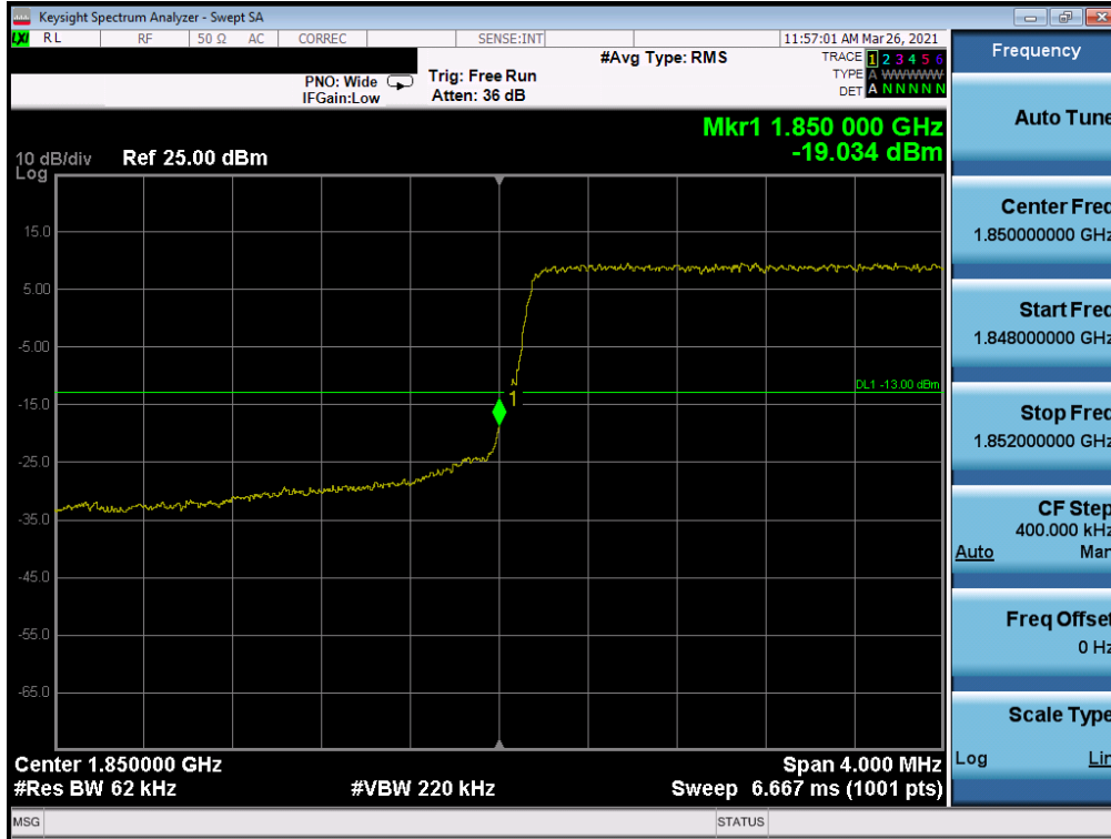
Plot 7-42. Lower Band Edge Plot (LTE Band 25 - 3MHz QPSK – Full RB Configuration)
