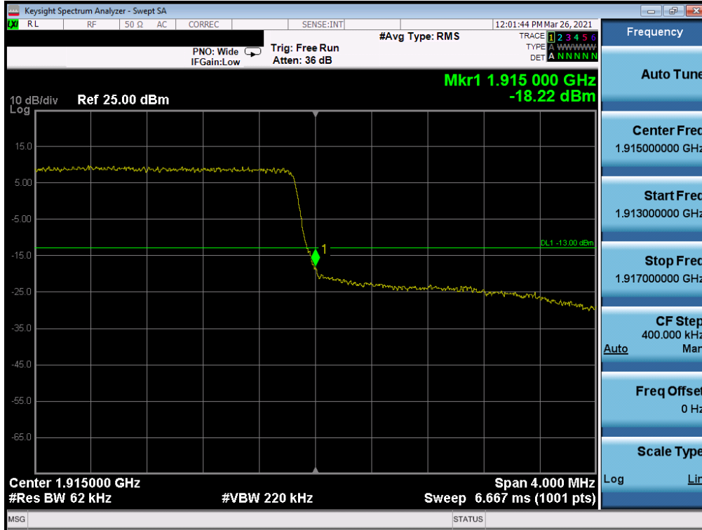
Plot 7-44. Upper Band Edge Plot (LTE Band 25 - 3MHz QPSK – Full RB Configuration)
