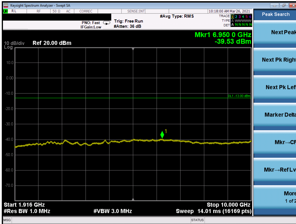
Plot 7-27. CSE (LTE Band 25/2 - 20MHz QPSK - RB Size 1, RB Offset 0 - High Channel)
