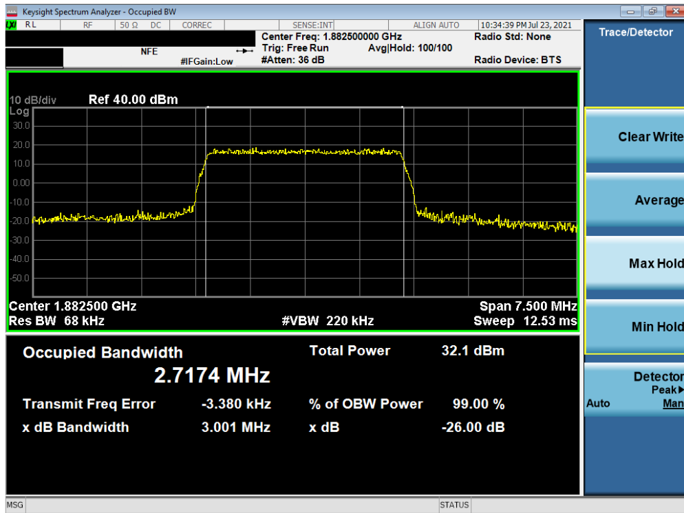
Plot 7-5. Occupied Bandwidth Plot (LTE Band 25/2 - 3MHz 16-QAM - Full RB Configuration)
