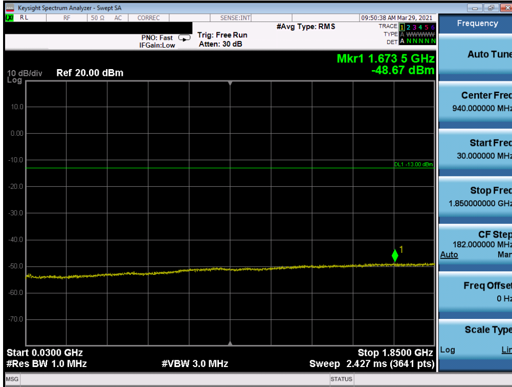
Plot 7-35. CSE (WCDMA Ch. 9538)
