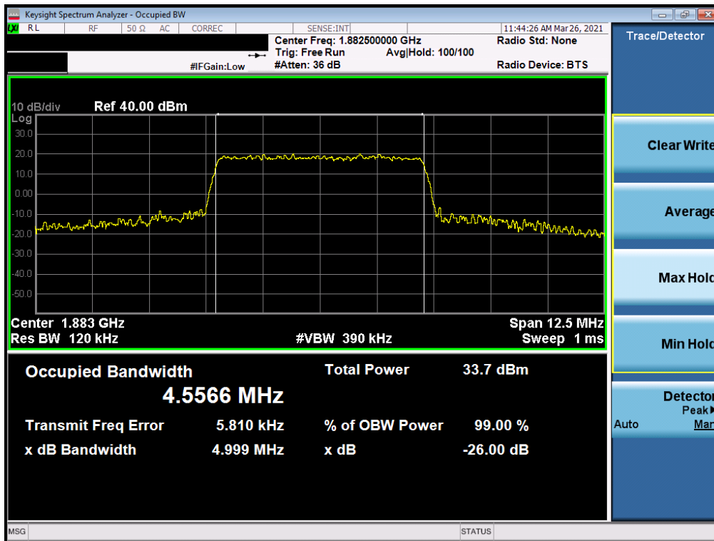
Plot 7-8. Occupied Bandwidth Plot (LTE Band 25/2 - 5MHz 16-QAM - Full RB Configuration)
