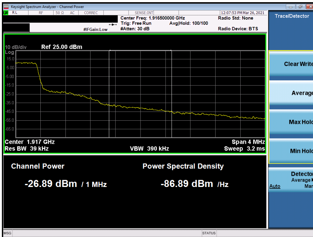
Plot 7-41. Extended Upper Band Edge Plot (LTE Band 25 – 1.4MHz QPSK – Full RB Configuration)
