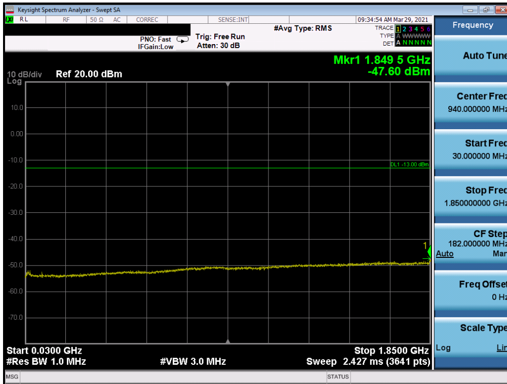
Plot 7-32. CSE (WCDMA Ch. 9400)
