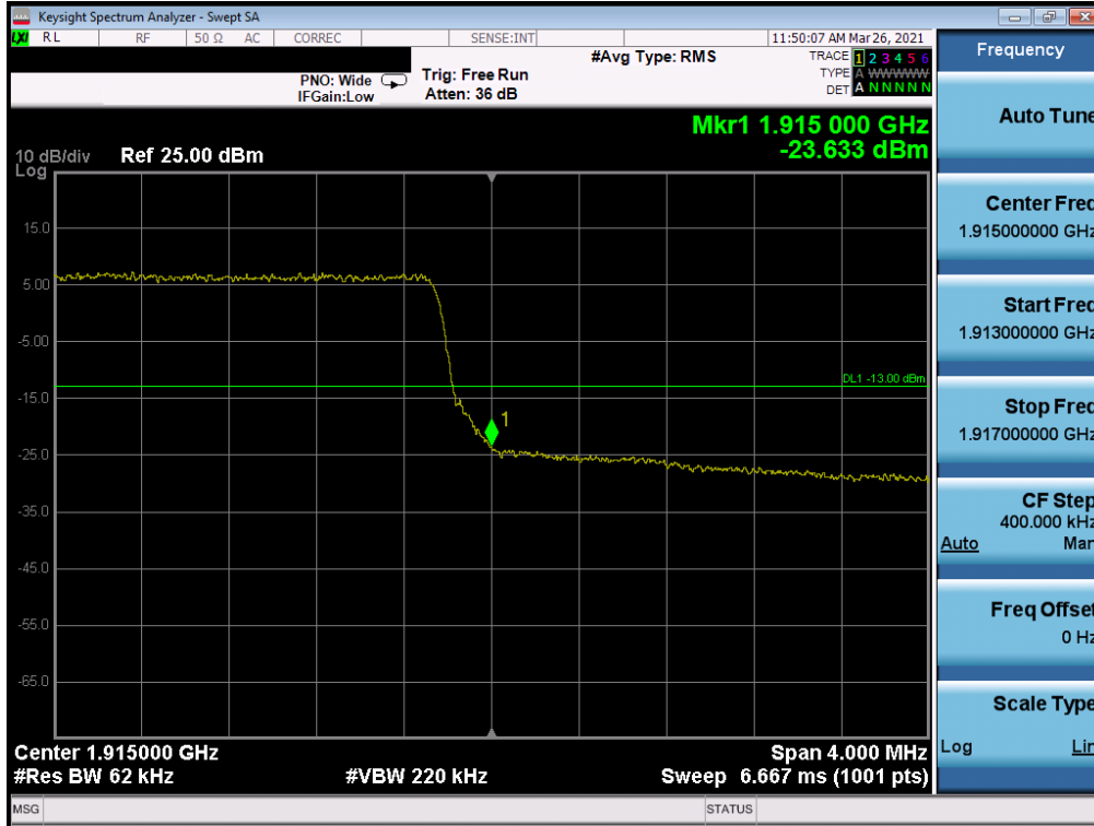
Plot 7-48. Upper Band Edge Plot (LTE Band 25 - 5MHz QPSK – Full RB Configuration)
