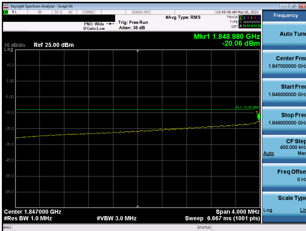
Plot 7-51. Extended Lower Band Edge Plot (LTE Band 25- 10MHz QPSK – Full RB Configuration)
