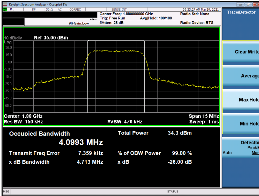
Plot 7-19. Occupied Bandwidth Plot (WCDMA, Ch. 9400)
