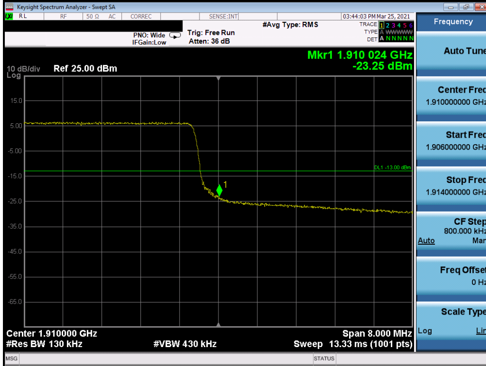
Plot 7-76. Upper Band Edge Plot (LTE Band 2 - 10MHz QPSK – Full RB Configuration)
