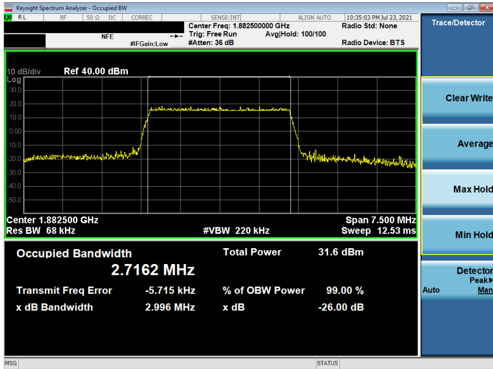
Plot 7-6. Occupied Bandwidth Plot (LTE Band 25/2 - 3MHz 64-QAM - Full RB Configuration)
