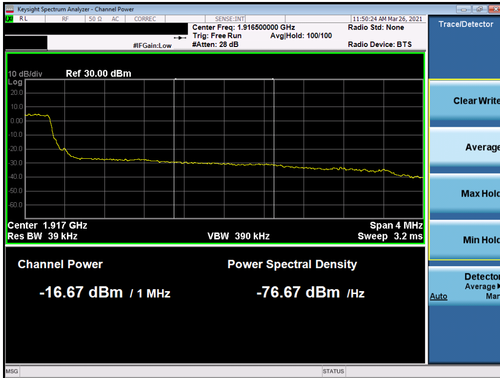
Plot 7-49. Extended Upper Band Edge Plot (LTE Band 25 - 5MHz QPSK – Full RB Configuration)
