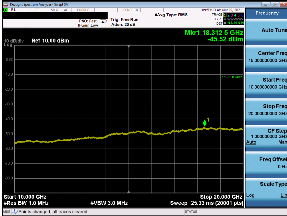
Plot 7-37. CSE (WCDMA Ch. 9538)
