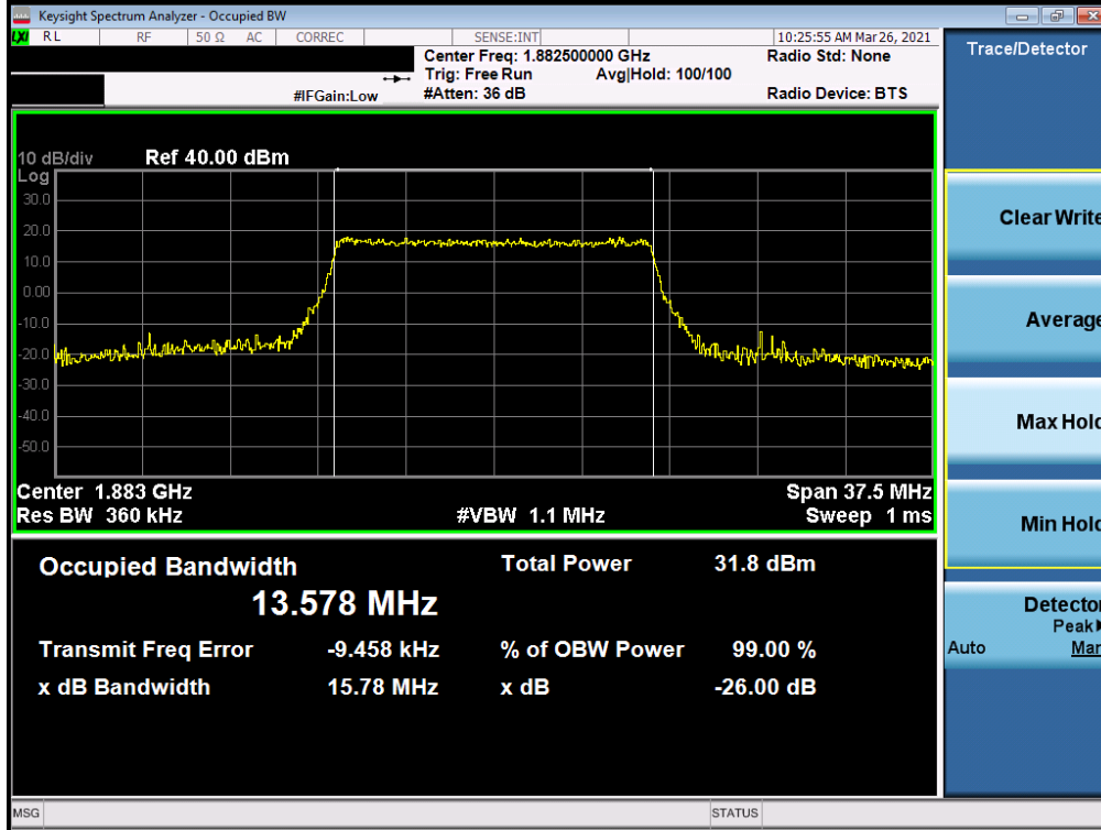
Plot 7-15. Occupied Bandwidth Plot (LTE Band 25/2 - 15MHz 64-QAM - Full RB Configuration)
