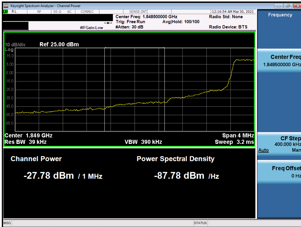
Plot 7-63. Extended Lower Band Edge Plot (LTE Band 2 – 1.4MHz QPSK – Full RB Configuration)
