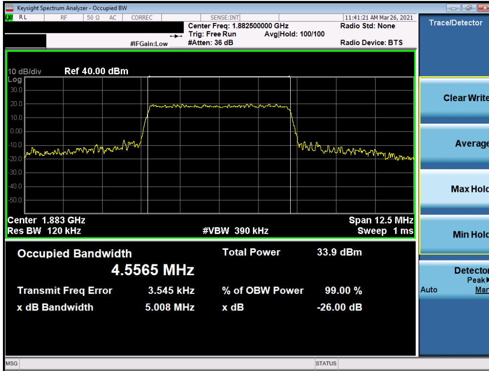
Plot 7-7. Occupied Bandwidth Plot (LTE Band 25/2 - 5MHz QPSK - Full RB Configuration)
