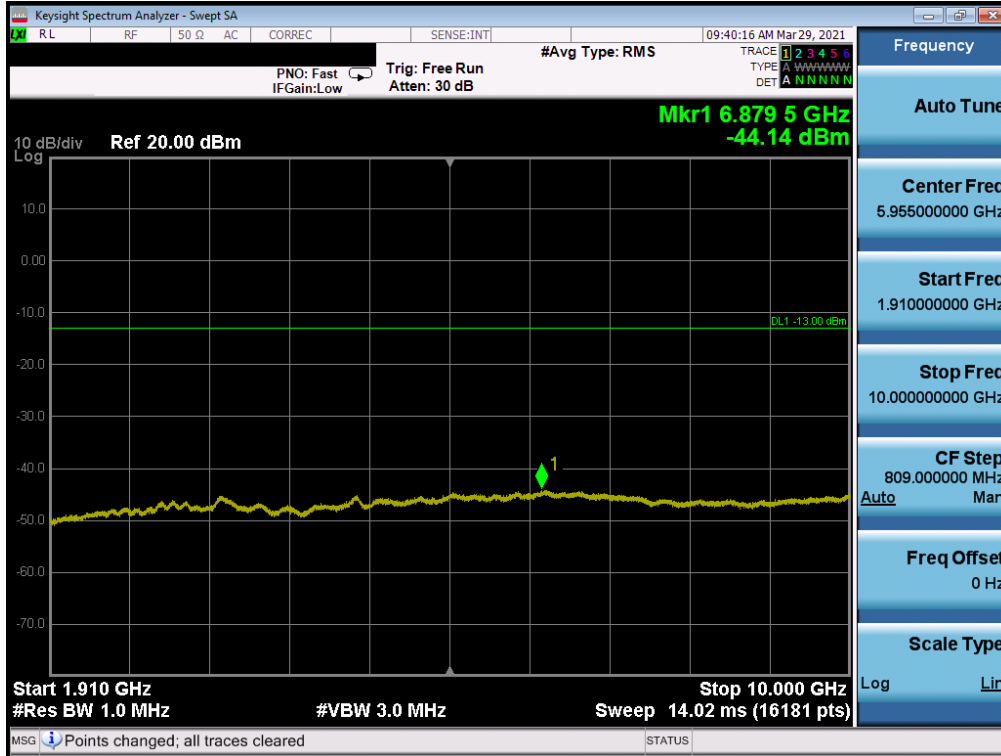
Plot 7-33. CSE (WCDMA Ch. 9400)
