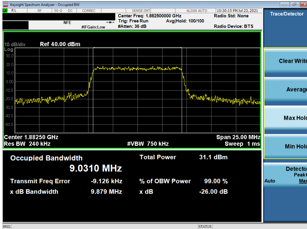
Plot 7-10. Occupied Bandwidth Plot (LTE Band 25/2 - 10MHz QPSK - Full RB Configuration)
