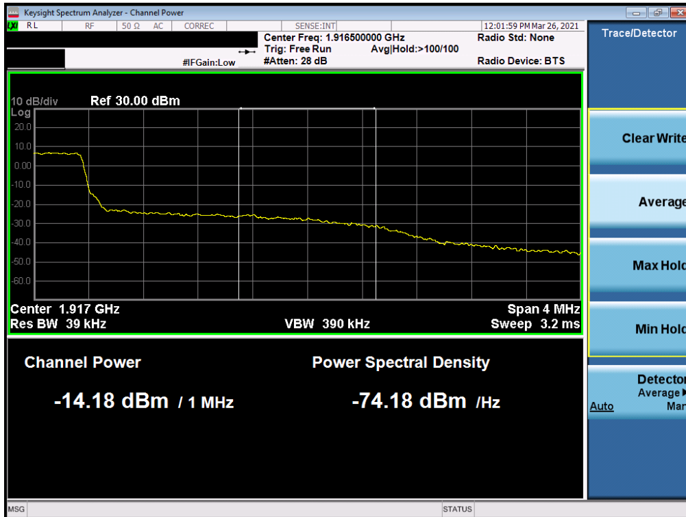
Plot 7-45. Extended Upper Band Edge Plot (LTE Band 25 - 3MHz QPSK – Full RB Configuration)
