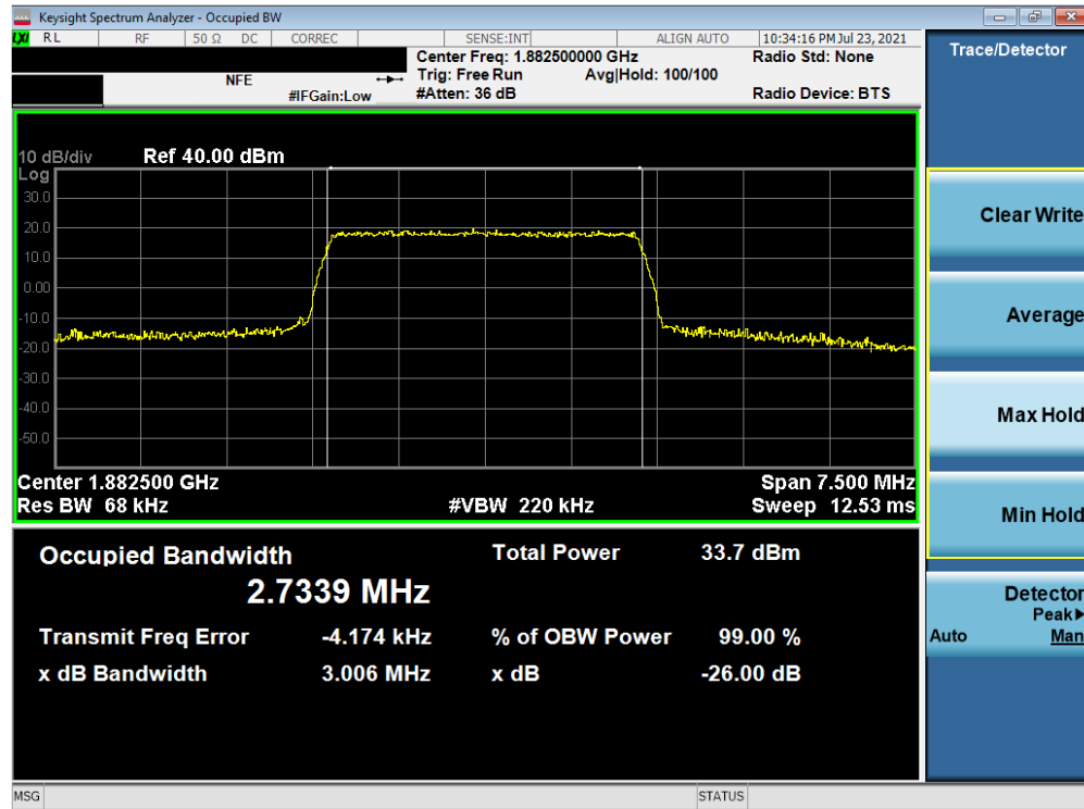
Plot 7-4. Occupied Bandwidth Plot (LTE Band 25/2 - 3MHz QPSK - Full RB Configuration)
