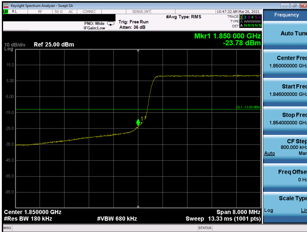
Plot 7-50. Lower Band Edge Plot (LTE Band 25 - 10MHz QPSK – Full RB Configuration)
