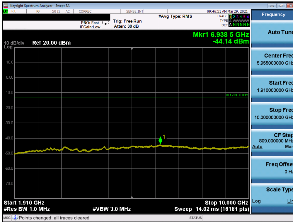
Plot 7-30. CSE (WCDMA Ch. 9262)
