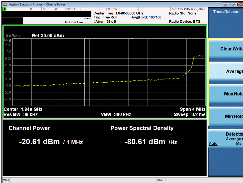
Plot 7-71. Extended Lower Band Edge Plot (LTE Band 2 - 5MHz QPSK – Full RB Configuration)
