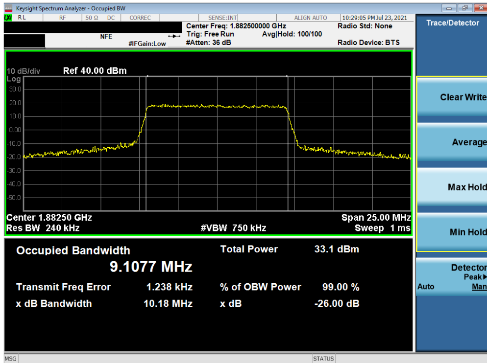
Plot 7-12. Occupied Bandwidth Plot (LTE Band 25/2 - 10MHz 64-QAM - Full RB Configuration)
