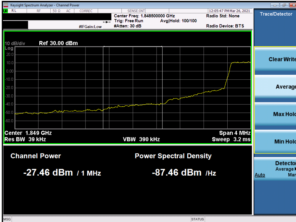
Plot 7-39. Extended Lower Band Edge Plot (LTE Band 25 – 1.4MHz QPSK – Full RB Configuration)
