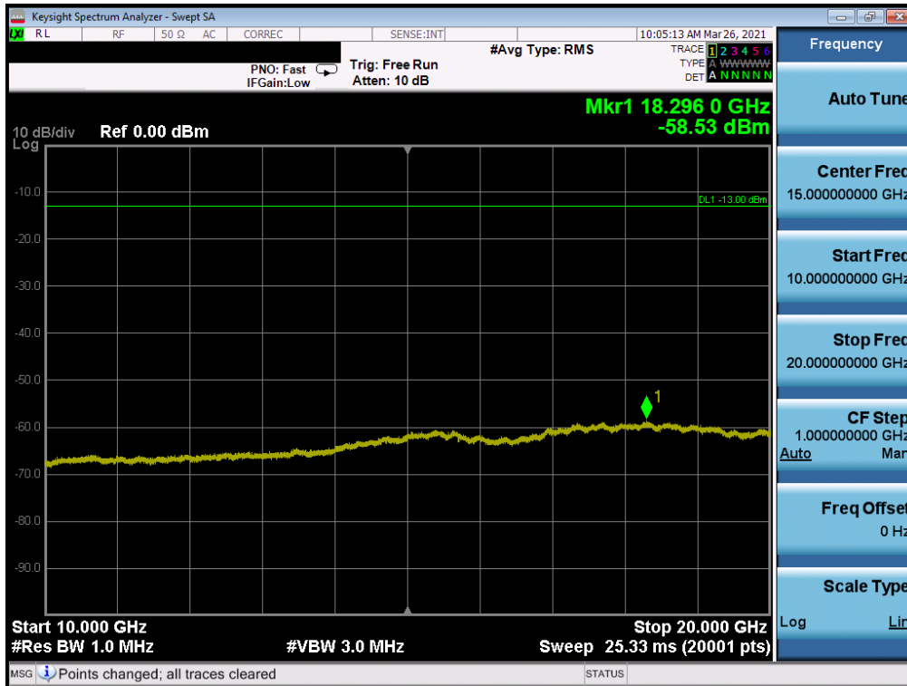
Plot 7-25. CSE (LTE Band 25/2 - 20MHz QPSK - RB Size 1, RB Offset 0 - Mid Channel)
