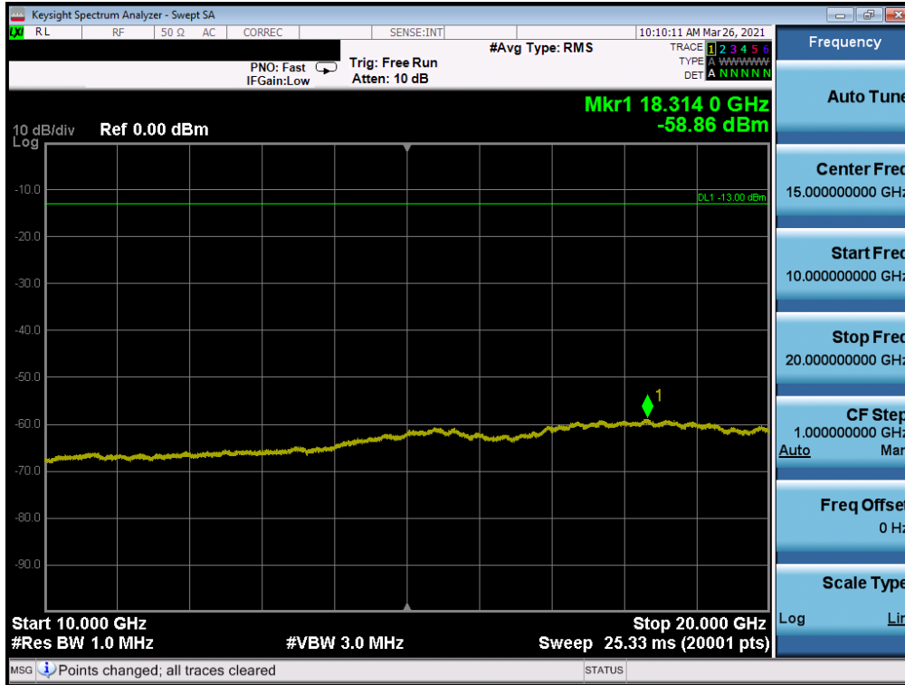
Plot 7-22. CSE (LTE Band 25/2 - 20MHz QPSK - RB Size 1, RB Offset 0 - Low Channel)
