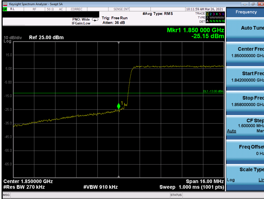
Plot 7-58. Lower Band Edge Plot (LTE Band 25 - 20MHz QPSK – Full RB Configuration)
