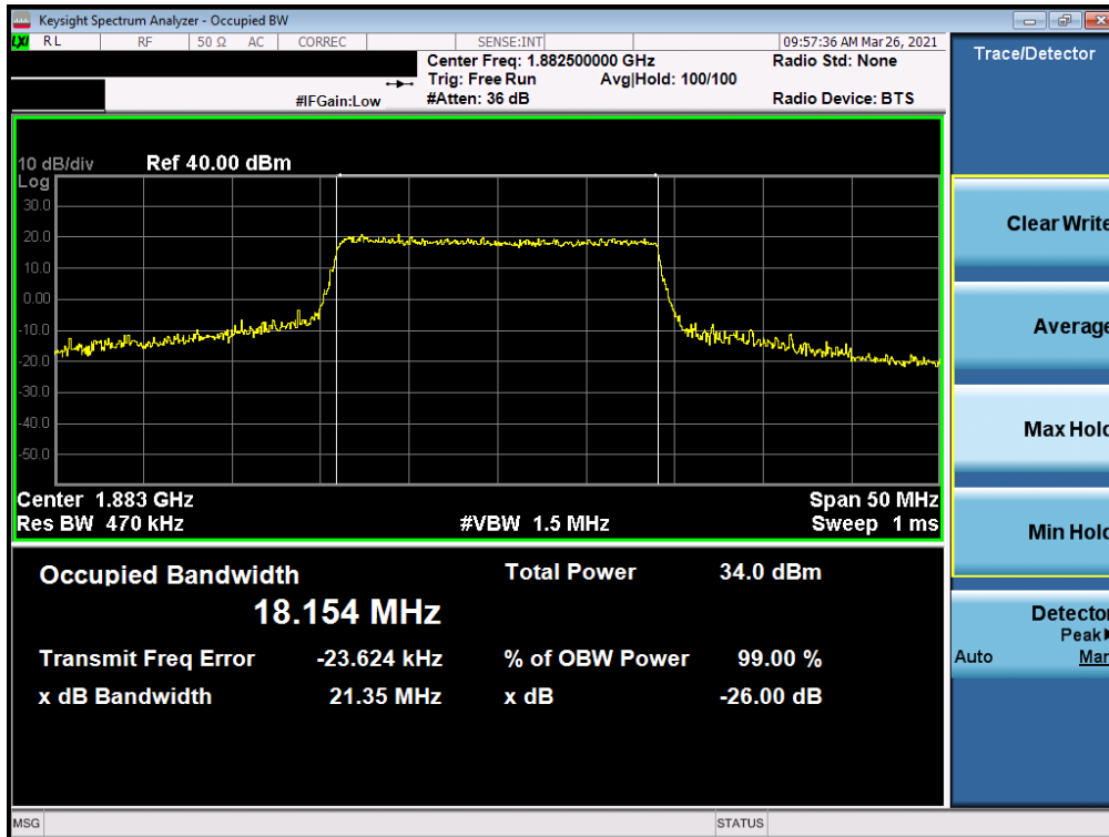
Plot 7-16. Occupied Bandwidth Plot (LTE Band 25/2 - 20MHz QPSK - Full RB Configuration)
