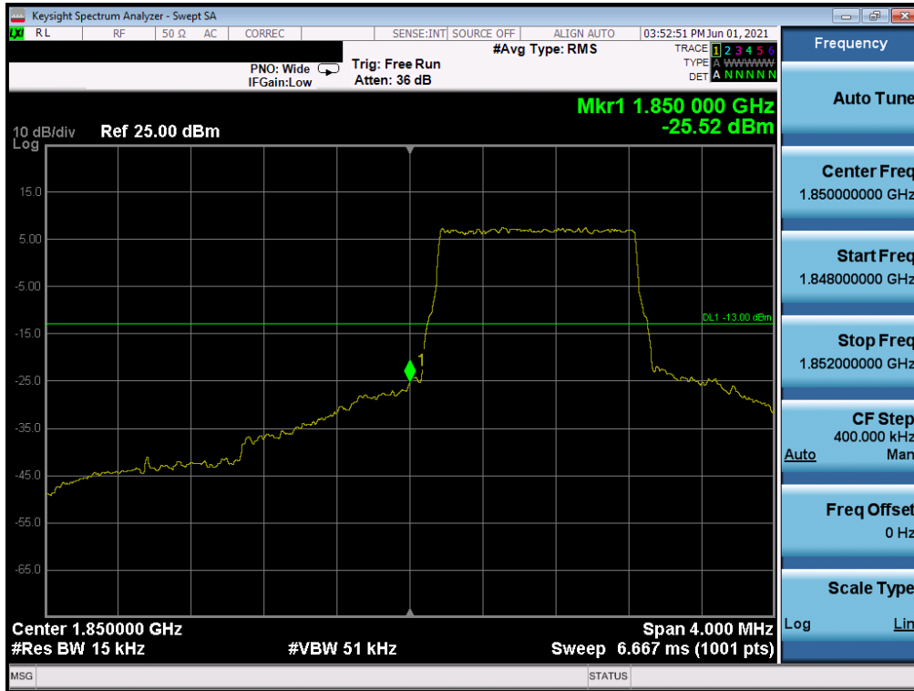
Plot 7-62. Lower Band Edge Plot (LTE Band 2 – 1.4MHz QPSK – Full RB Configuration)
