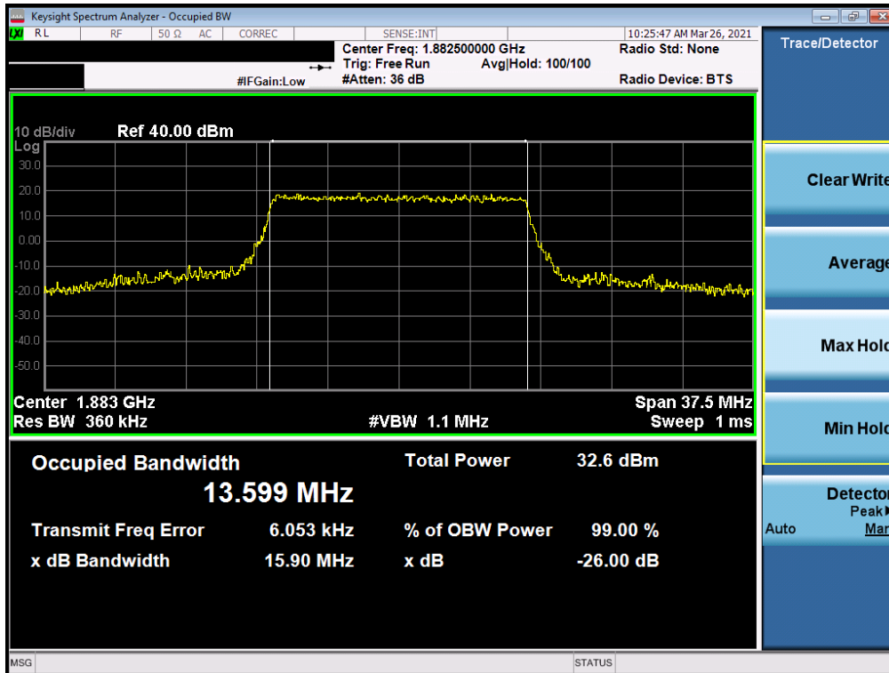
Plot 7-14. Occupied Bandwidth Plot (LTE Band 25/2 - 15MHz 16-QAM - Full RB Configuration)
