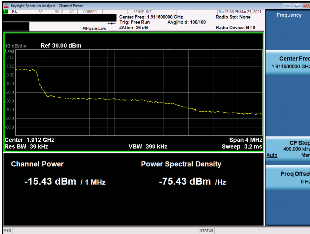
Plot 7-69. Extended Upper Band Edge Plot (LTE Band 2 - 3MHz QPSK – Full RB Configuration)
