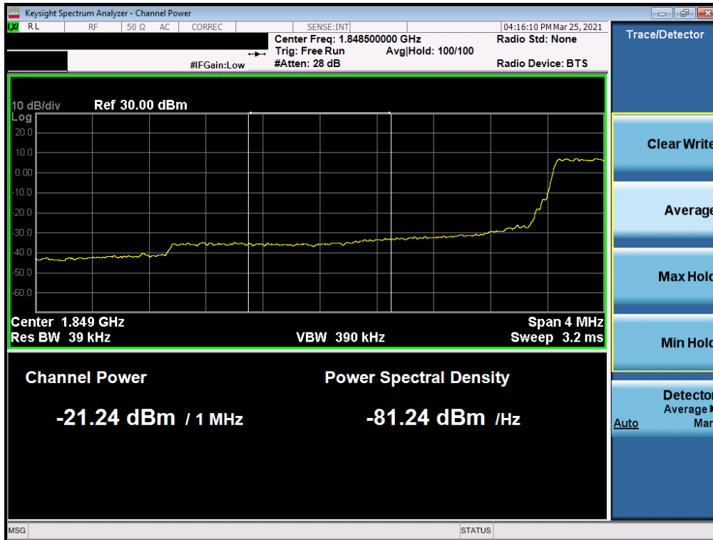
Plot 7-67. Extended Lower Band Edge Plot (LTE Band 2 - 3MHz QPSK – Full RB Configuration)
