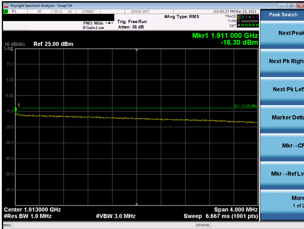
Plot 7-77. Extended Upper Band Edge Plot (LTE Band 2 - 10MHz QPSK – Full RB Configuration)
