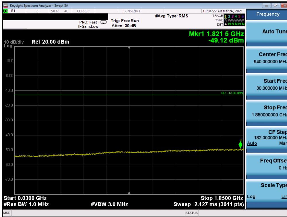
Plot 7-23. CSE (LTE Band 25/2 - 20MHz QPSK - RB Size 1, RB Offset 0 - Mid Channel)
