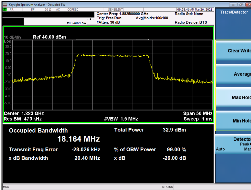
Plot 7-18. Occupied Bandwidth Plot (LTE Band 25/2 - 20MHz 64-QAM - Full RB Configuration)
