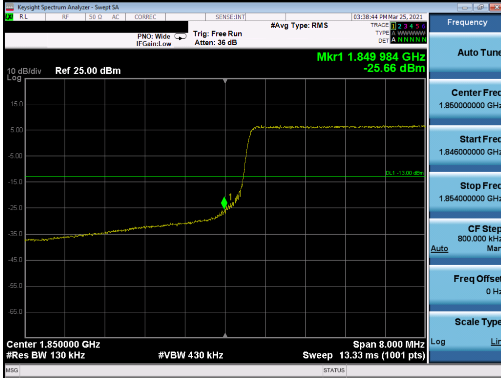
Plot 7-74. Lower Band Edge Plot (LTE Band 2 - 10MHz QPSK – Full RB Configuration)
