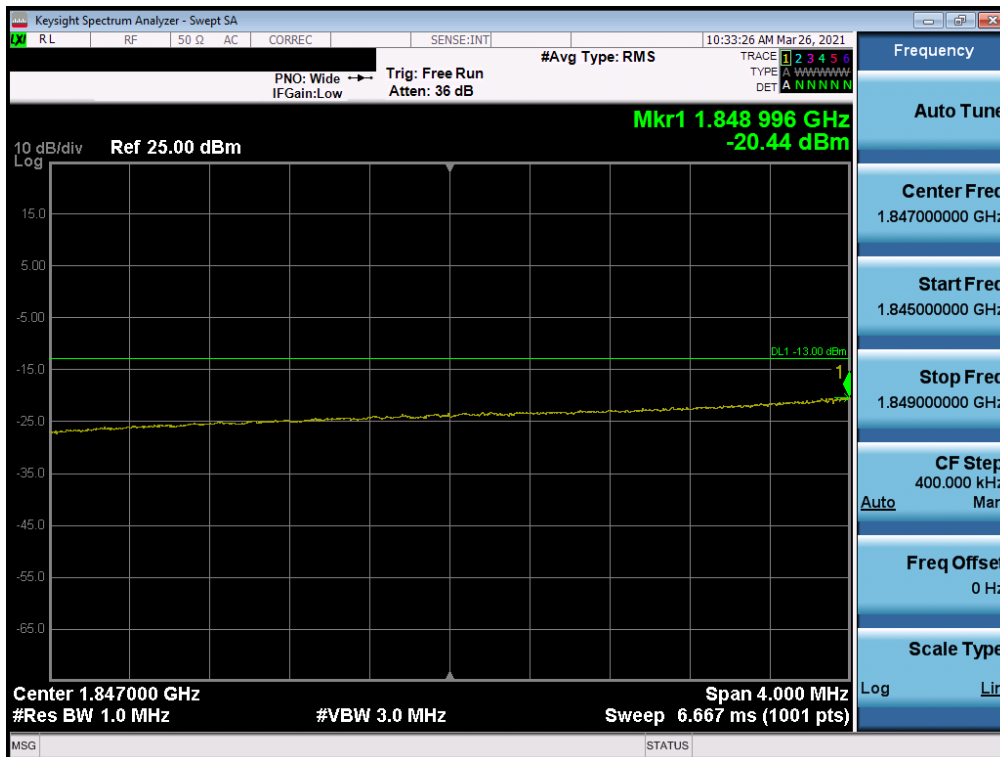
Plot 7-55. Extended Lower Band Edge Plot (LTE Band 25 - 15MHz QPSK – Full RB Configuration)
