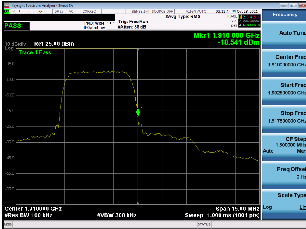
Plot 7-182. Upper Band Edge Plot (WCDMA PCS – Ch. 9538)
