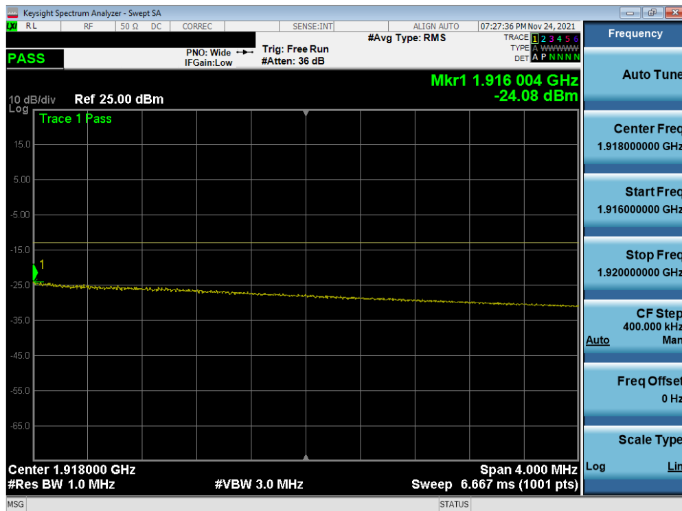
Plot 7-151. Extended Upper Band Edge Plot (NR Band n25 – 20MHz CP-OFDM QPSK – Full RB Configuration)
