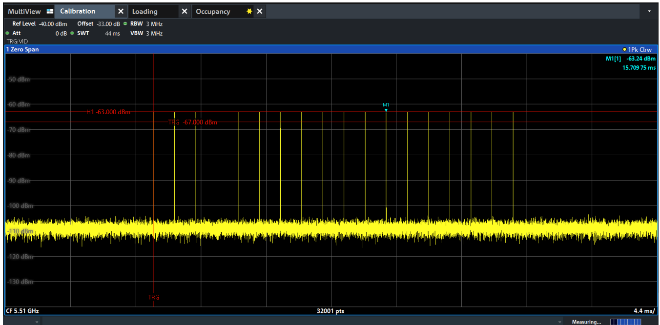
Figure 7-4. 5510MHz – Radar Pulse Type 0 (40MHz)
