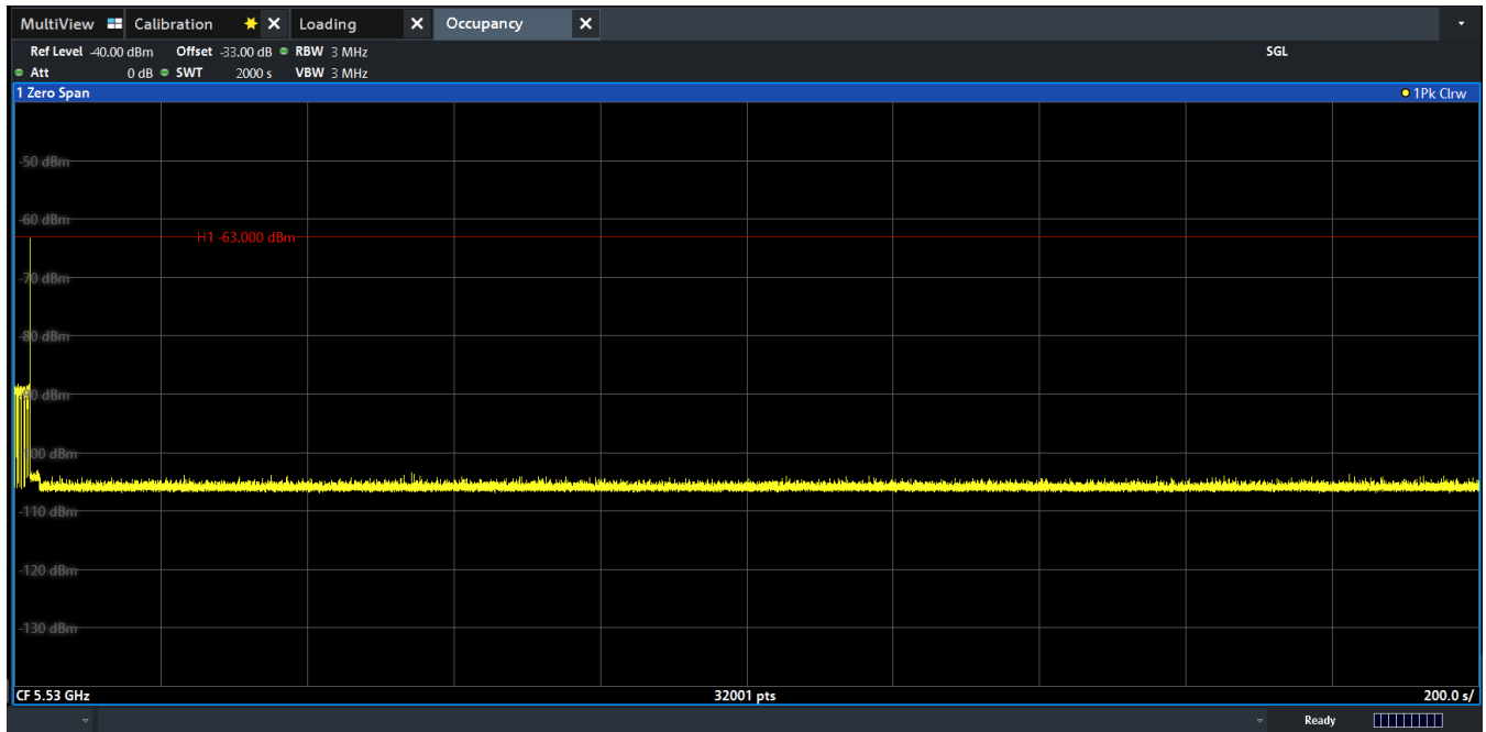
Figure 9-48. 5530MHz - Non-Occupancy Period (30 Minutes) - Mode 4 (80MHz)
