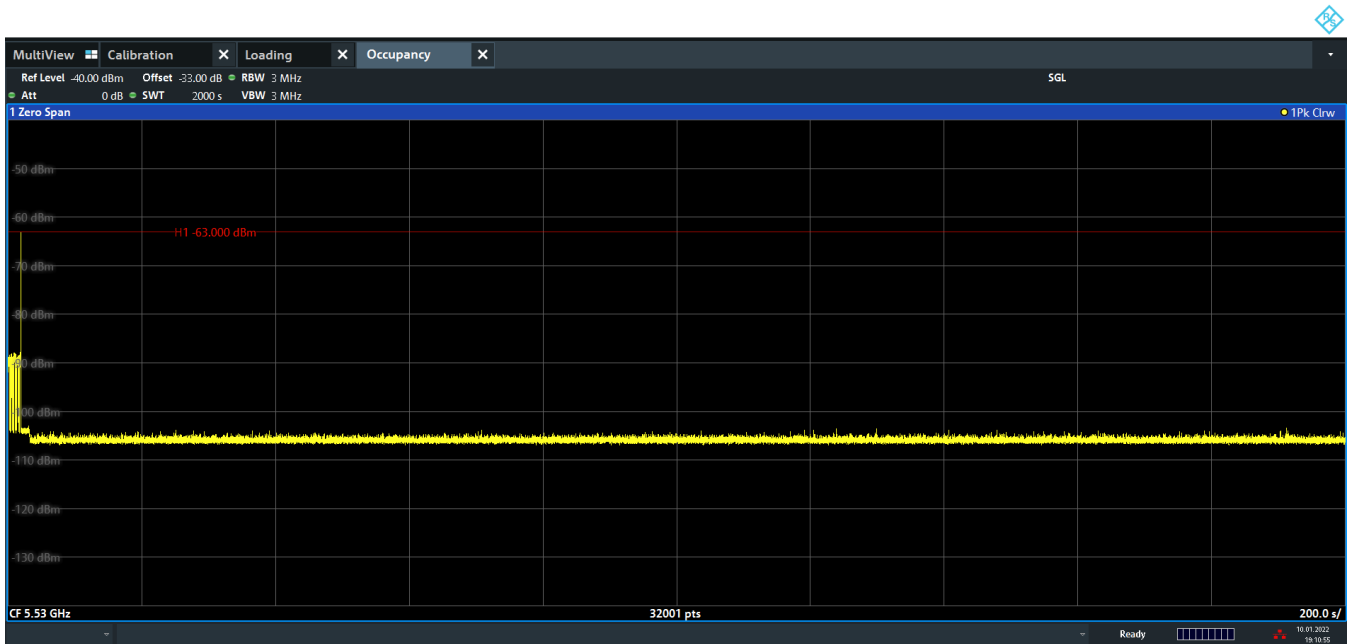
Figure 9-42. 5530MHz - Non-Occupancy Period (30 Minutes) - Mode 2 (80MHz)
