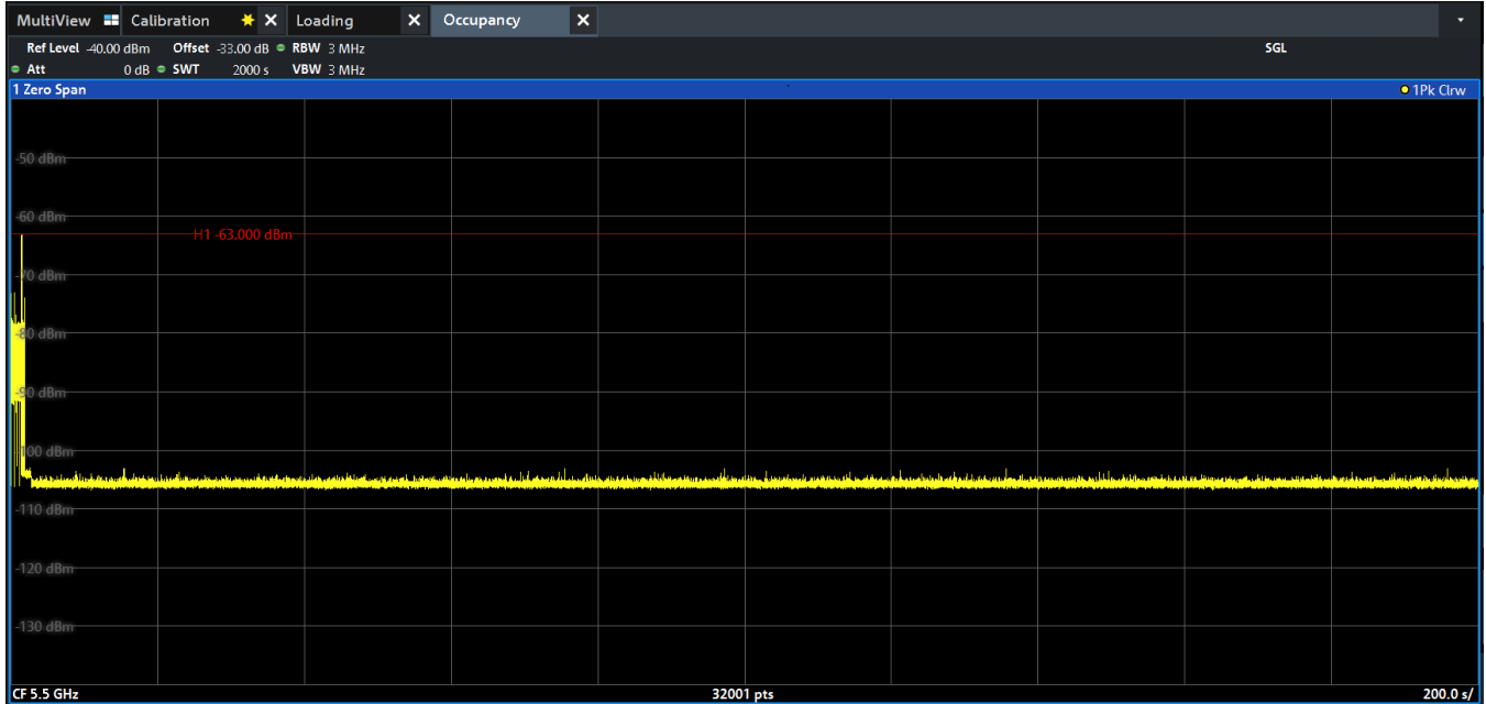
Figure 9-46. 5500MHz - Non-Occupancy Period (30 Minutes) - Mode 4 (20MHz)
