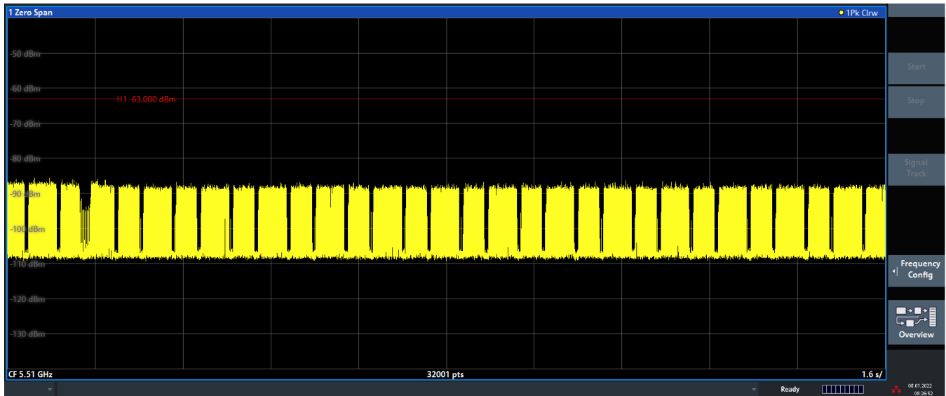
Figure 9-9. 5510MHz - Channel Loading - Mode 2 (40MHz)
