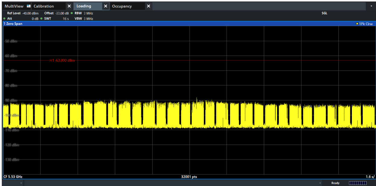
Figure 9-11. 5530MHz - Channel Loading - Mode 2 (80MHz)
