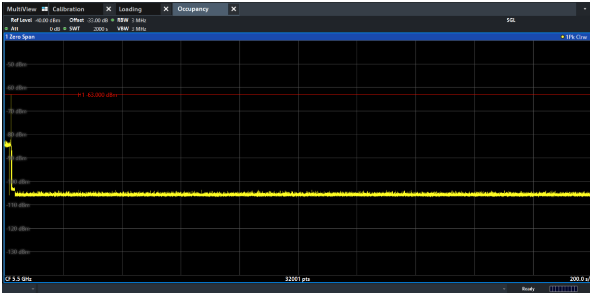
Figure 9-37. 5500MHz - Non-Occupancy Period (30 Minutes) - Mode 1 (20MHz)
