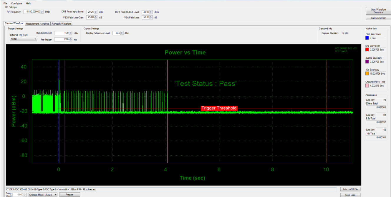
Figure 9-35. 5510MHz - Channel Move/ Closing Transmission Time - Mode 4 (40 MHz)
