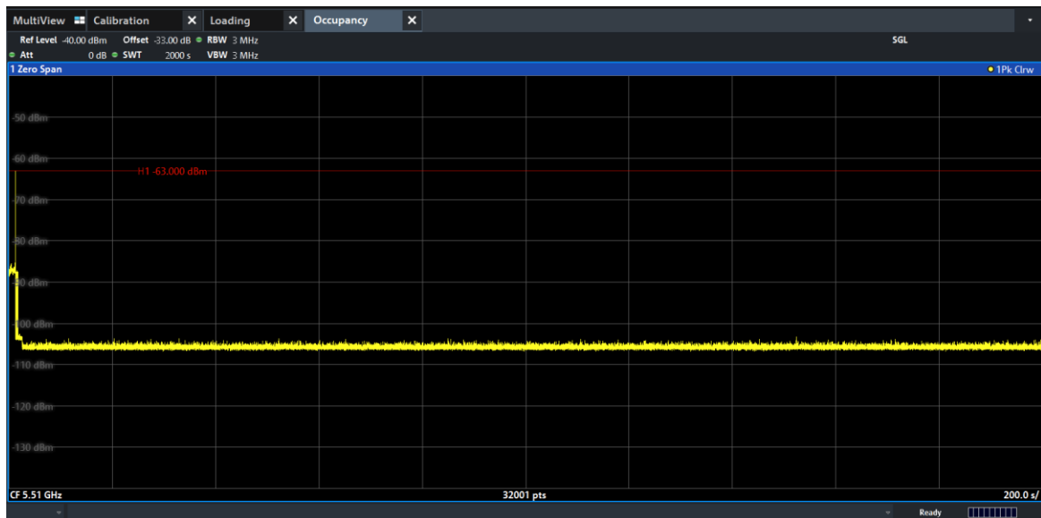
Figure 9-38. 5510MHz - Non-Occupancy Period (30 Minutes) - Mode 1 (40MHz)
