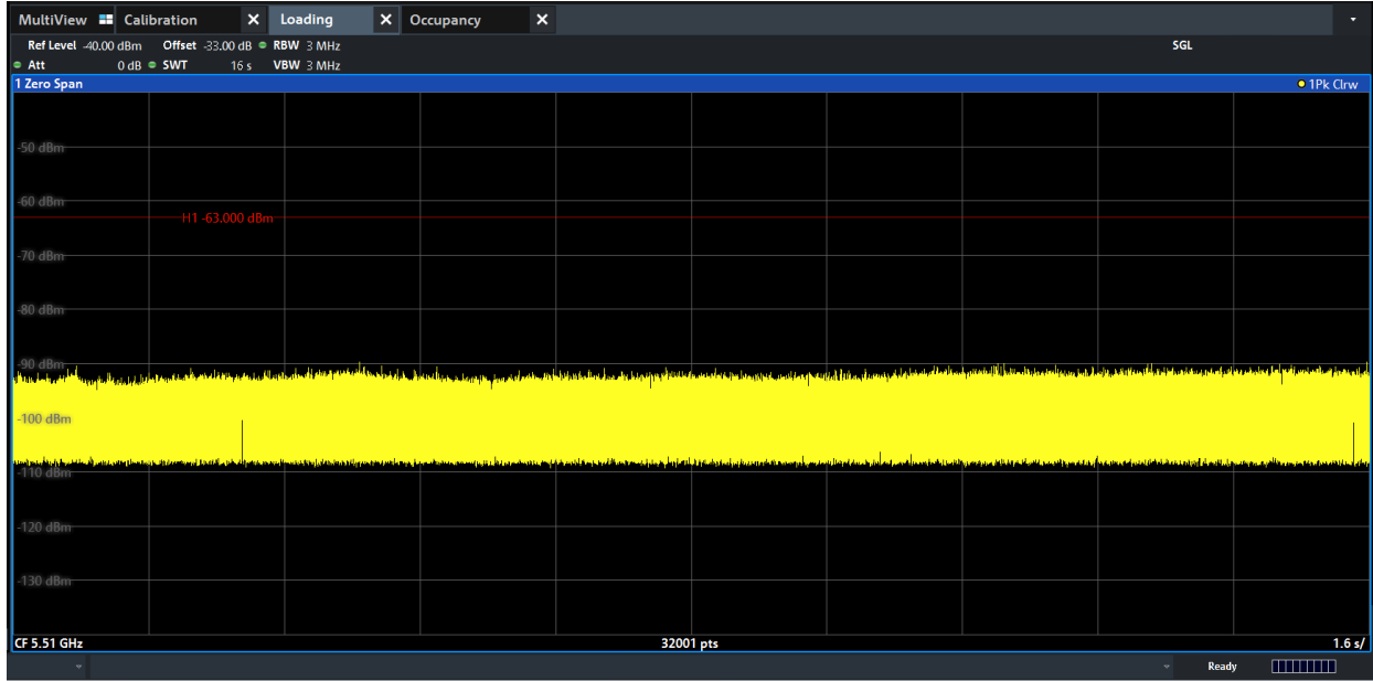
Figure 9-3. 5510MHz - Channel Loading - Mode 1 (40MHz)
