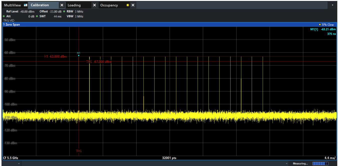
Figure 7-3. 5500MHz – Radar Pulse Type 0 (20MHz)
