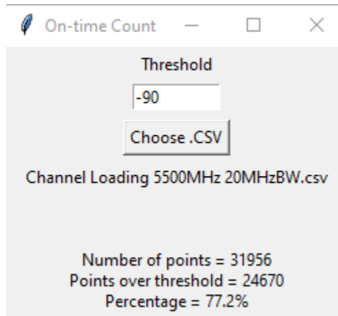
Figure 9-2. 5500MHz - Channel Loading Calculation - Mode 1 (20MHz)
