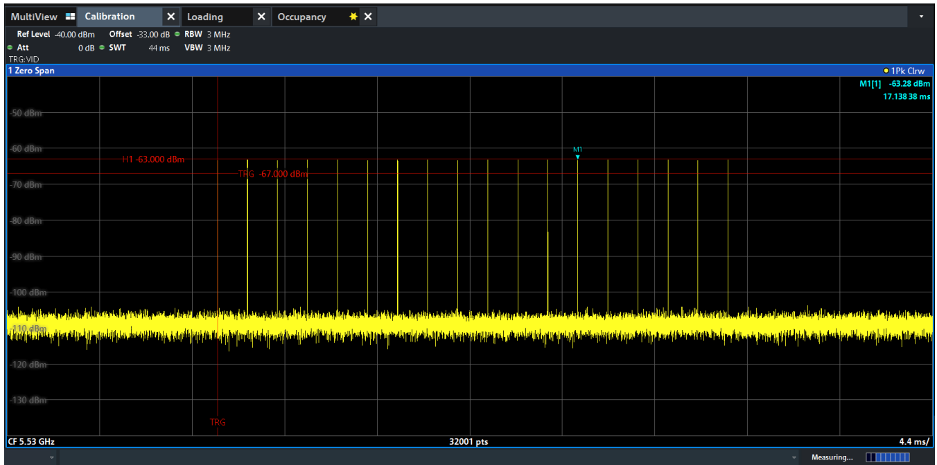
Figure 7-5. 5530MHz – Radar Pulse Type 0 (80MHz)
