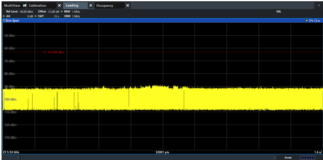
Figure 9-5. 5530MHz - Channel Loading - Mode 1 (80MHz)
