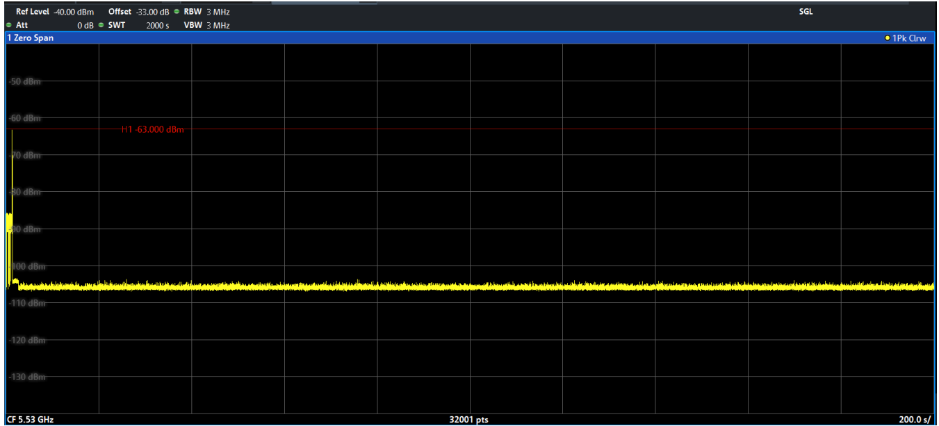
Figure 9-45. 5530MHz - Non-Occupancy Period (30 Minutes) - Mode 3 (80MHz)
