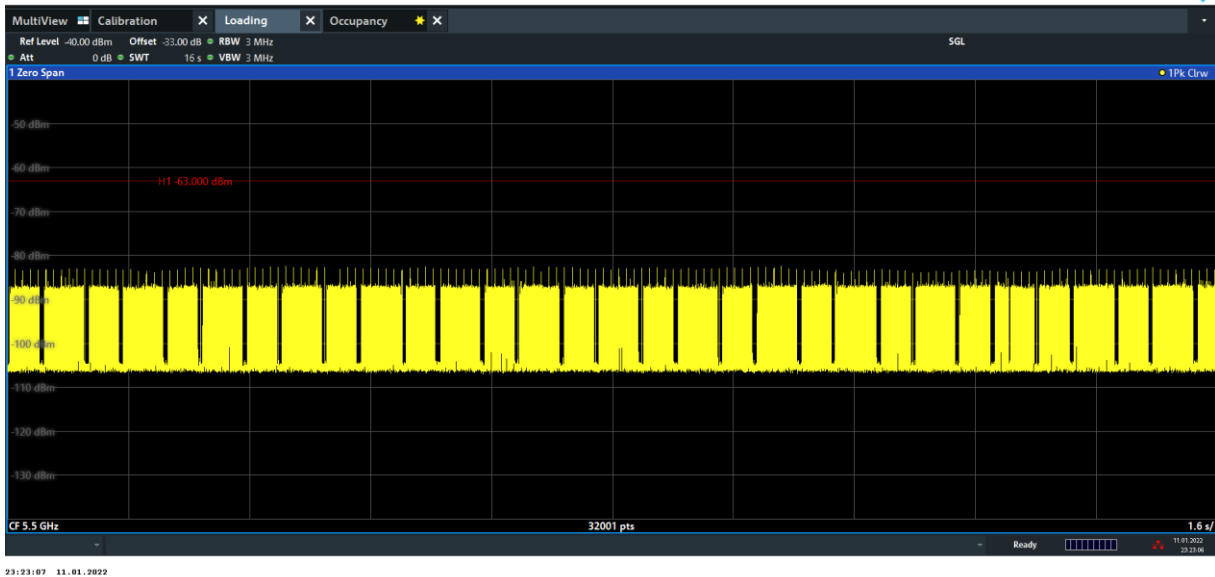
Figure 9-13. 5500MHz - Channel Loading - Mode 3 (20MHz)
