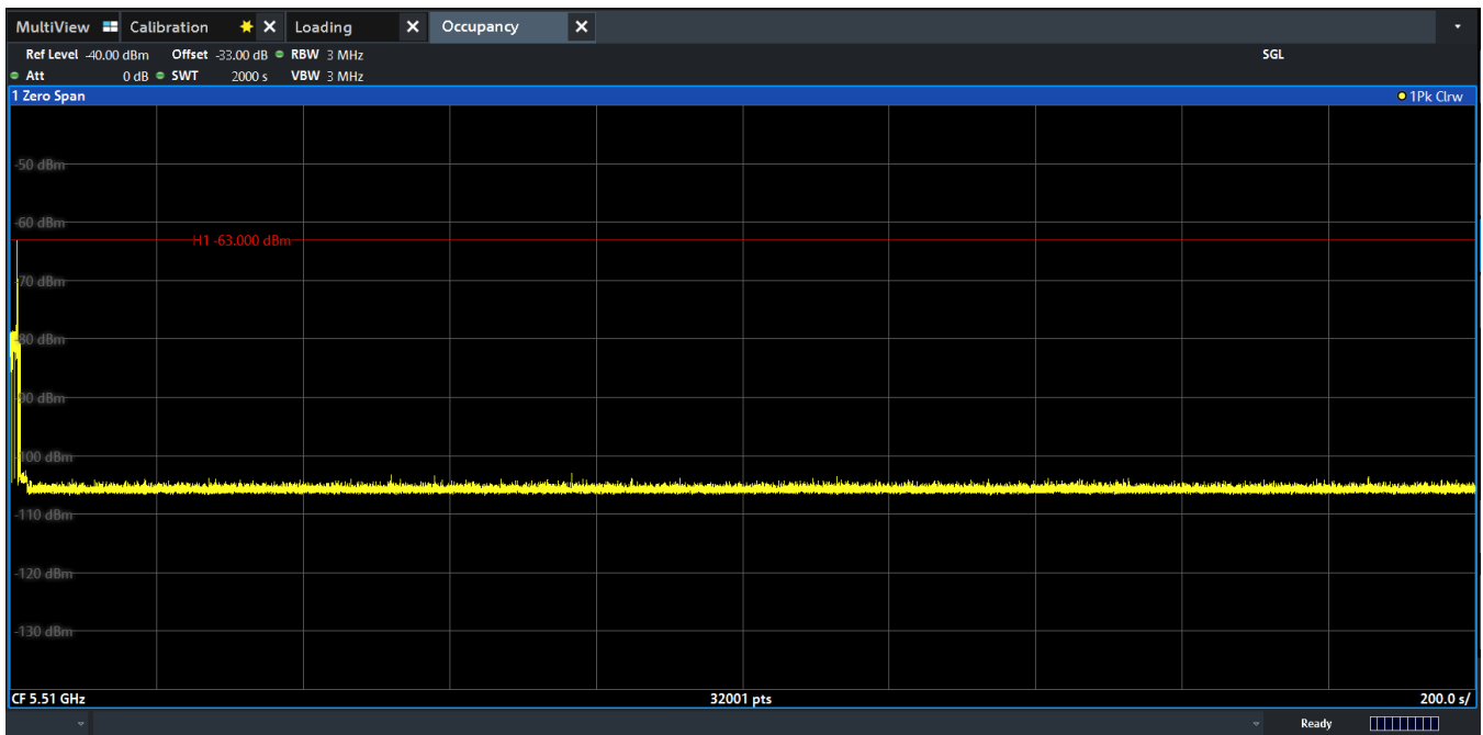
Figure 9-47. 5510MHz - Non-Occupancy Period (30 Minutes) - Mode 4 (40MHz)
