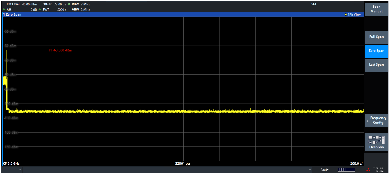
Figure 9-43. 5500MHz - Non-Occupancy Period (30 Minutes) - Mode 3 (20MHz)
