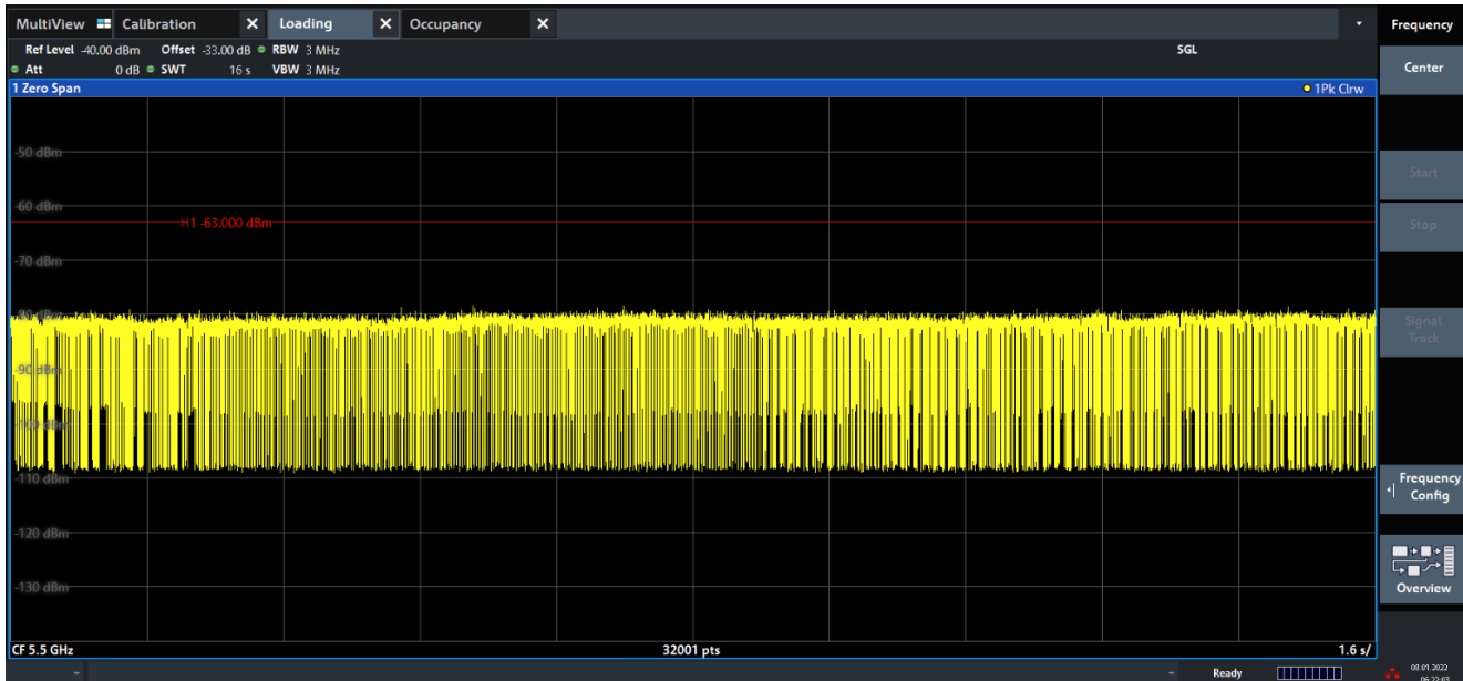
Figure 9-7. 5500MHz - Channel Loading - Mode 2 (20MHz)
