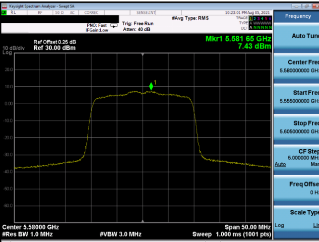
Plot 7-549. PSD CDD Antenna 5T (20MHz BW 802.11ax(SU) – Ch. 116, MCS3)
