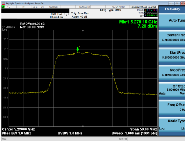
Plot 7-500. PSD SDM Antenna 3b (20MHz BW 802.11n – Ch. 56, MCS10)
