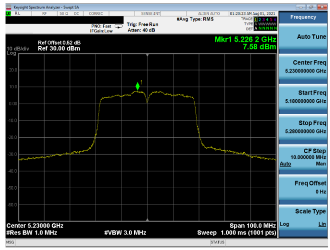
Plot 7-527. PSD SDM Antenna 5T (40MHz BW 802.11n – Ch. 46, MCS11)
