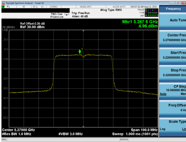
Plot 7-505. PSD SDM Antenna 5T (40MHz BW 802.11ax(SU) – Ch. 54, MCS2)
