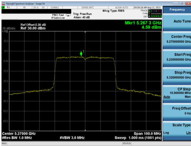
Plot 7-542. PSD SDM Antenna 3b (40MHz BW 802.11ax(SU) – Ch. 54, MCS3)
