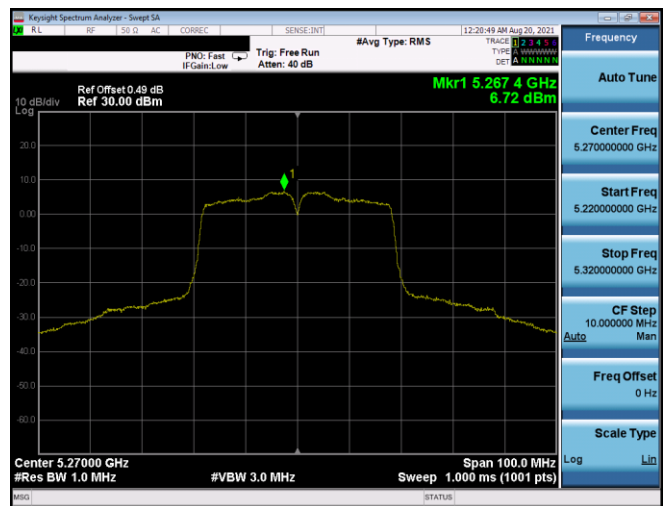
Plot 7-504. PSD SDM Antenna 3b (40MHz BW 802.11n – Ch. 54, MCS10)
