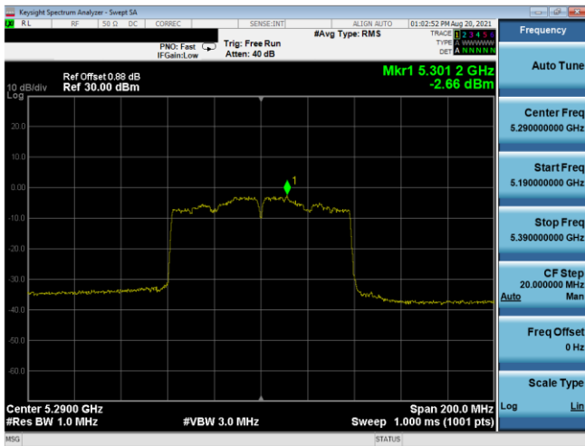
Plot 7-543. PSD CDD Antenna 5T (80MHz BW 802.11ac – Ch. 58, MCS3)
