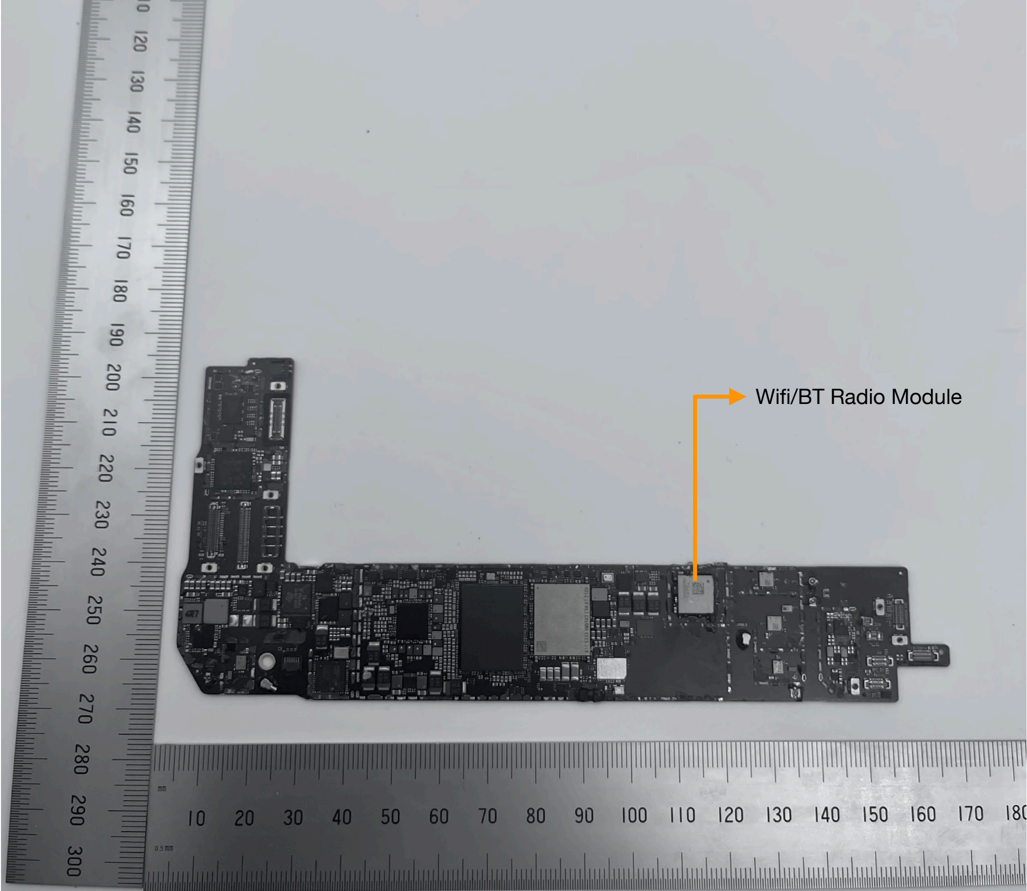
A2567 MLB with Shield Removed - Front
