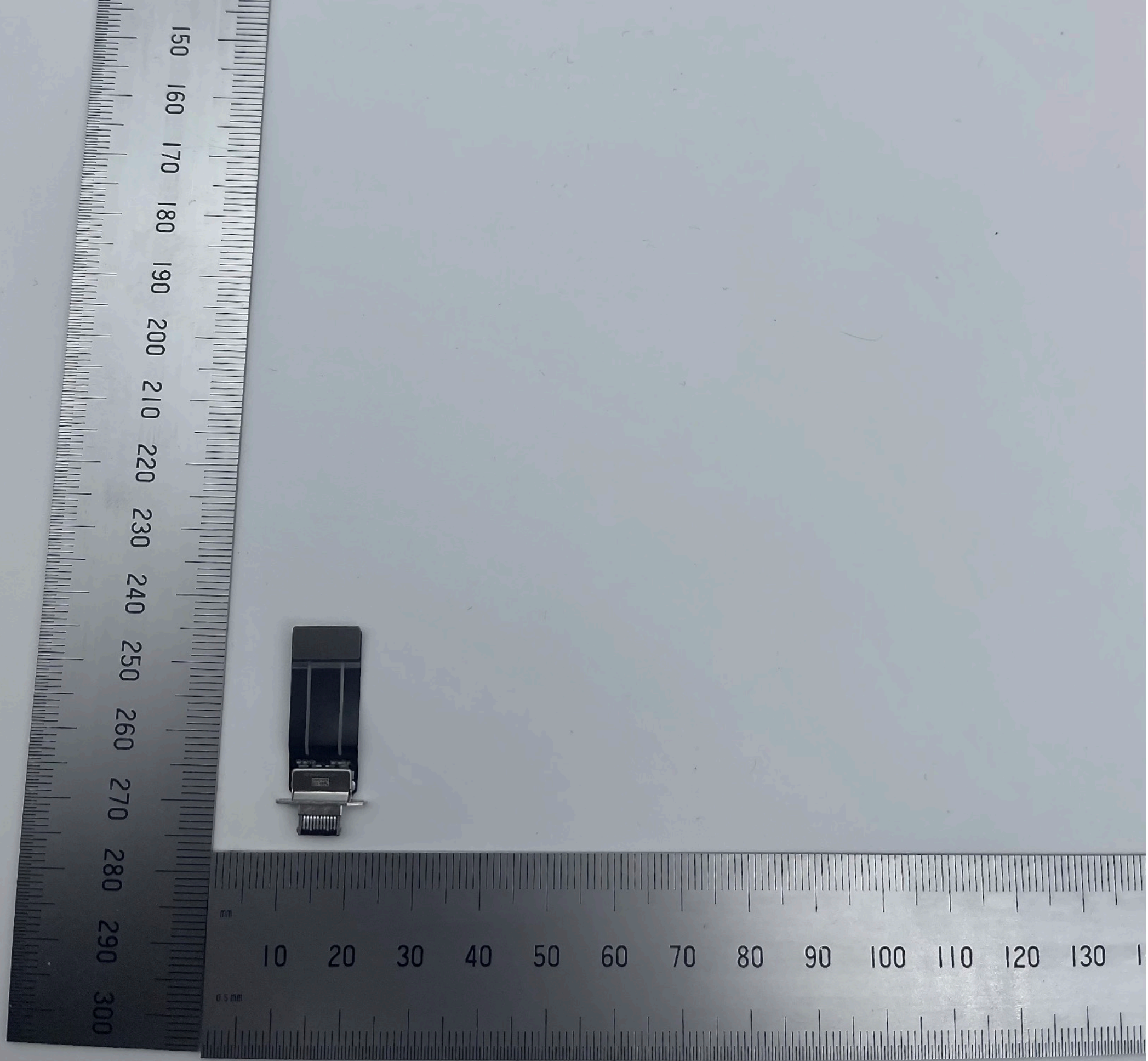
A2567 USB-C Connector Assembly - Front
