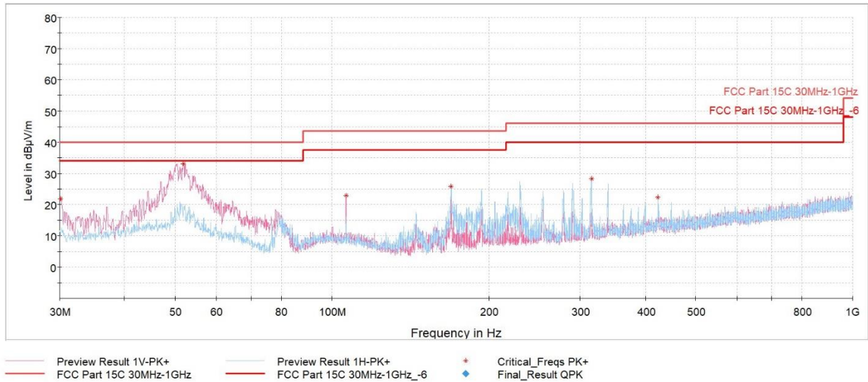
Plot 7-31. Radiated Spurious Emissions Below 1GHz (1Mbps, – Ch.19, Pol. H & V, with Tablet + AC/DC adaptor)
