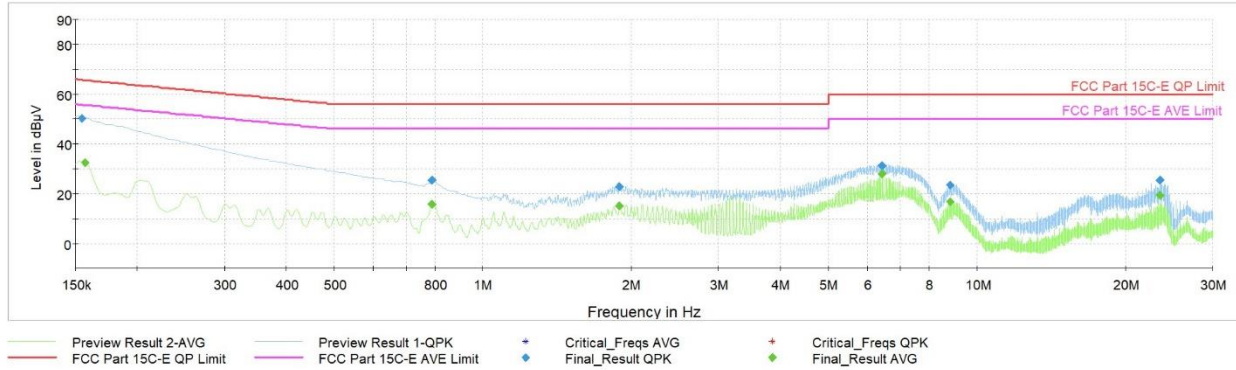
Plot 7-33. AC Line Conducted Plot with Bluetooth LE (N, 1Mbps – Ch.19, with Tablet + Laptop)
