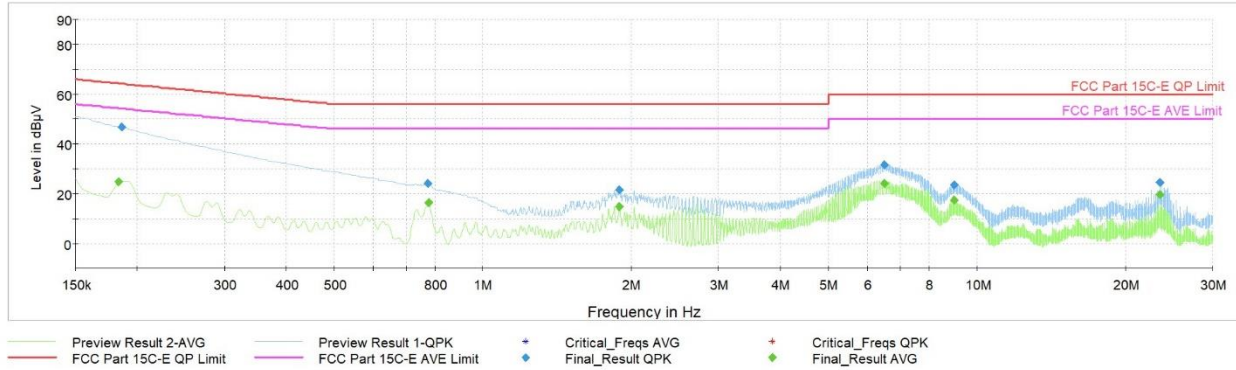
Plot 7-32. AC Line Conducted Plot with Bluetooth LE (L1, 1Mbps- Ch.19 with Tablet + Laptop)
