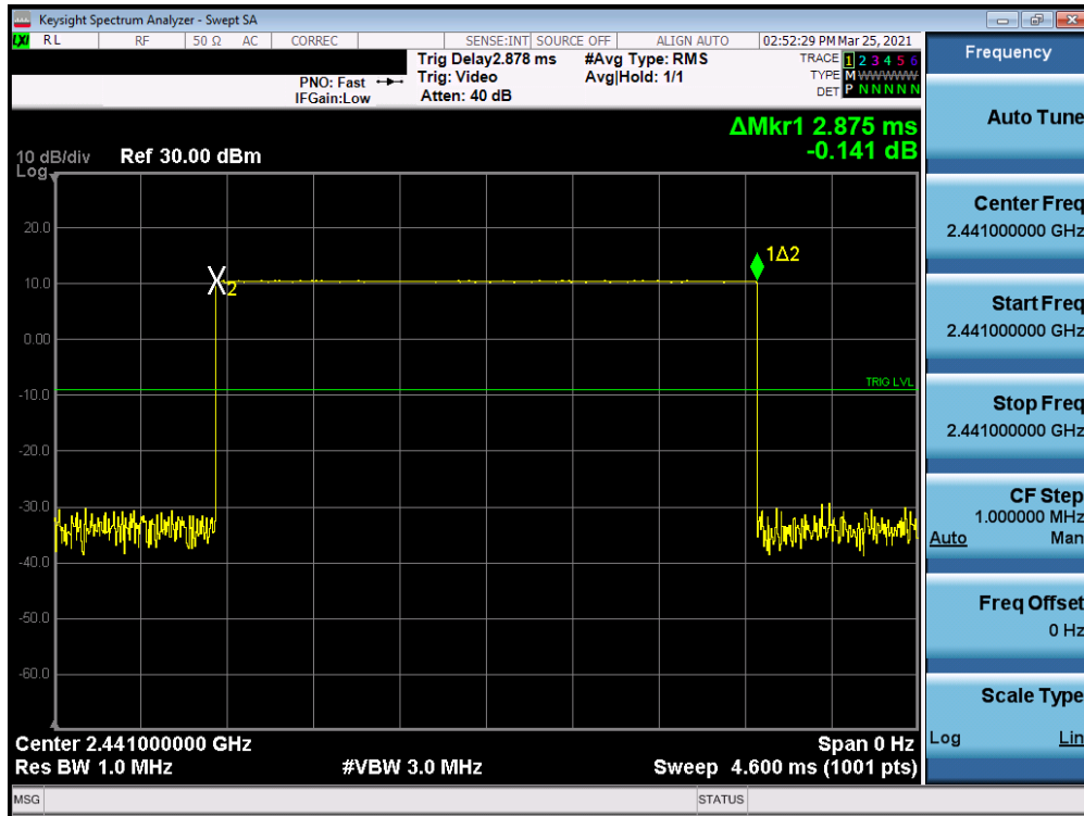
Plot 7-17. Conducted Time of Occupancy (Bluetooth, GFSK)
