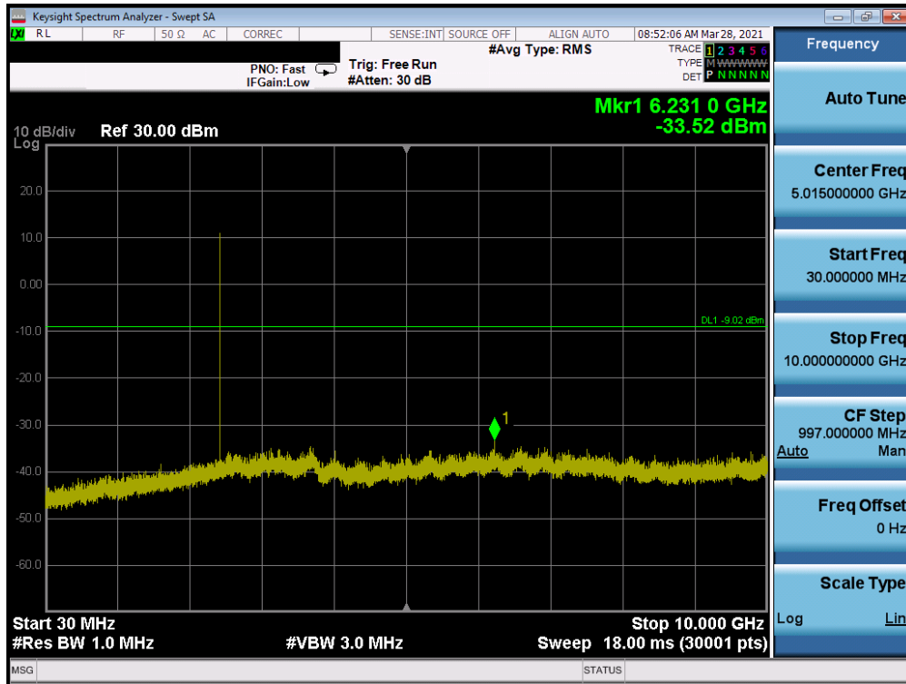
Plot 7-25. Conducted Spurious Emissions (Bluetooth, GFSK, Ch. 39)
