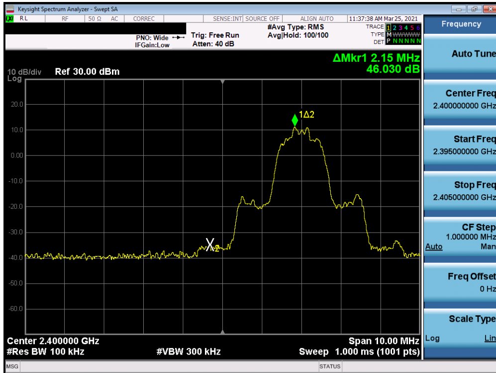
Plot 7-11. Conducted Band Edge (Bluetooth with Hopping Disabled, 8DPSK, Ch. 0)
