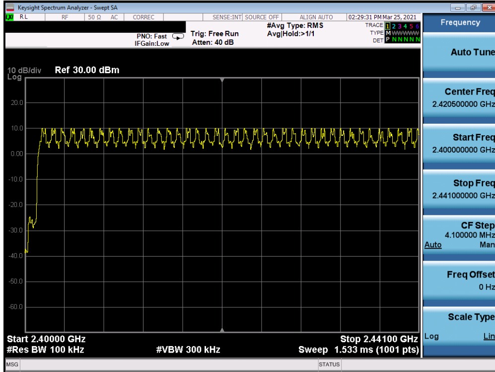
Plot 7-21. Conducted Low End Spectrum Channel Hopping (Bluetooth, 8DPSK)
