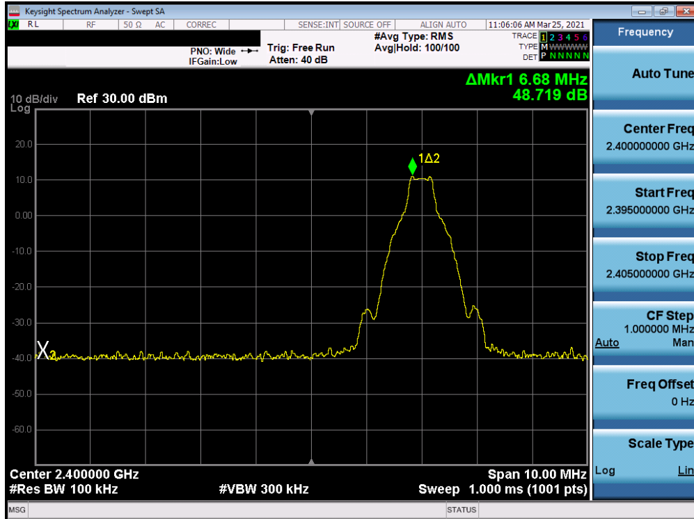
Plot 7-7. Conducted Band Edge (Bluetooth with Hopping Disabled, GFSK, Ch. 0)
