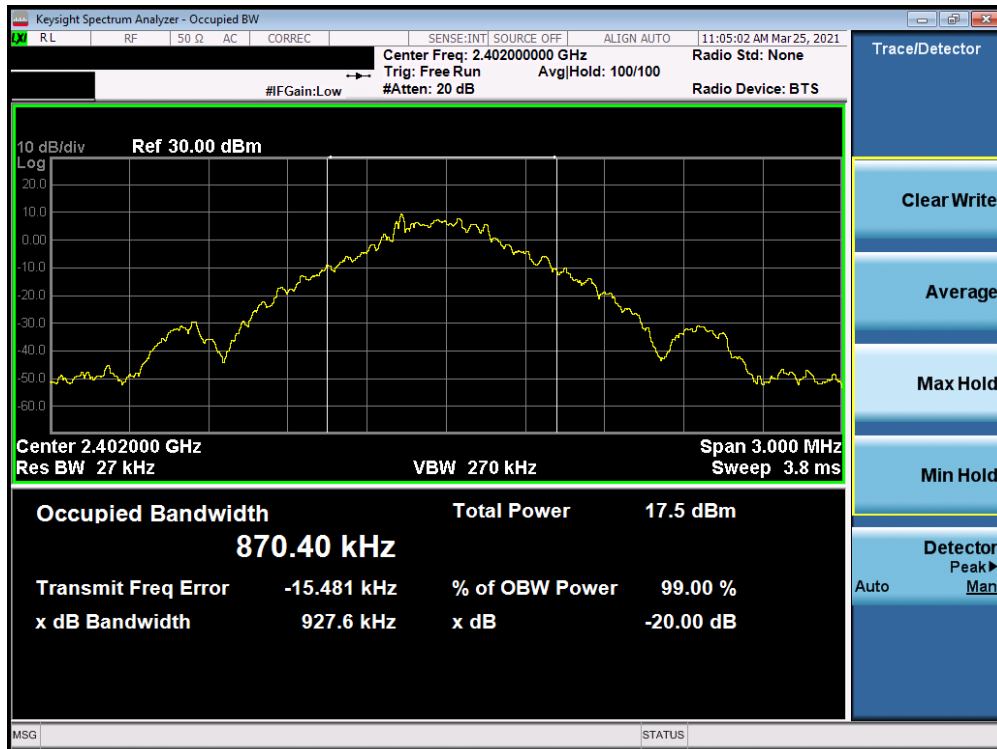
Plot 7-1. Conducted 20dB BW and 99% OBW (Bluetooth, GFSK, Ch. 0)
