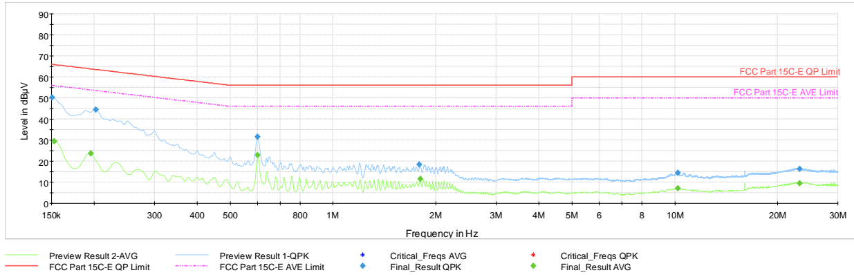
Plot 7-39. AC Line-Conducted Test Plot (L1, GFSK – Ch.39, with Laptop and Charging Case)
