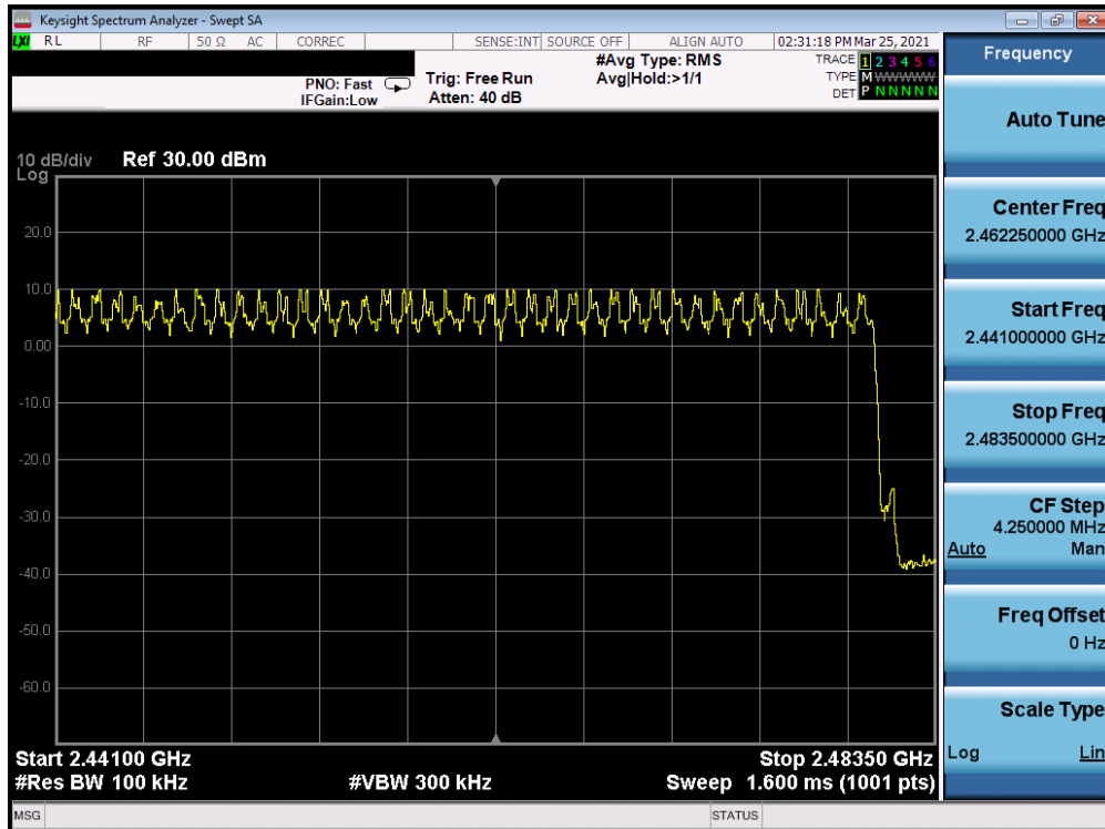
Plot 7-22. Conducted High End Spectrum Channel Hopping (Bluetooth, 8DPSK)
