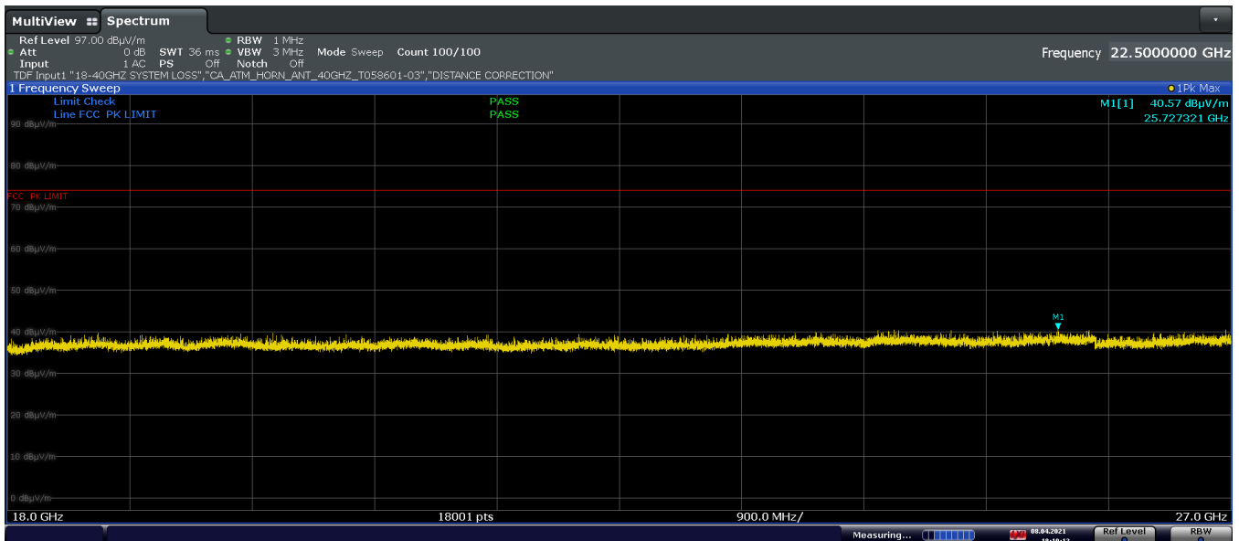
Plot 7-33. Radiated Spurious Emissions Above 18GHz (GFSK - Ch.39, Pol. V)
