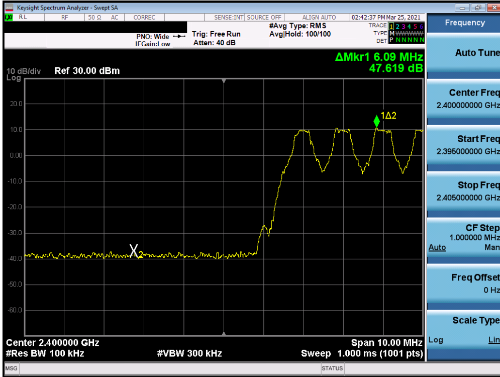
Plot 7-9. Conducted Band Edge (Bluetooth with Hopping Enabled, GFSK)
