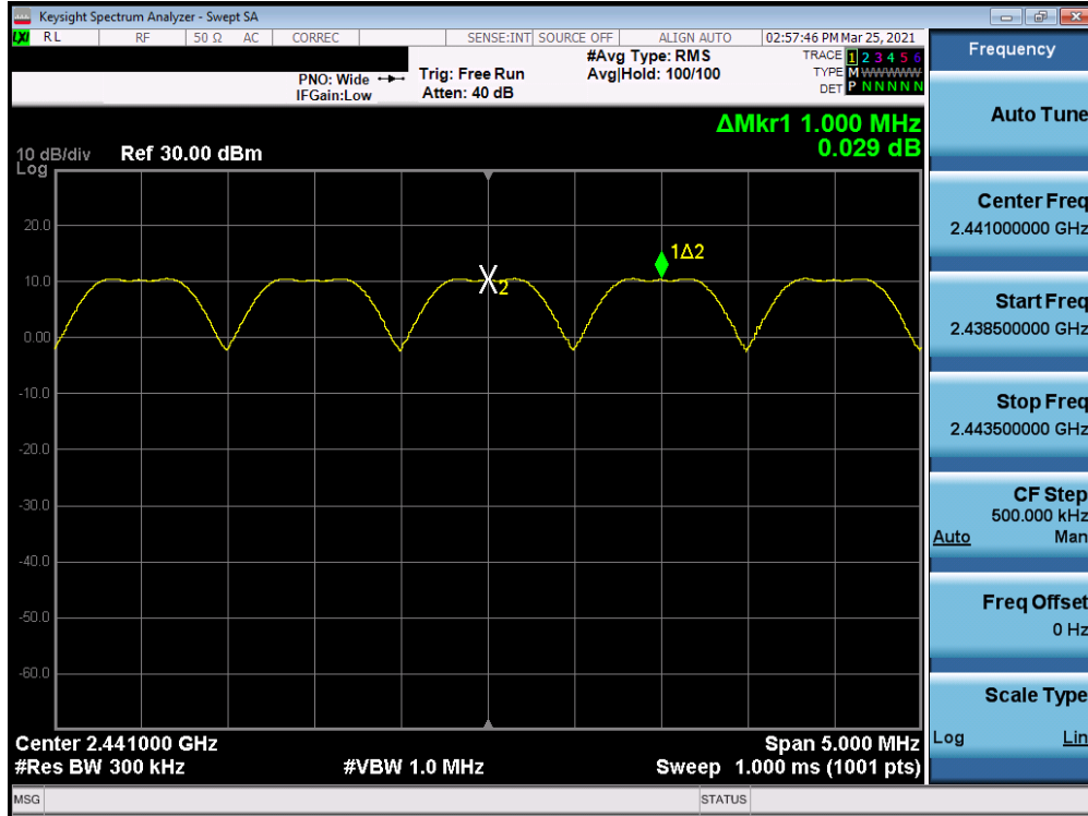
Plot 7-15. Conducted Channel Spacing (Bluetooth, GFSK)
