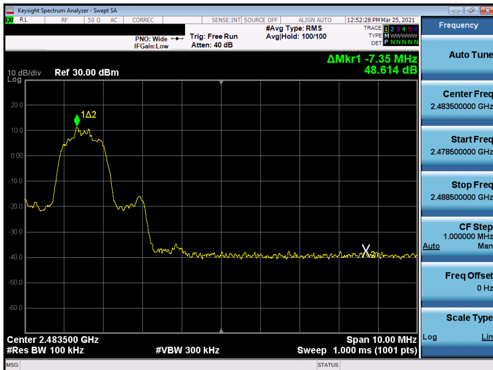
Plot 7-12. Conducted Band Edge (Bluetooth with Hopping Disabled, 8DPSK, Ch. 78)
