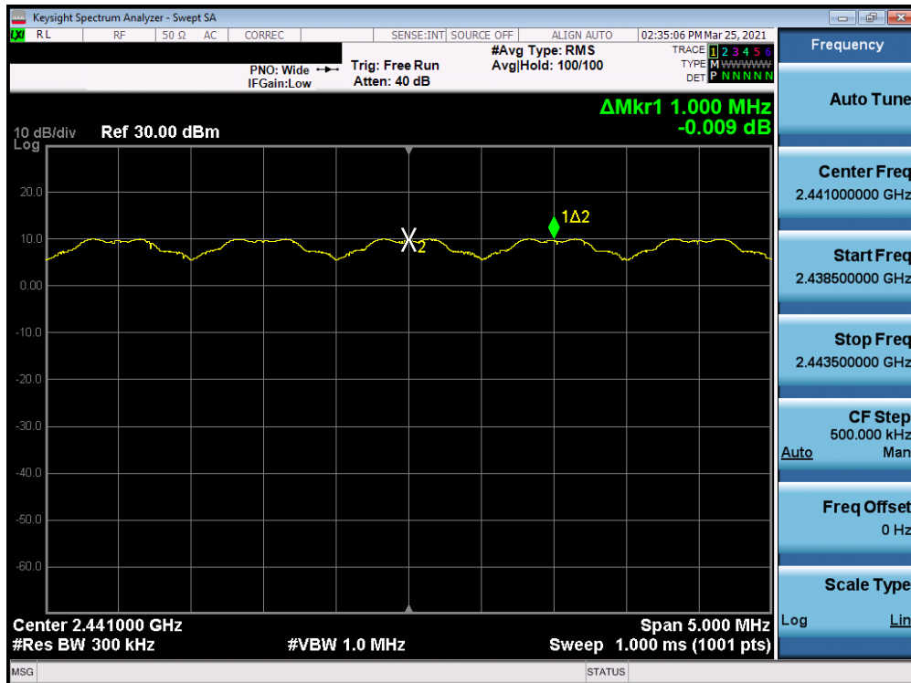
Plot 7-16. Conducted Channel Spacing (Bluetooth, 8DPSK)
