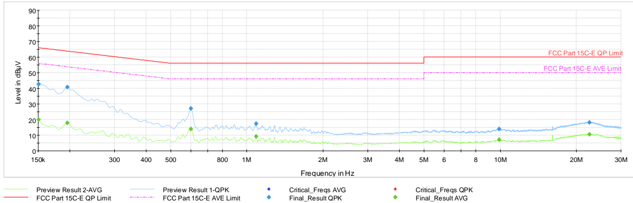
Plot 7-40. AC Line-Conducted Test Plot (N, GFSK – Ch.39, with Laptop and Charging Case)
