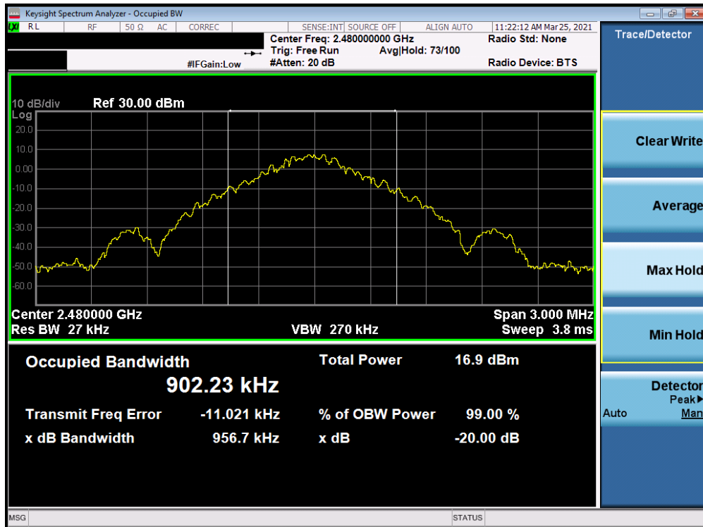
Plot 7-3. Conducted 20dB BW and 99% OBW (Bluetooth, GFSK, Ch. 78)
