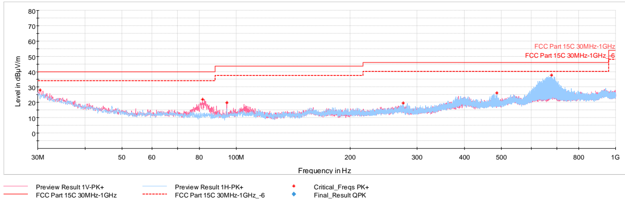
Plot 7-38. Radiated Spurious Emissions Below 1GHz (GFSK – Ch.39, with Laptop and Charging Case)
