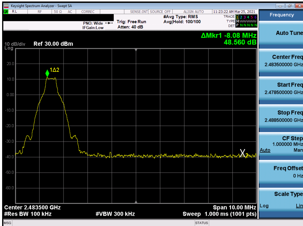
Plot 7-8. Conducted Band Edge (Bluetooth with Hopping Disabled, GFSK, Ch. 78)
