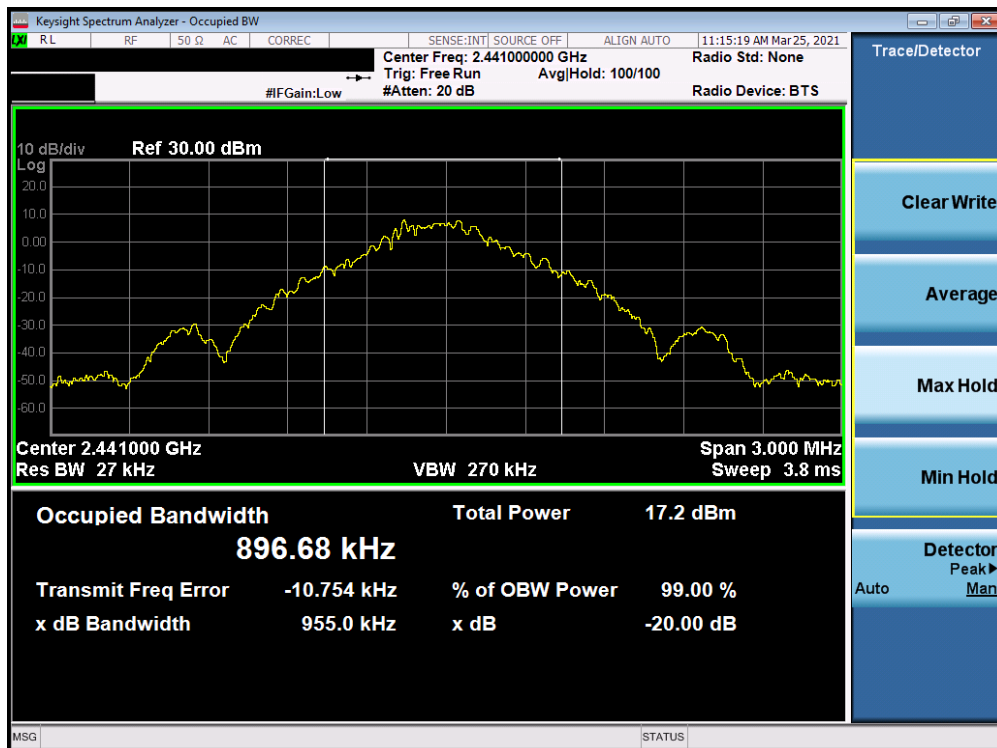
Plot 7-2. Conducted 20dB BW and 99% OBW (Bluetooth, GFSK, Ch. 39)
