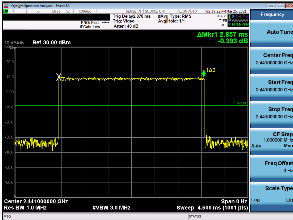
Plot 7-18. Conducted Time of Occupancy (Bluetooth, 8DPSK)
