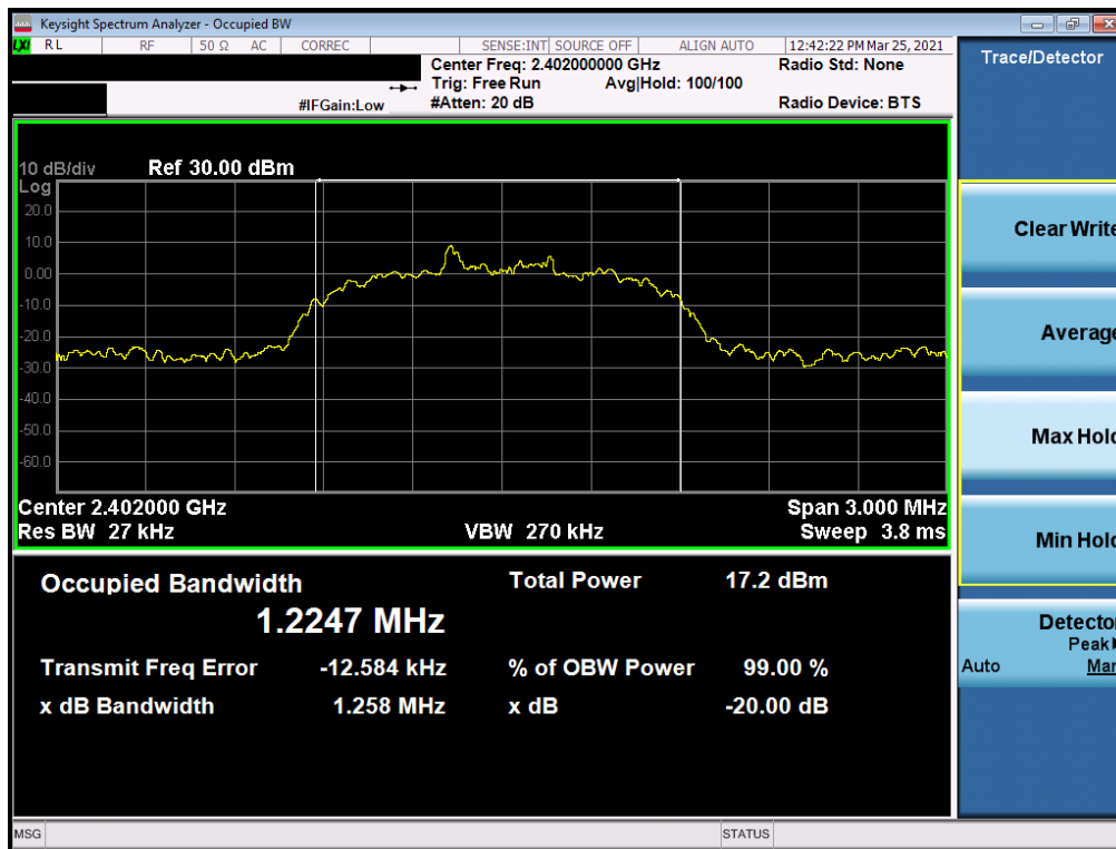
Plot 7-4. Conducted 20dB BW and 99% OBW (Bluetooth, 8DPSK, Ch. 0)
