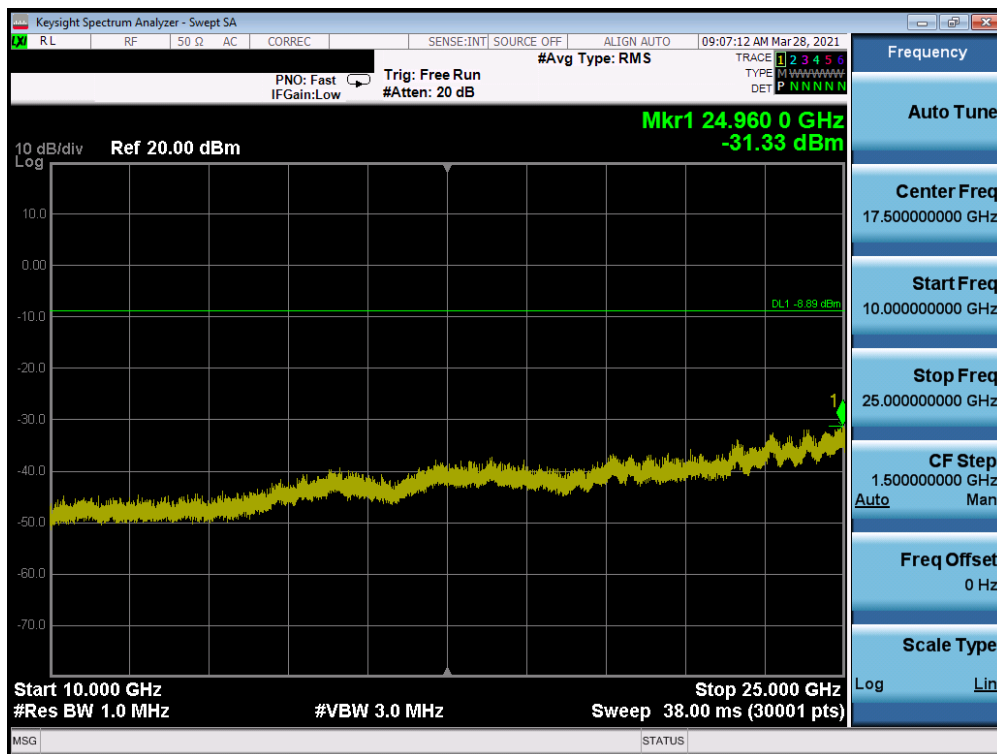
Plot 7-28. Conducted Spurious Emissions (Bluetooth, GFSK, Ch. 78)
