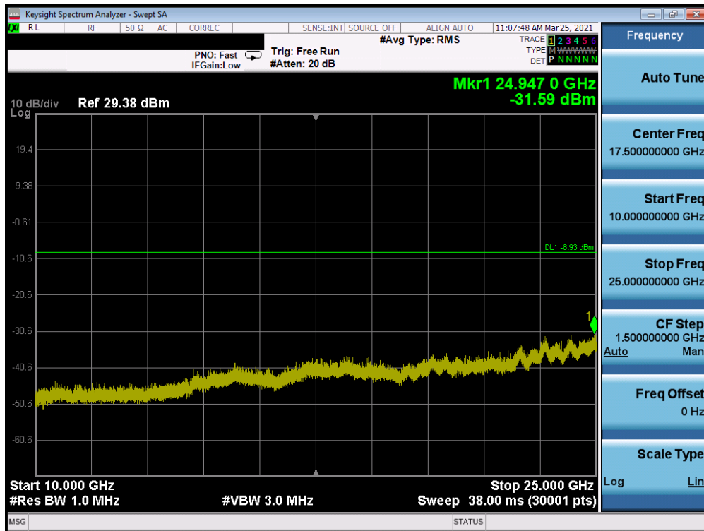
Plot 7-24. Conducted Spurious Emissions (Bluetooth, GFSK, Ch. 0)
