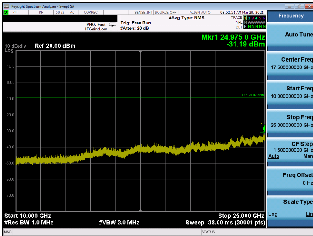
Plot 7-26. Conducted Spurious Emissions (Bluetooth, GFSK, Ch. 39)
