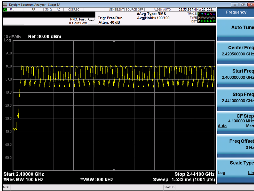
Plot 7-19. Conducted Low End Spectrum Channel Hopping (Bluetooth, GFSK)
