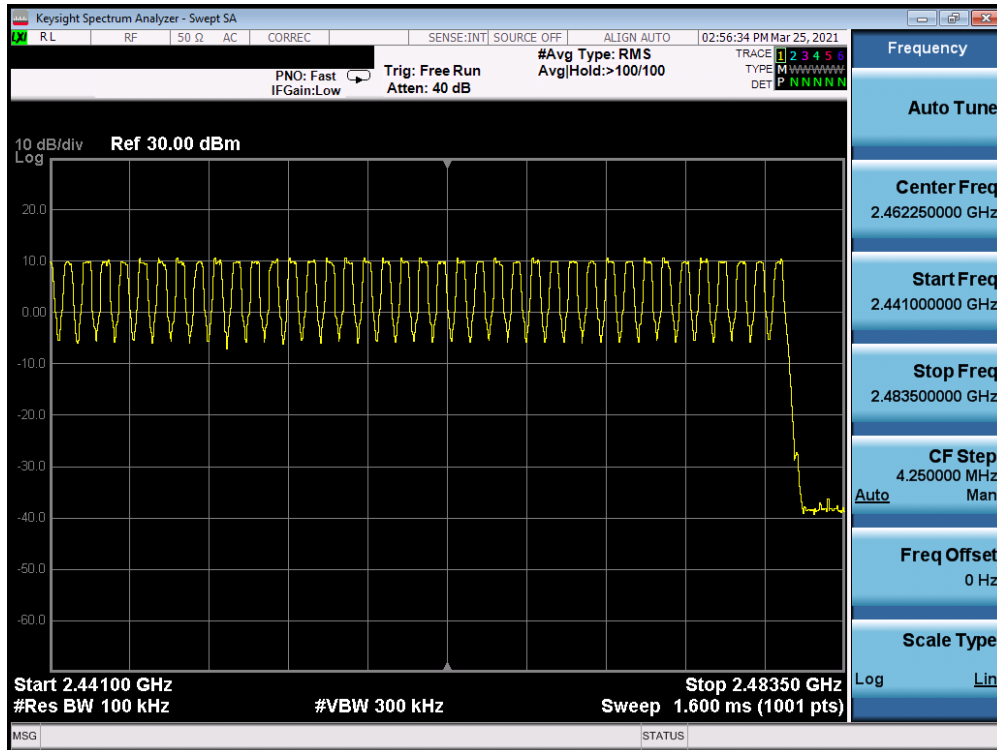
Plot 7-20. Conducted High End Spectrum Channel Hopping (Bluetooth, GFSK)
