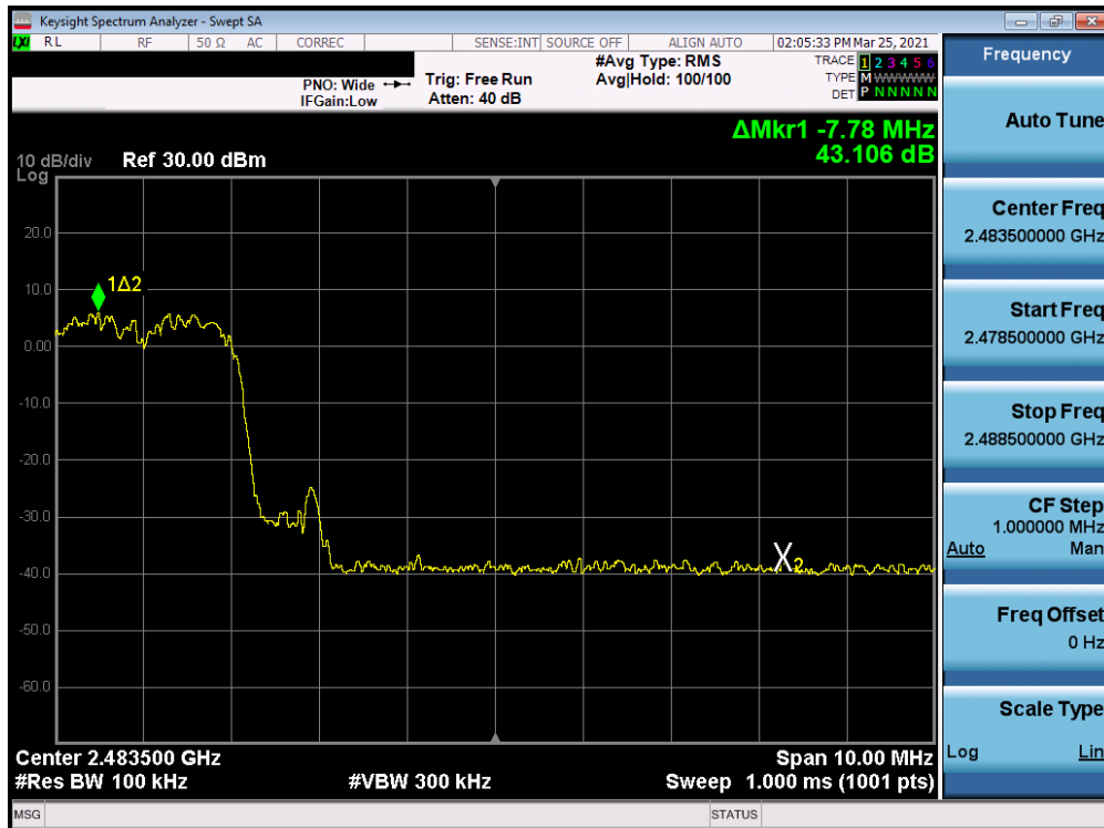
Plot 7-14. Conducted Band Edge (Bluetooth with Hopping Enabled, 8DPSK)
