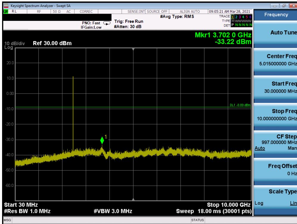
Plot 7-27. Conducted Spurious Emissions (Bluetooth, GFSK, Ch. 78)
