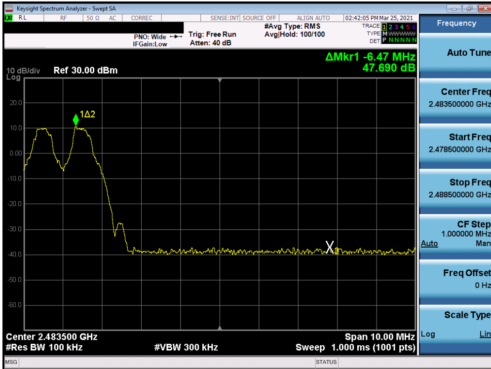
Plot 7-10. Conducted Band Edge (Bluetooth with Hopping Enabled, GFSK)
