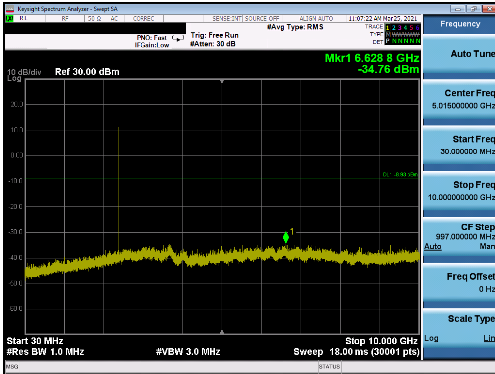
Plot 7-23. Conducted Spurious Emissions (Bluetooth, GFSK, Ch. 0)
