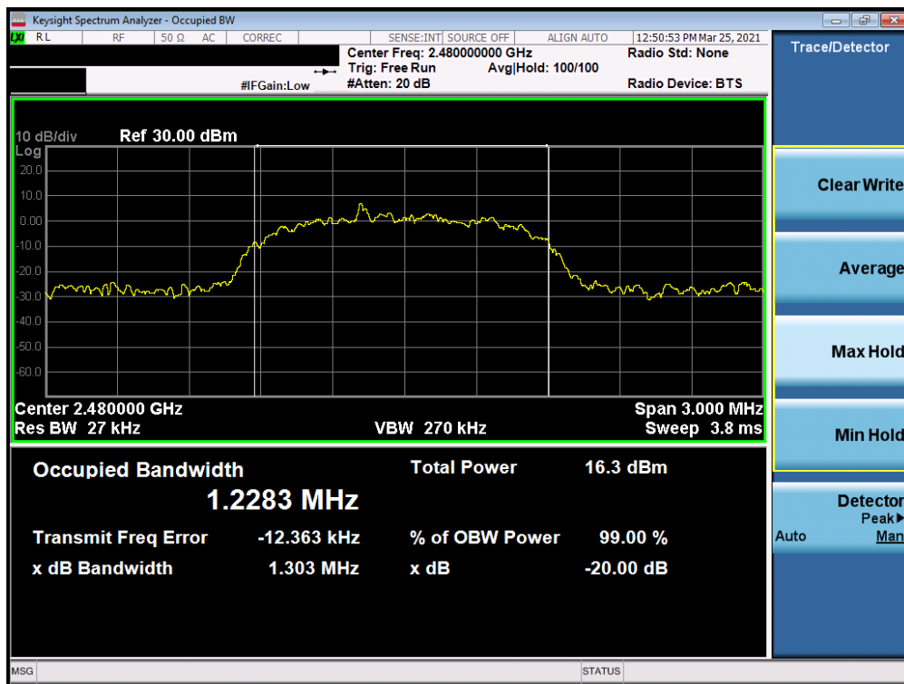
Plot 7-6. Conducted 20dB BW and 99% OBW (Bluetooth, 8DPSK, Ch. 78)
