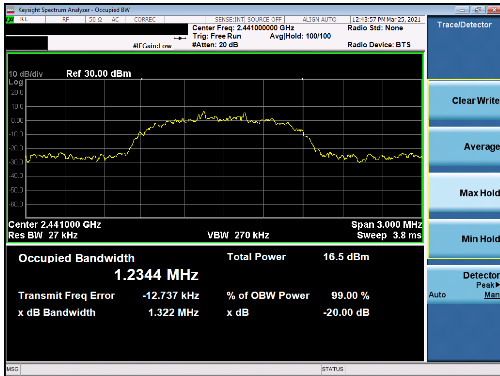
Plot 7-5. Conducted 20dB BW and 99% OBW (Bluetooth, 8DPSK, Ch. 39)
