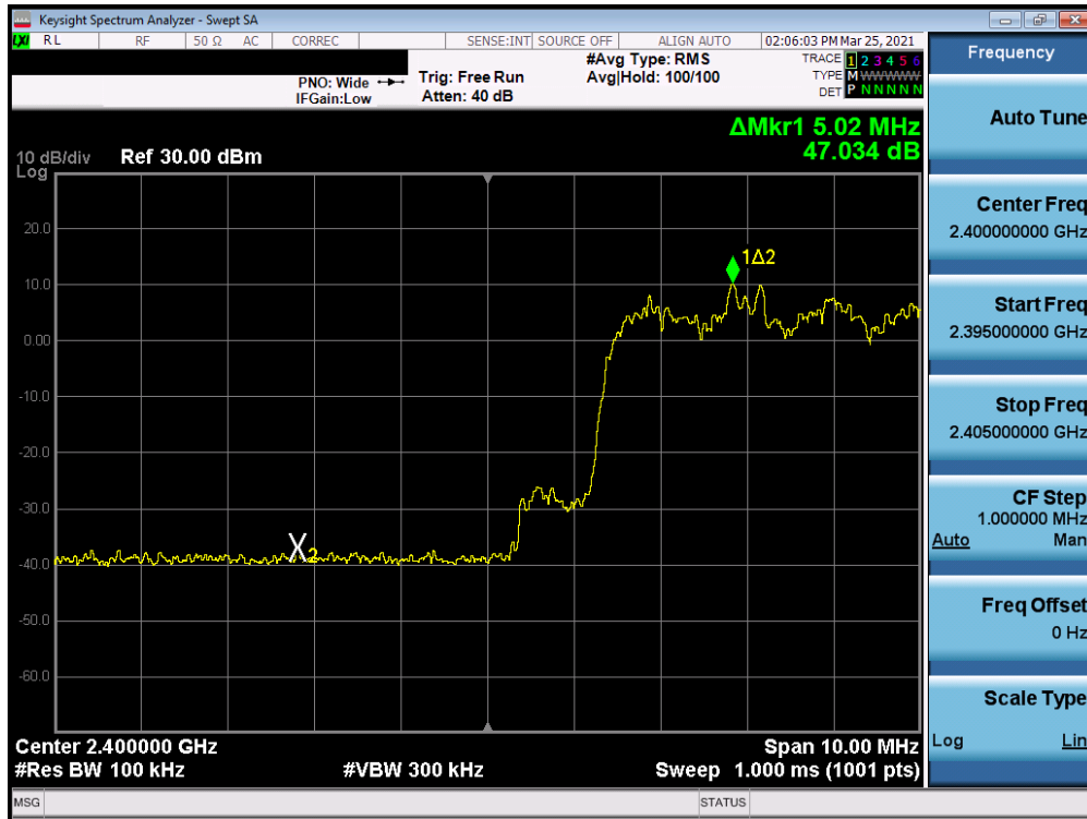
Plot 7-13. Conducted Band Edge (Bluetooth with Hopping Enabled, 8DPSK)
