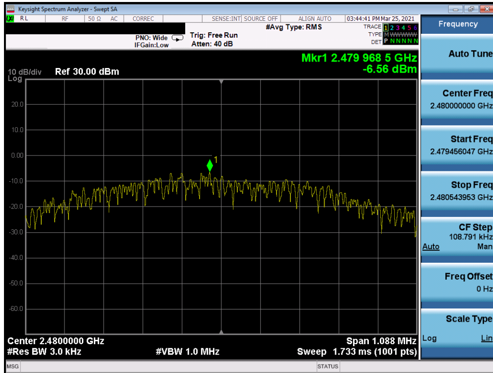
Plot 7-9. Power Spectral Density (Bluetooth (LE), 1Mbps,- Ch. 39)
