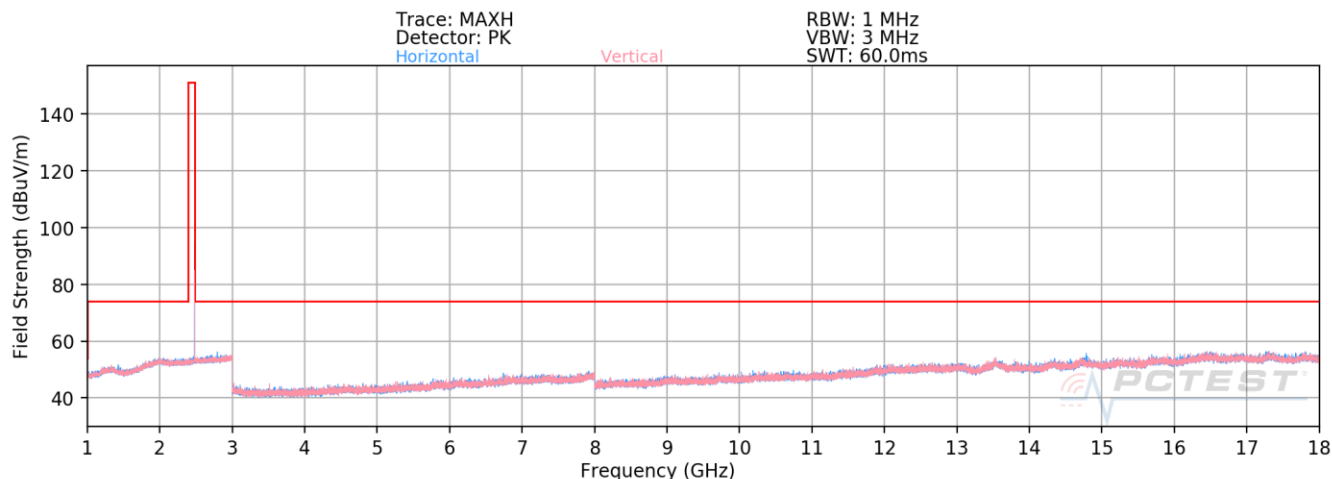
Plot 7-25. Radiated Spurious Emissions Above 1GHz (1Mbps – Ch. 39)
