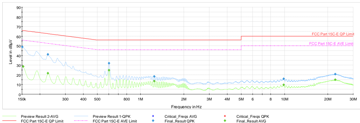
Plot 7-34. AC Line Conducted Plot with Bluetooth LE (1Mbps, – Ch.19, N, with Laptop and Charging Case)
