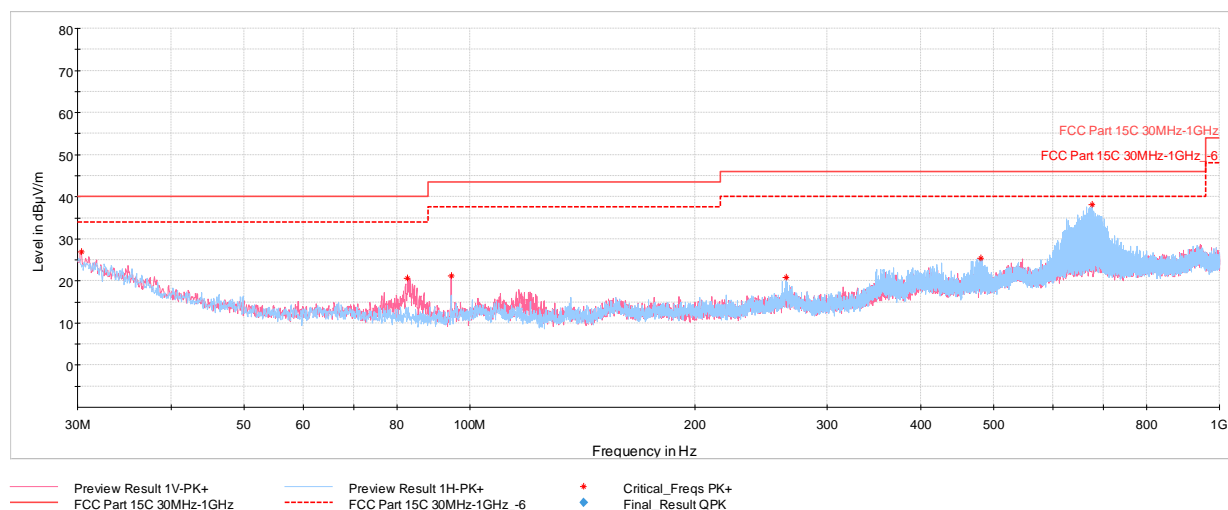
Plot 7-32. Radiated Spurious Emissions Below 1GHz (1Mbps, Ch.19, Pol. H&V, with Laptop and Charging Case)
