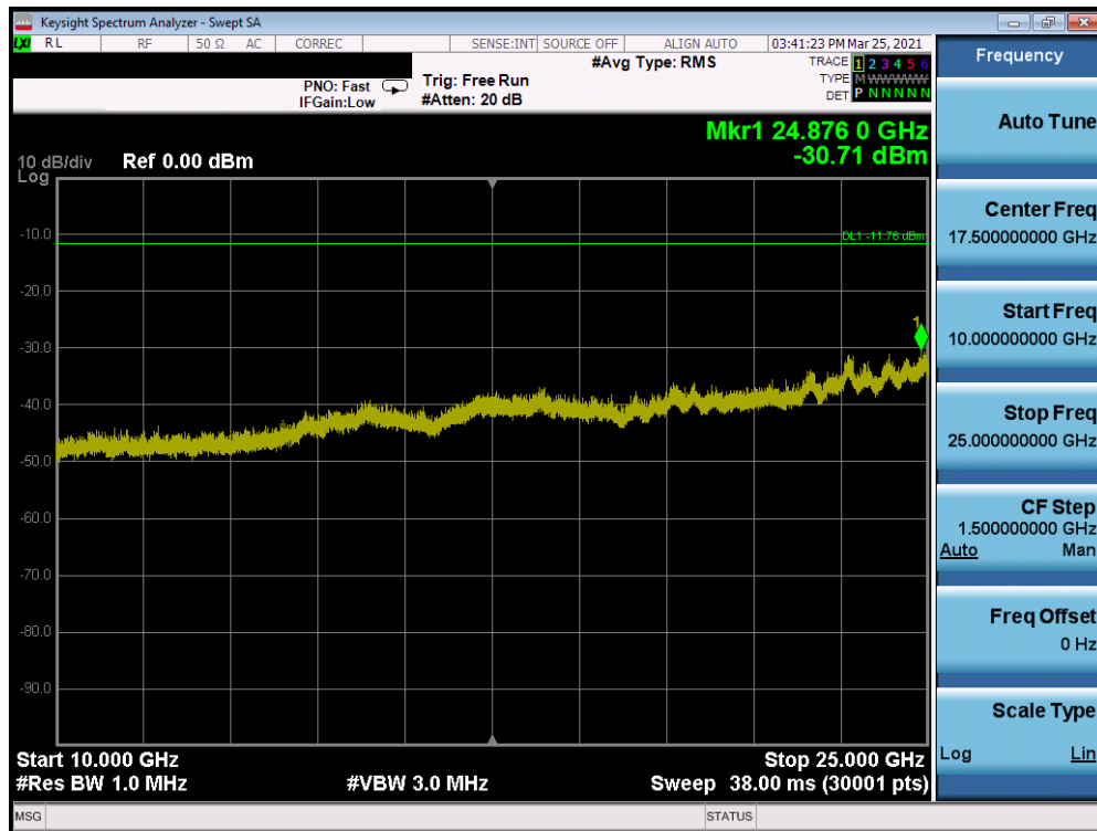
Plot 7-18. Conducted Spurious Emissions (Bluetooth (LE), 1Mbps,- Ch. 0)
