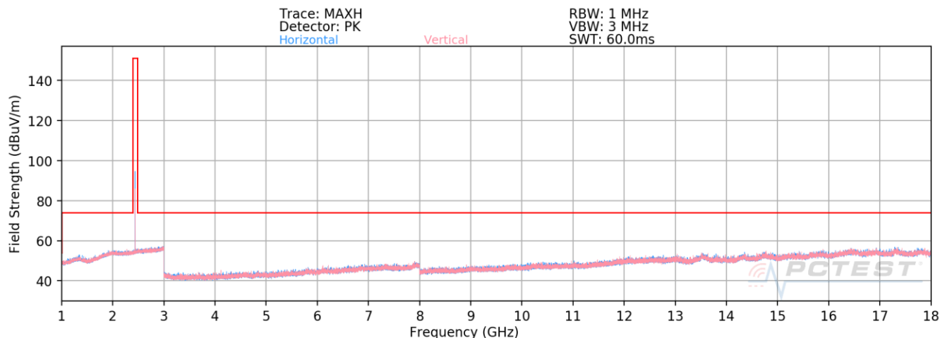
Plot 7-24. Radiated Spurious Emissions Above 1GHz (1Mbps, – Ch. 19)
