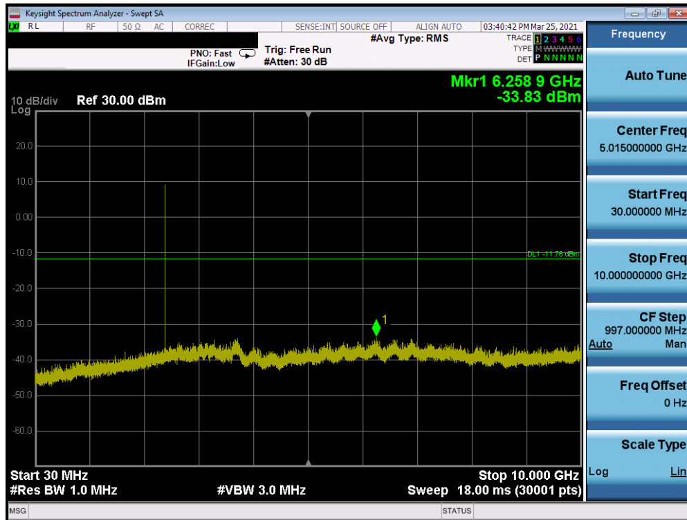
Plot 7-17. Conducted Spurious Emissions (Bluetooth (LE), 1Mbps,- Ch. 0)
