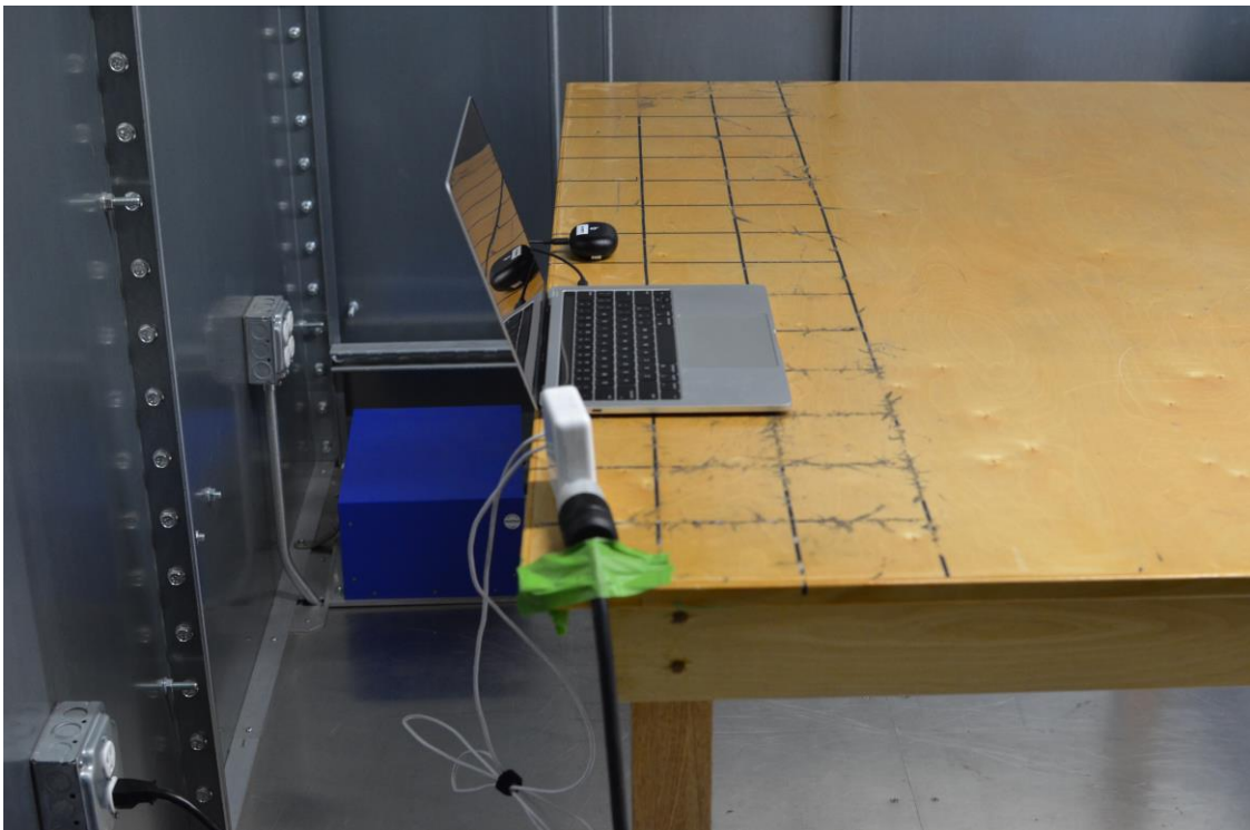
Figure 12: AC Line Test Setup (Side View)
