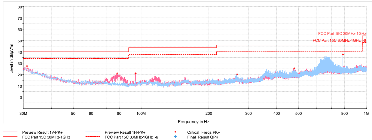
Plot 7-38. Radiated Spurious Emissions Below 1GHz (GFSK – Ch.39, with Laptop and Charging Case)
