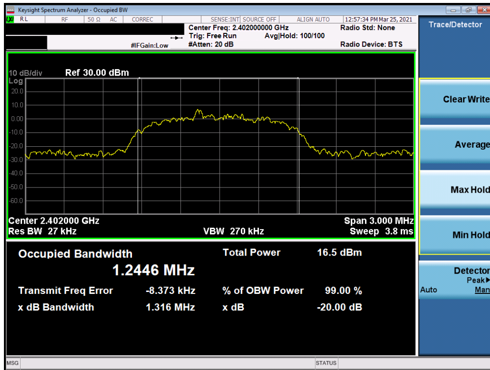
Plot 7-4. Conducted 20dB BW and 99% OBW (Bluetooth, 8DPSK, Ch. 0)
