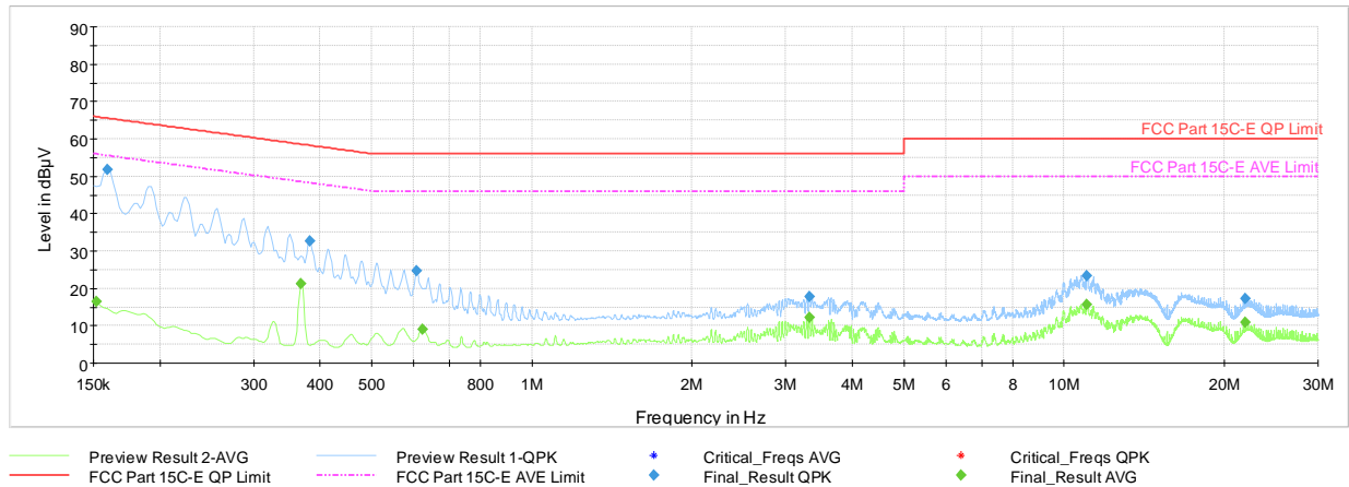
Plot 7-39. AC Line-Conducted Test Plot (L1, GFSK – Ch.39, with Laptop and Charging Case)
