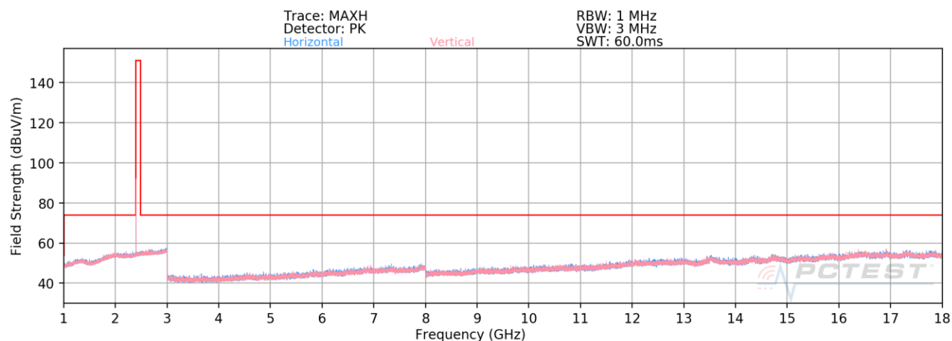
Plot 7-29. Radiated Spurious Emissions above 1GHz (BT GFSK – Ch. 0)
