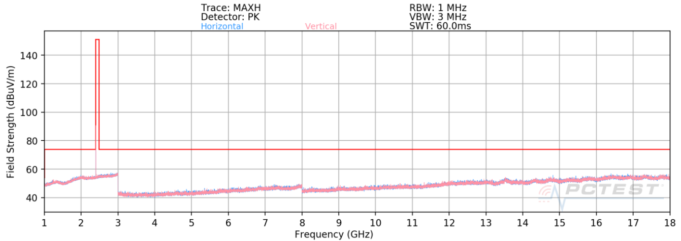
Plot 7-23. Radiated Spurious Emissions Above 1GHz (1Mbps, – Ch. 0)
