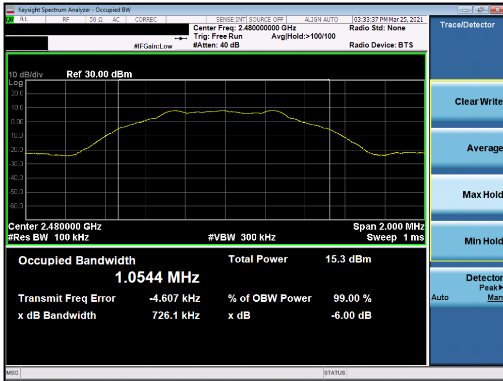
Plot 7-3. 6dB BW & 99% OBW (Bluetooth (LE), 1Mbps,- Ch. 39)
