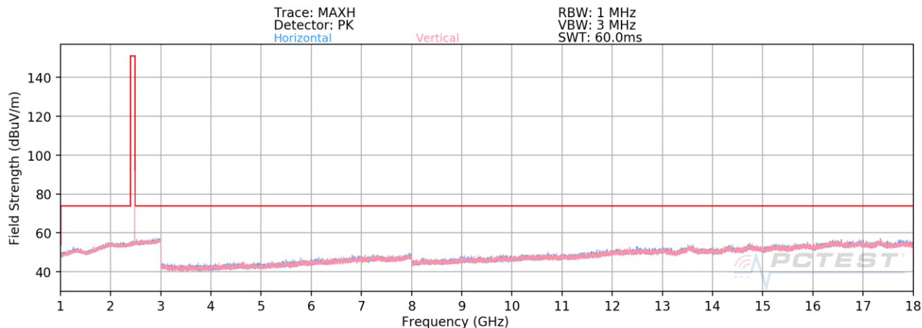
Plot 7-25. Radiated Spurious Emissions Above 1GHz (1Mbps – Ch. 39)
