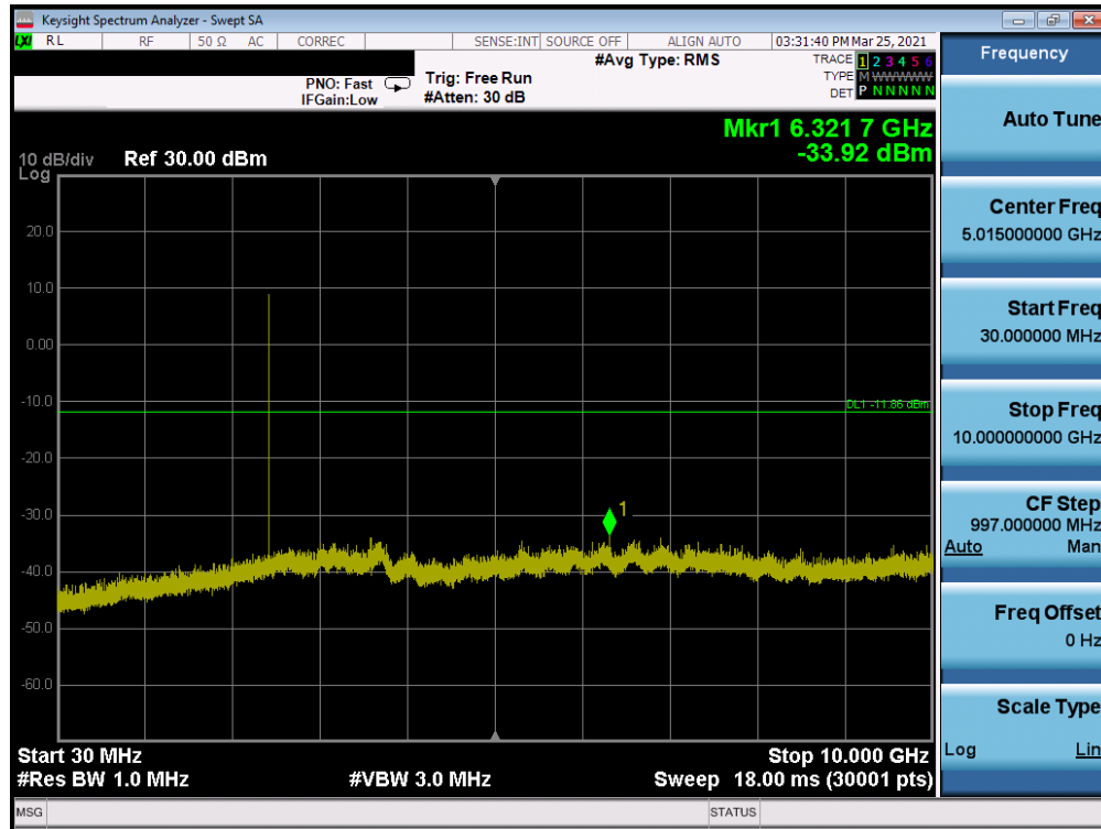
Plot 7-19. Conducted Spurious Emissions (Bluetooth (LE), 1Mbps,- Ch. 19)
