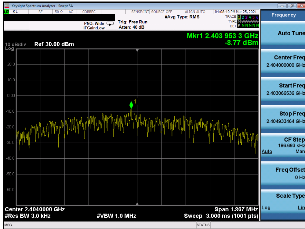
Plot 7-10. Power Spectral Density (Bluetooth (LE), 2Mbps,- Ch. 1)
