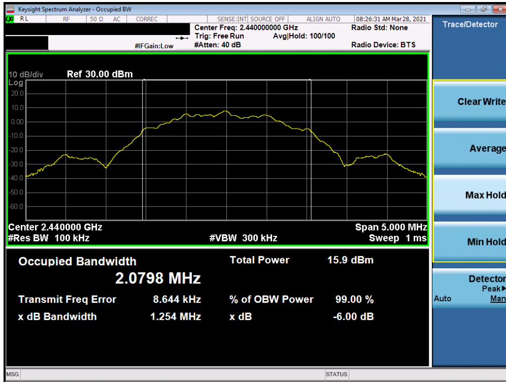
Plot 7-5. 6dB BW & 99% OBW (Bluetooth (LE), 2Mbps,– Ch. 19)
