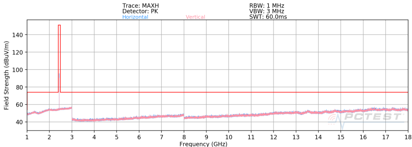
Plot 7-24. Radiated Spurious Emissions Above 1GHz (1Mbps, – Ch. 19)
