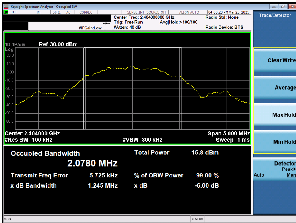
Plot 7-4. 6dB BW & 99% OBW (Bluetooth (LE), 2Mbps,- Ch. 1)
