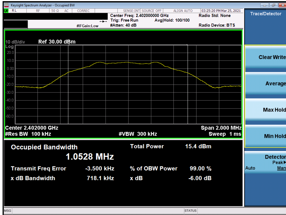
Plot 7-1. 6dB BW & 99% OBW (Bluetooth (LE), 1Mbps, – Ch. 0)
