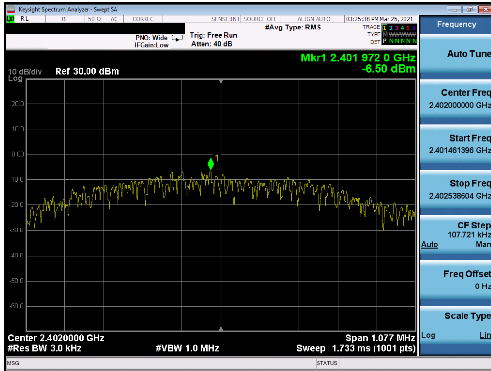
Plot 7-7. Power Spectral Density (Bluetooth (LE), 1Mbps,- Ch. 0)
