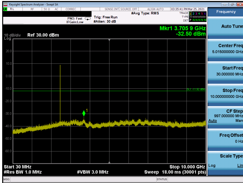
Plot 7-21. Conducted Spurious Emissions (Bluetooth (LE), 1Mbps,– Ch. 39)
