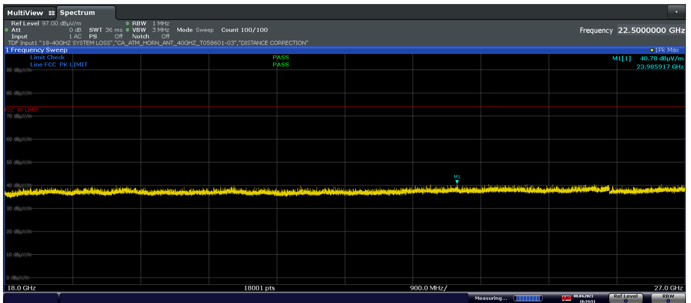
Plot 7-27. Radiated Spurious Emissions Above 18GHz (1Mbps, – Ch.19, Pol. V)
