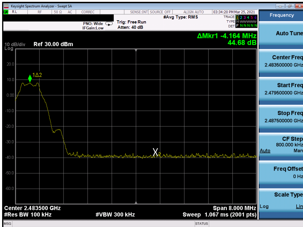
Plot 7-14. Conducted Band Edge (Bluetooth (LE), 1Mbps,- Ch. 39)
