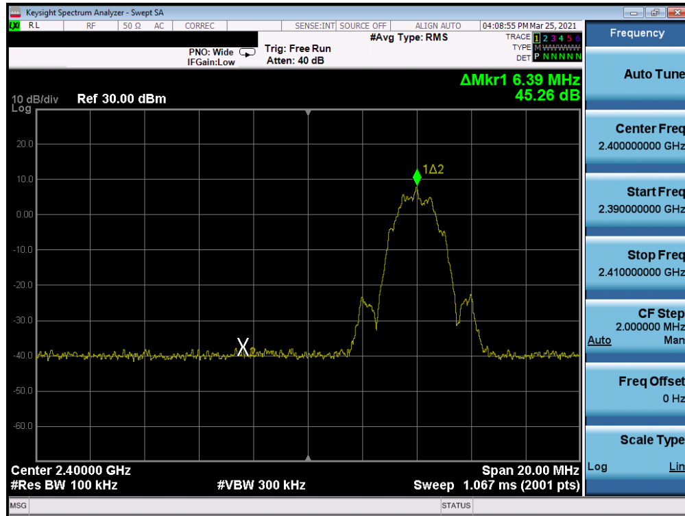
Plot 7-15. Conducted Band Edge (Bluetooth (LE), 2Mbps,- Ch. 1)
