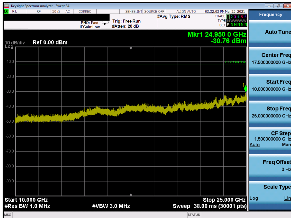
Plot 7-20. Conducted Spurious Emissions (Bluetooth (LE), 1Mbps,- Ch. 19)
