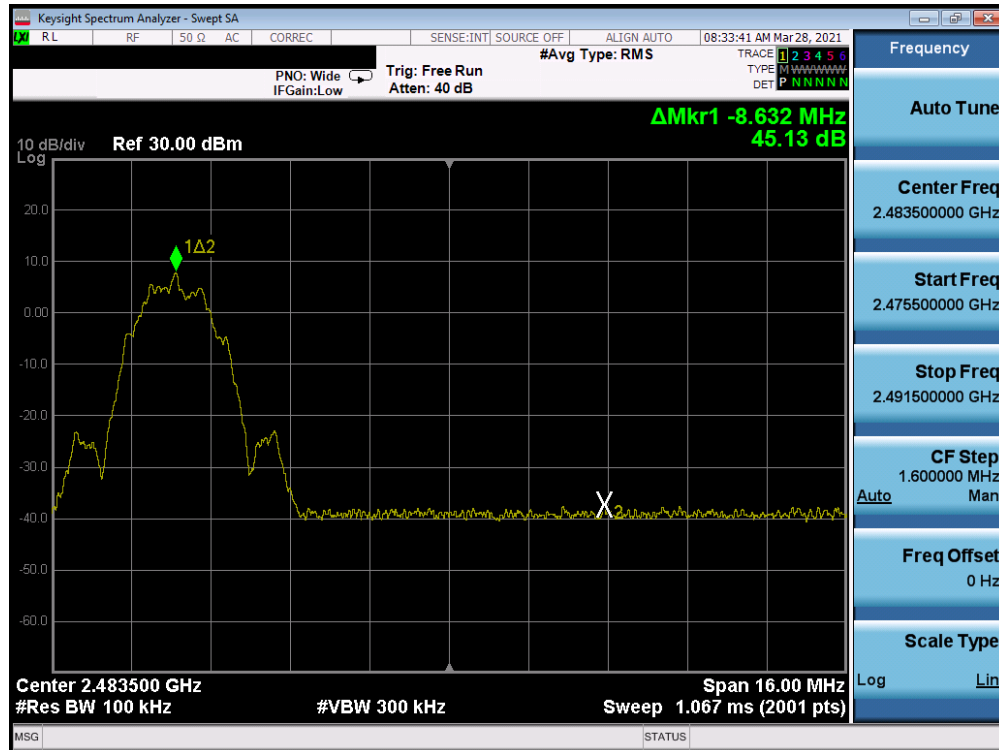
Plot 7-16. Conducted Band Edge (Bluetooth (LE), 2Mbps,- Ch. 38)
