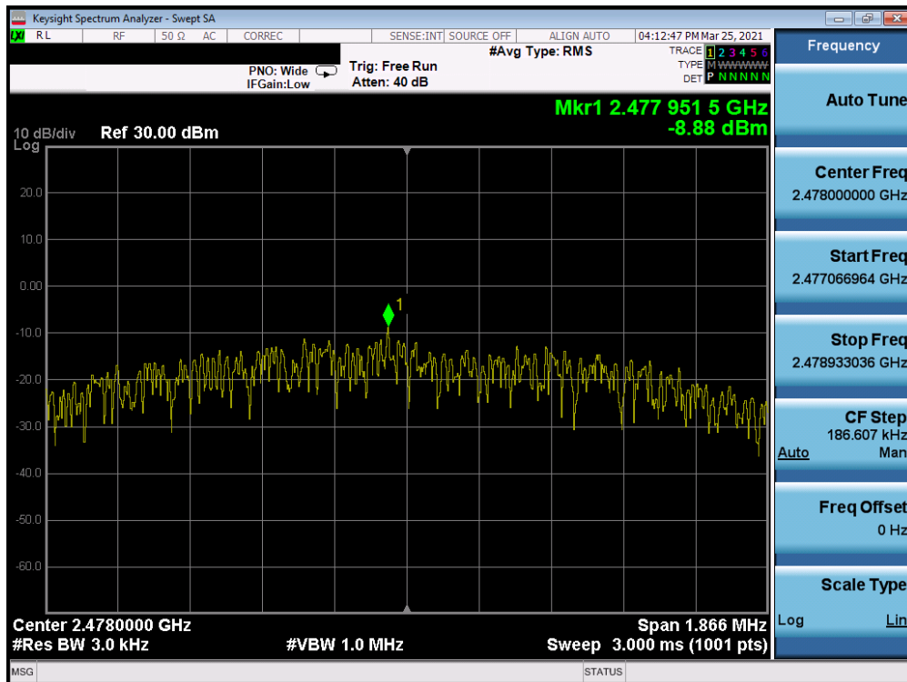
Plot 7-12. Power Spectral Density (Bluetooth (LE), 2Mbps,- Ch. 38)
