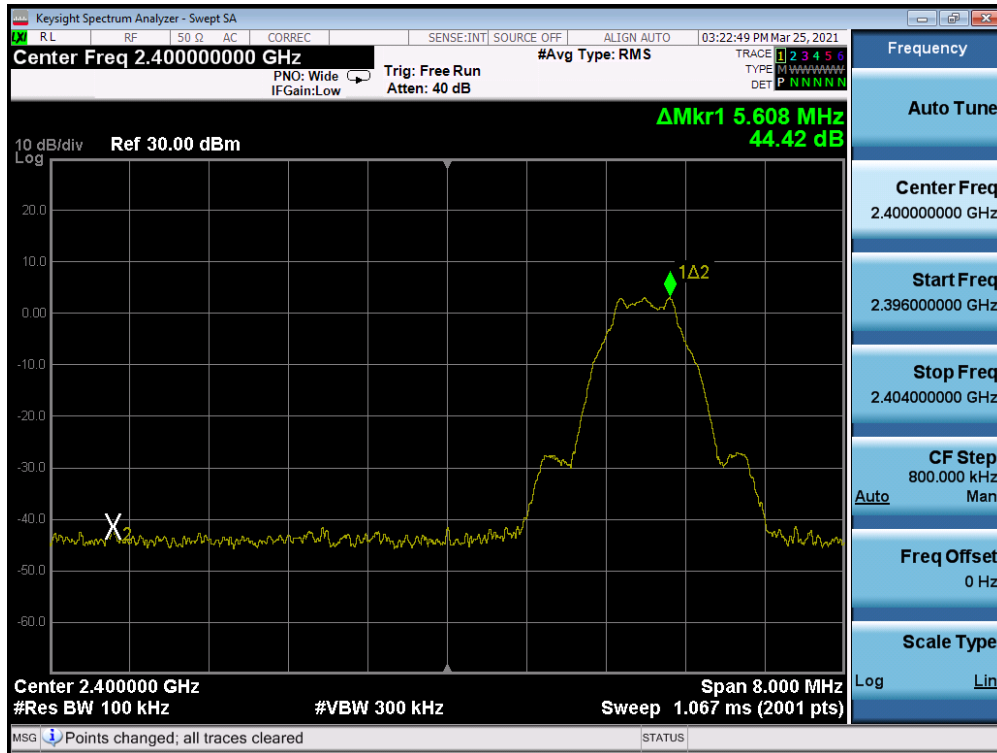
Plot 7-13. Conducted Band Edge (Bluetooth (LE), 1Mbps,- Ch. 0)
