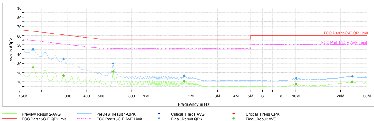
Plot 7-33. AC Line Conducted Plot with Bluetooth LE (1Mbps, – Ch.19, L1, with Laptop and Charging Case)
