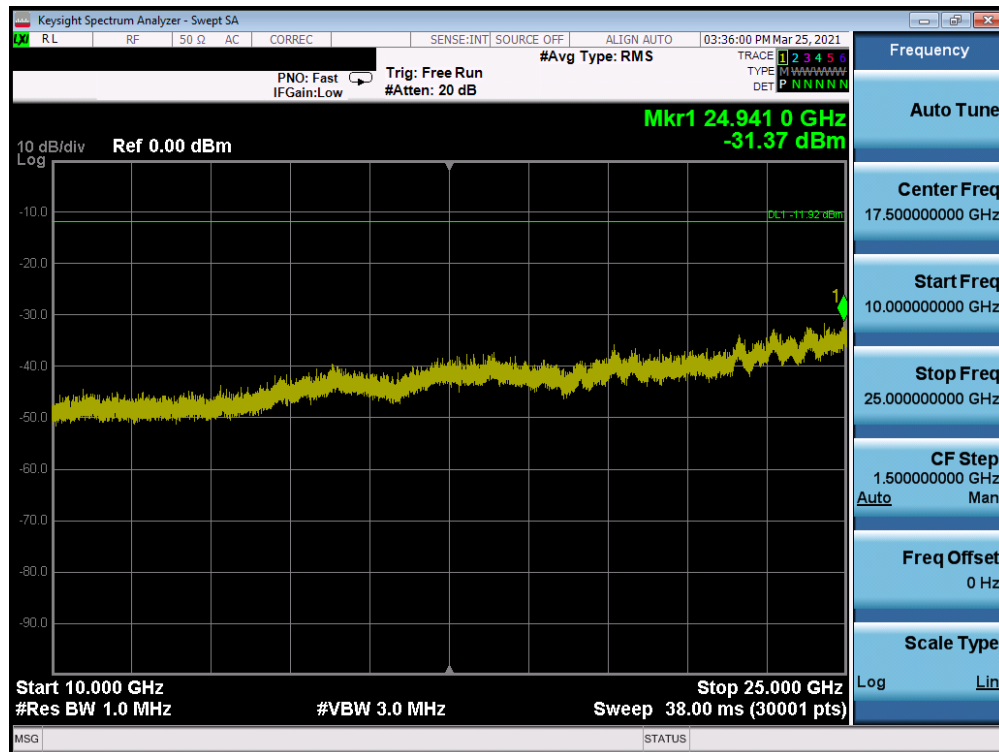
Plot 7-22. Conducted Spurious Emissions (Bluetooth (LE), 1Mbps,– Ch. 39)
