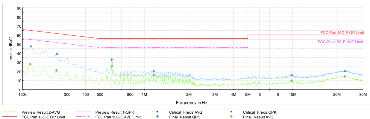
Plot 7-34. AC Line Conducted Plot with Bluetooth LE (1Mbps, – Ch.19, N, with Laptop and Charging Case)
