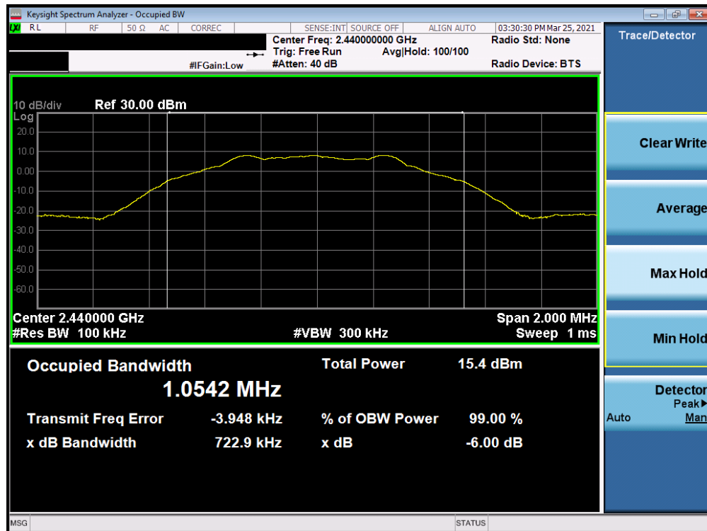
Plot 7-2. 6dB BW & 99% OBW (Bluetooth (LE), 1Mbps, – Ch. 19)
