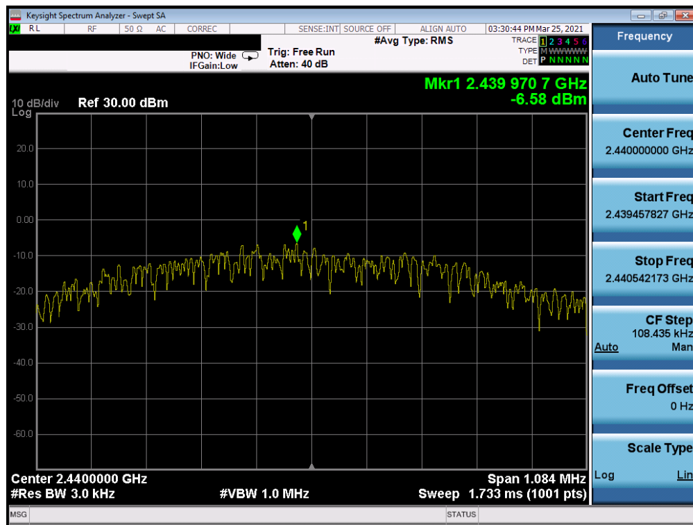
Plot 7-8. Power Spectral Density (Bluetooth (LE), 1Mbps,- Ch. 19)
