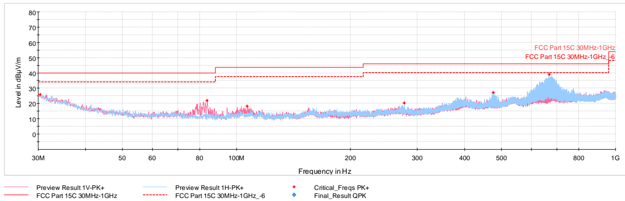
Plot 7-32. Radiated Spurious Emissions Below 1GHz (1Mbps, Ch.19, Pol. H&V, with Laptop and Charging Case)
