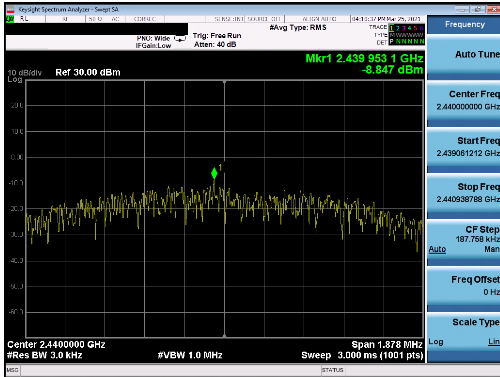
Plot 7-11. Power Spectral Density (Bluetooth (LE), 2Mbps,- Ch. 19)
