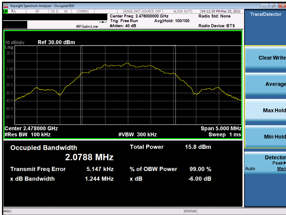
Plot 7-6. 6dB BW & 99% OBW (Bluetooth (LE), 2Mbps,– Ch. 38)
