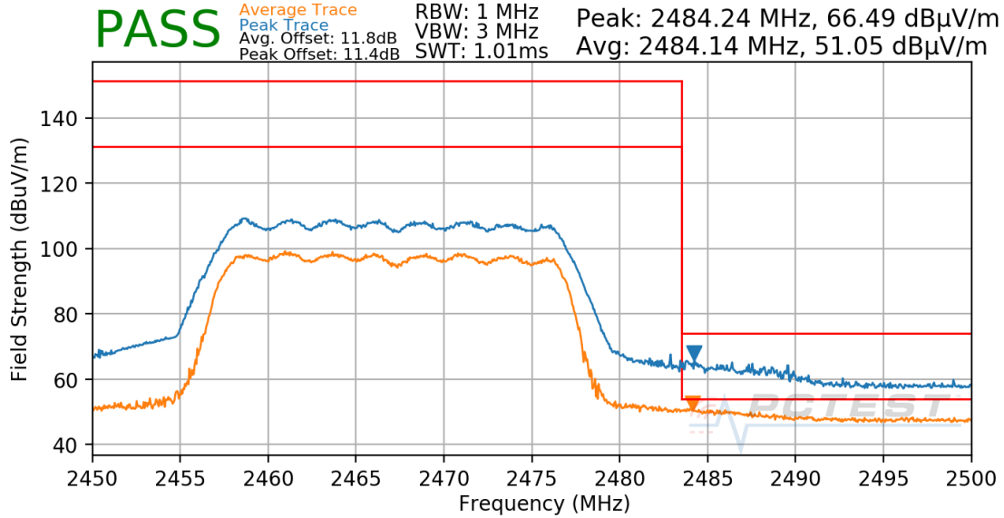
Plot 7-120. Radiated Restricted Upper Band Edge Measurement CDD
