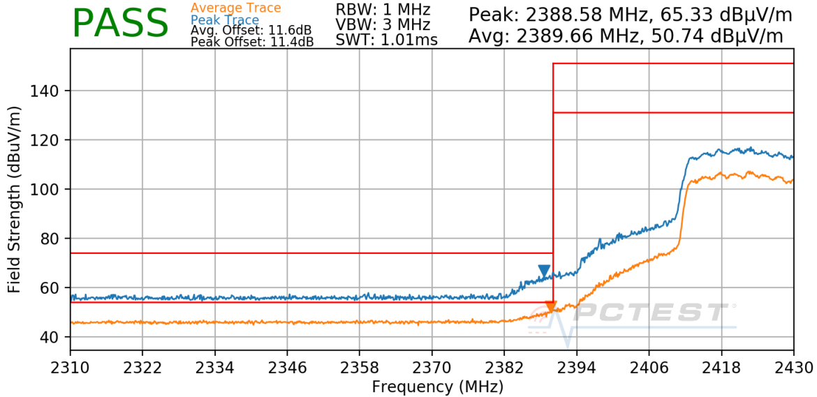
Plot 7-104. Radiated Restricted Lower Band Edge Measurement CDD
