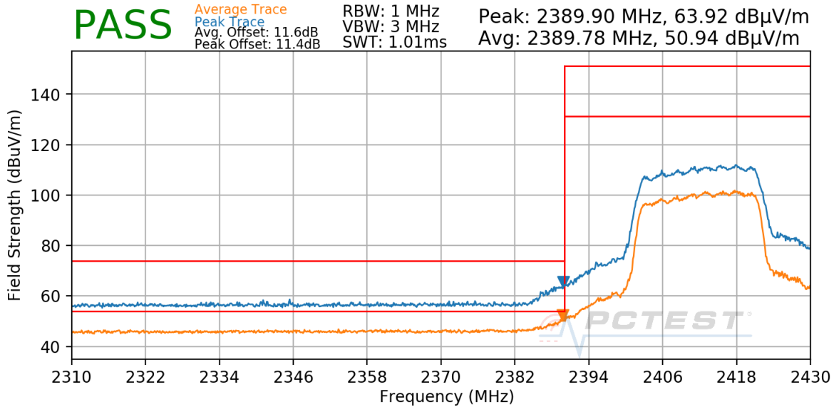
Plot 7-98. Radiated Restricted Lower Band Edge Measurement CDD
