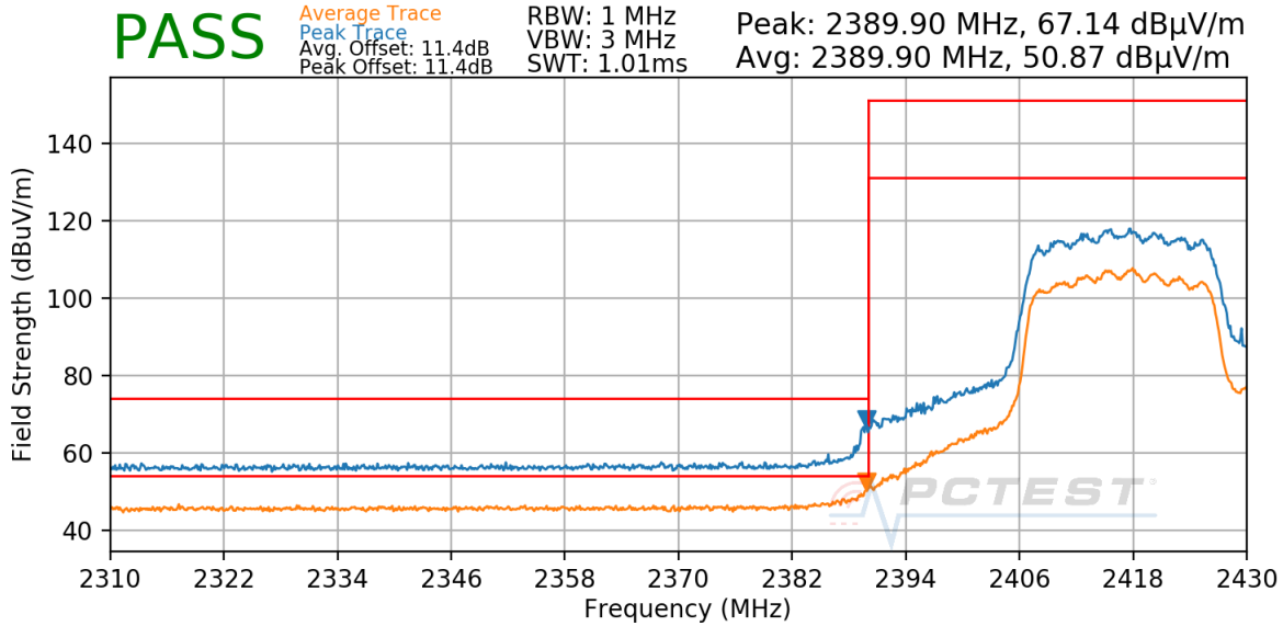
Plot 7-100. Radiated Restricted Lower Band Edge Measurement CDD
