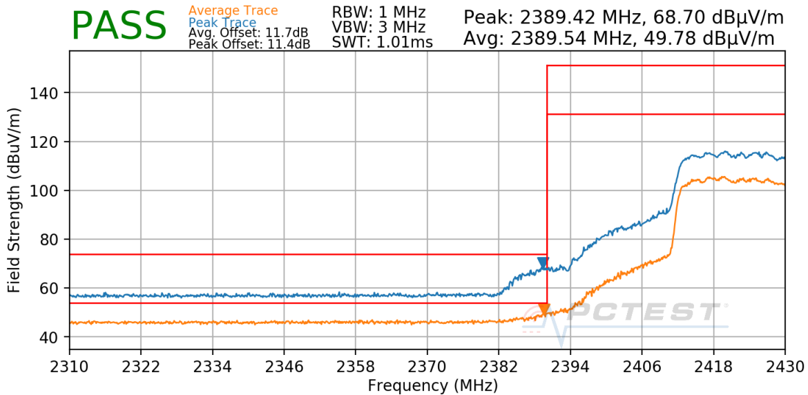
Plot 7-105. Radiated Restricted Lower Band Edge Measurement CDD
