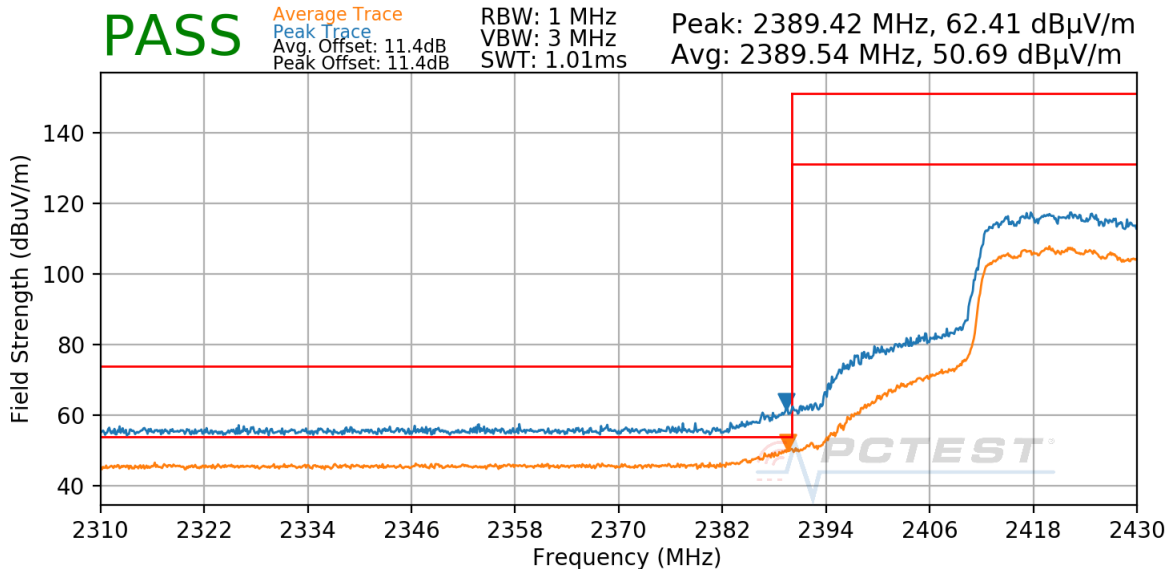
Plot 7-103. Radiated Restricted Lower Band Edge Measurement CDD
