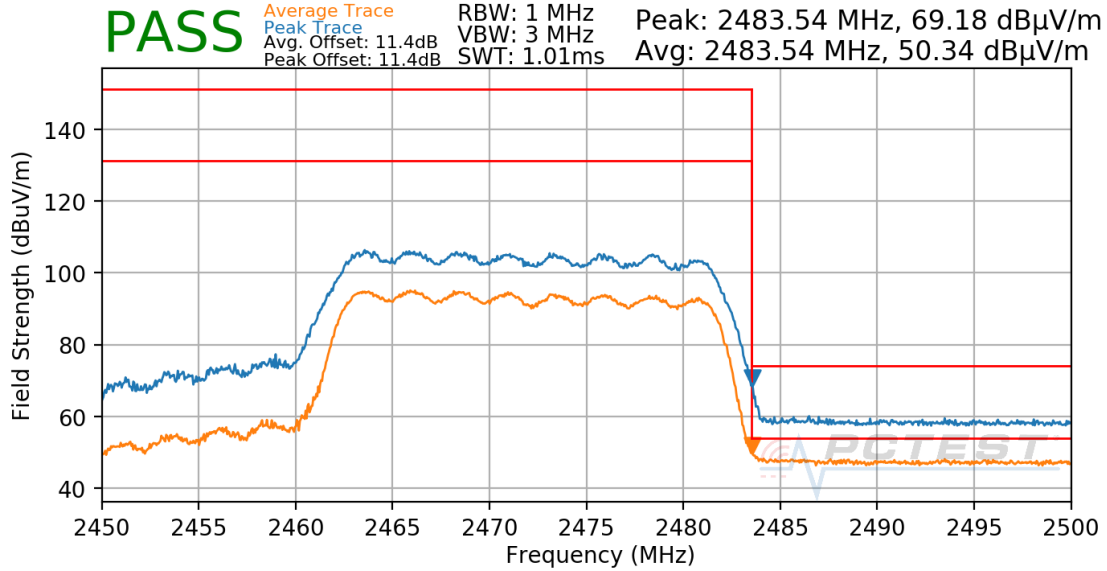
Plot 7-94. Radiated Restricted Upper Band Edge Measurement CDD
