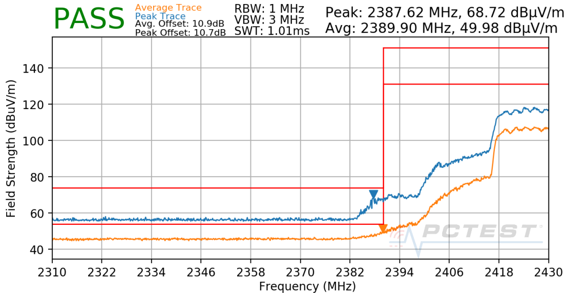
Plot 7-107. Radiated Restricted Lower Band Edge Measurement CDD
