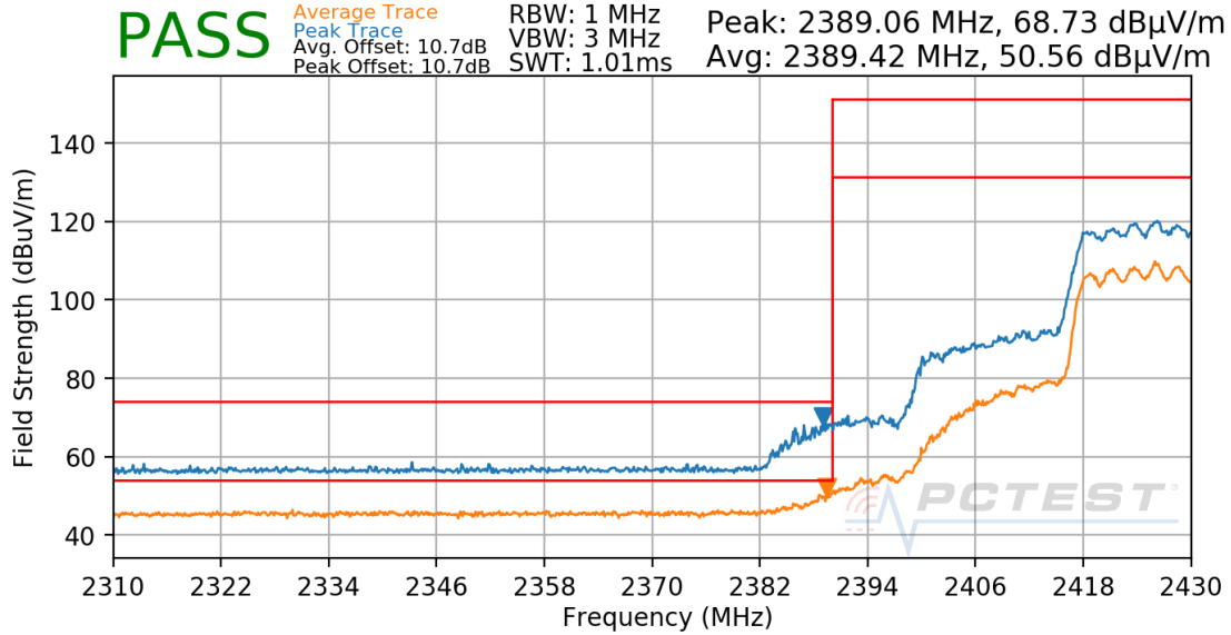
Plot 7-106. Radiated Restricted Lower Band Edge Measurement CDD
