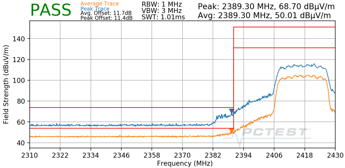
Plot 7-102. Radiated Restricted Lower Band Edge Measurement CDD
