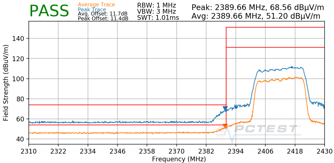
Plot 7-99. Radiated Restricted Lower Band Edge Measurement CDD
