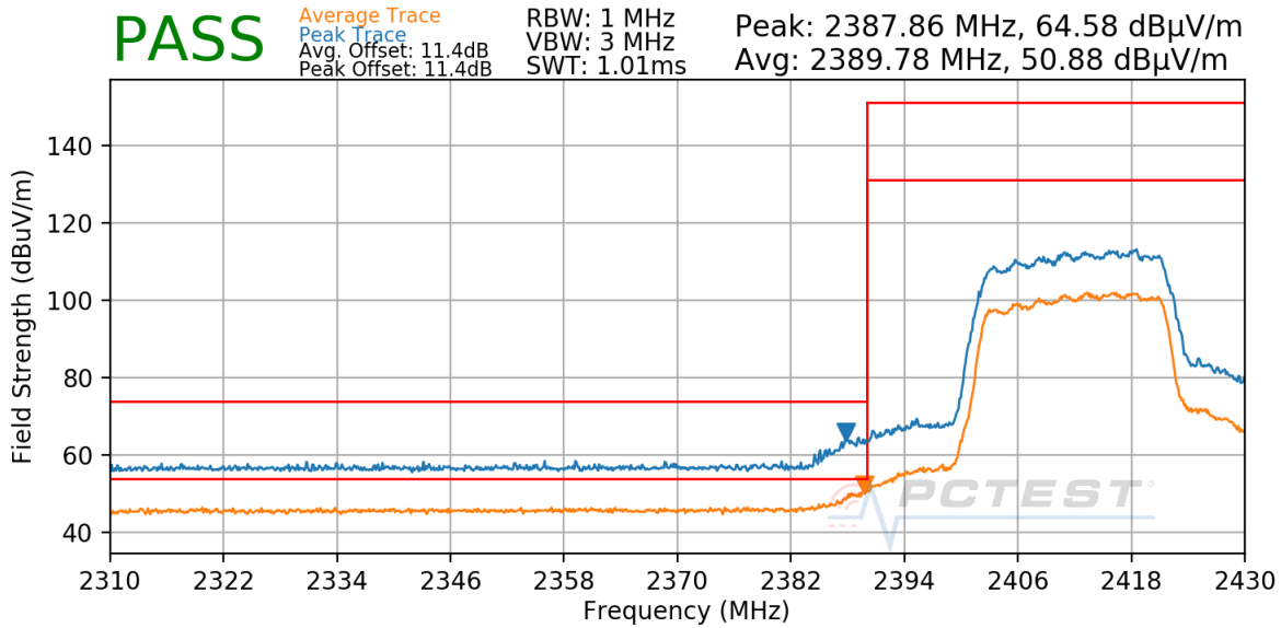
Plot 7-97. Radiated Restricted Lower Band Edge Measurement CDD
