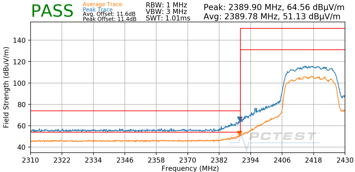
Plot 7-101. Radiated Restricted Lower Band Edge Measurement CDD
