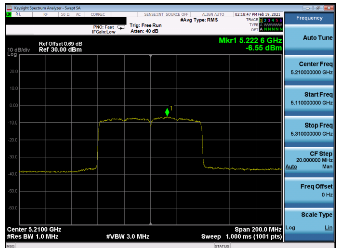
Plot 7-491. ISED PSD SDM Antenna 5b (80MHz BW 11ax (SU) – Ch.42, MCS3)
