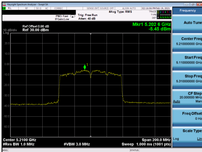
Plot 7-489. ISED PSD SDM Antenna 5b (80MHz BW 11ac – Ch.42, MCS3)
