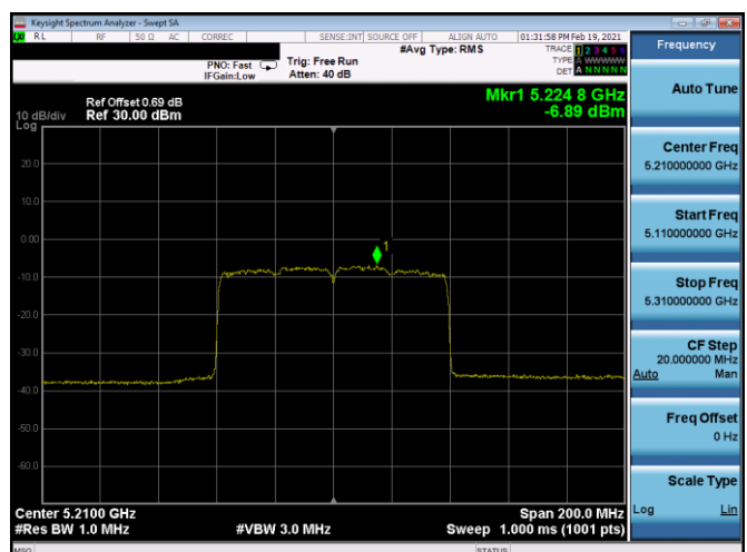
Plot 7-492. ISED PSD SDM Antenna 4b (80MHz BW 11ax (SU) – Ch.42, MCS3)
