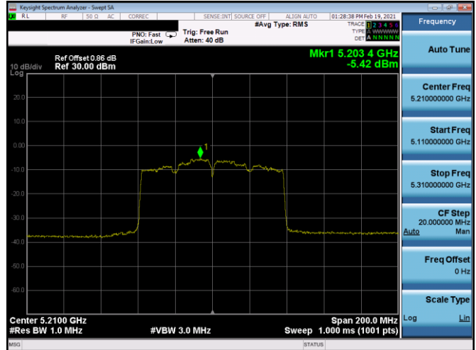
Plot 7-490. ISED PSD SDM Antenna 4b (80MHz BW 11ac – Ch.42, MCS3)
