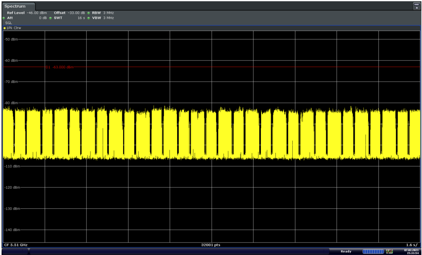
Figure 9-9. 5510MHz - Channel Loading - Mode 2 (40MHz)
