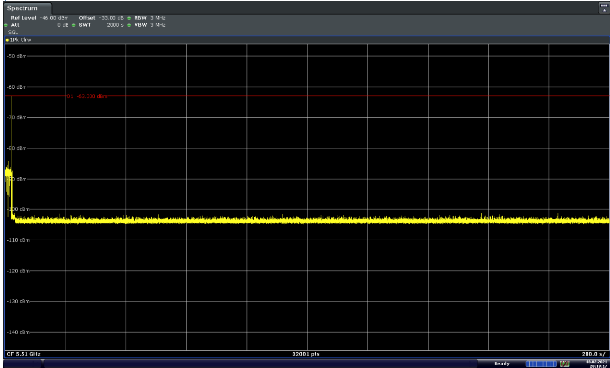
Figure 9-44. 5510MHz - Non-Occupancy Period (30 Minutes) - Mode 3 (40MHz)
