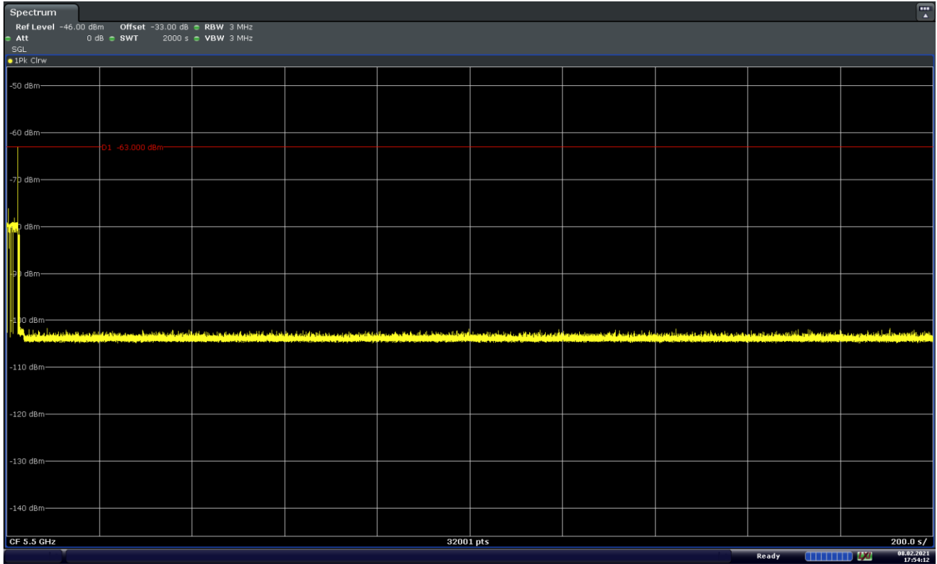
Figure 9-46. 5500MHz - Non-Occupancy Period (30 Minutes) - Mode 4 (20MHz)
