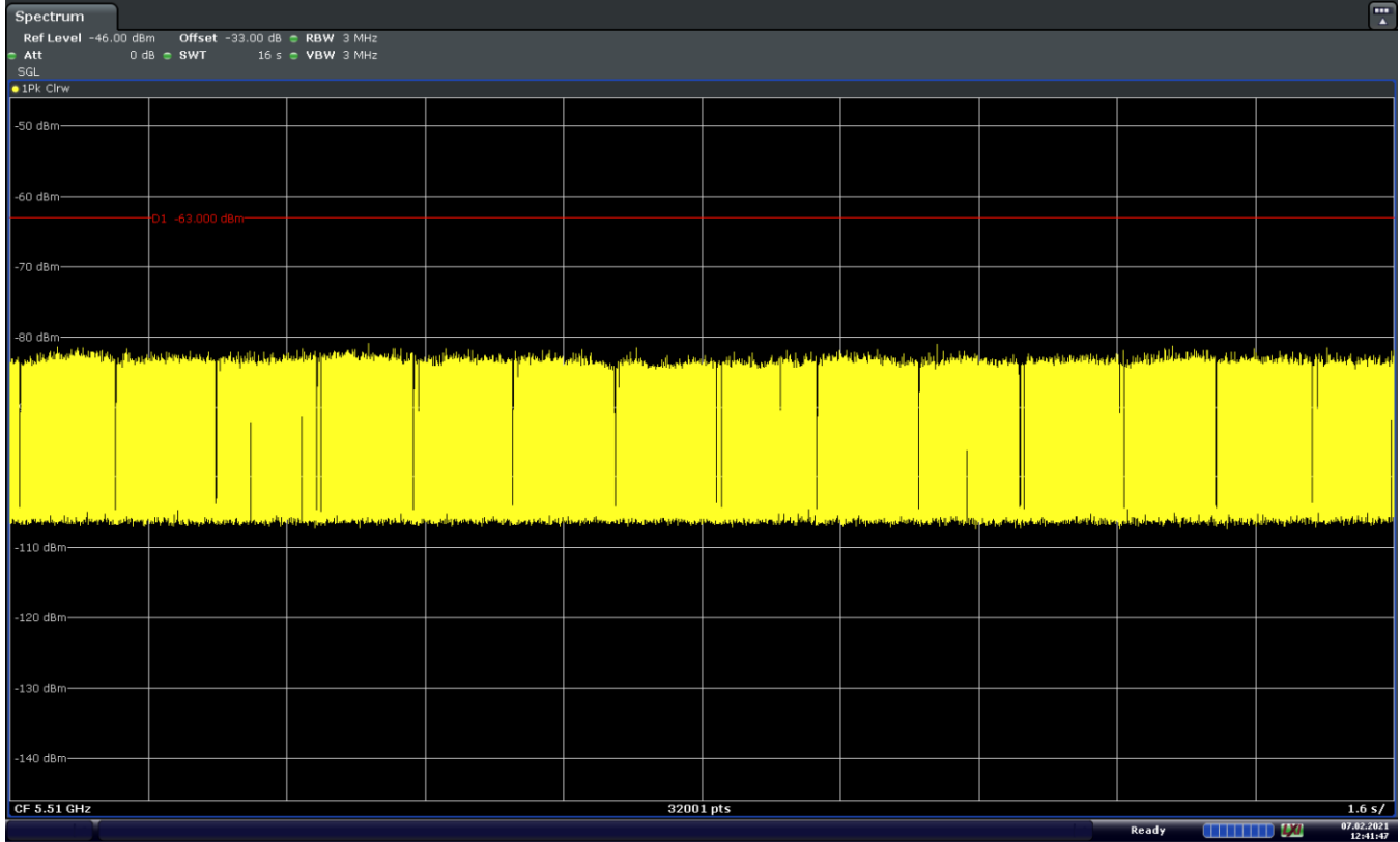
Figure 9-3. 5510MHz - Channel Loading - Mode 1 (40MHz)
