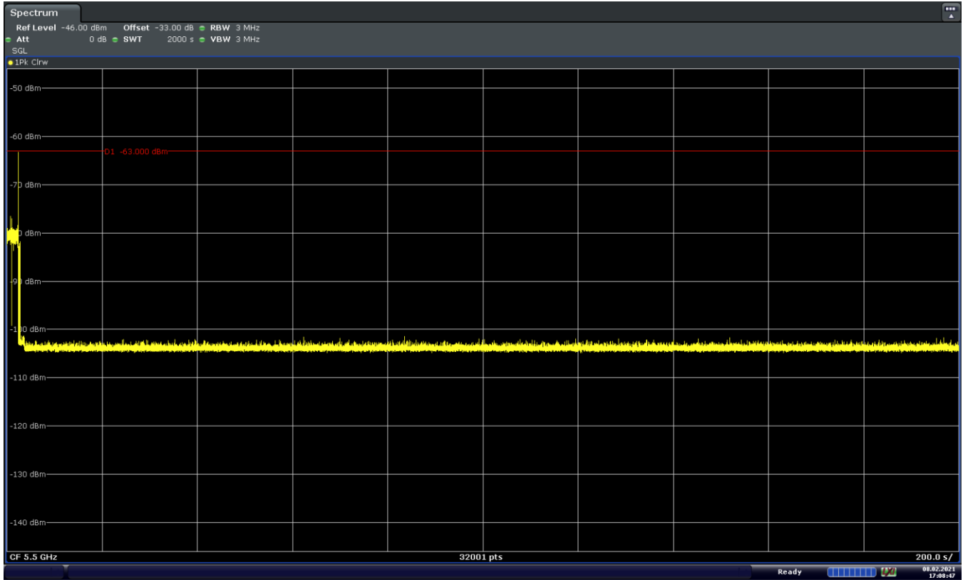
Figure 9-43. 5500MHz - Non-Occupancy Period (30 Minutes) - Mode 3 (20MHz)
