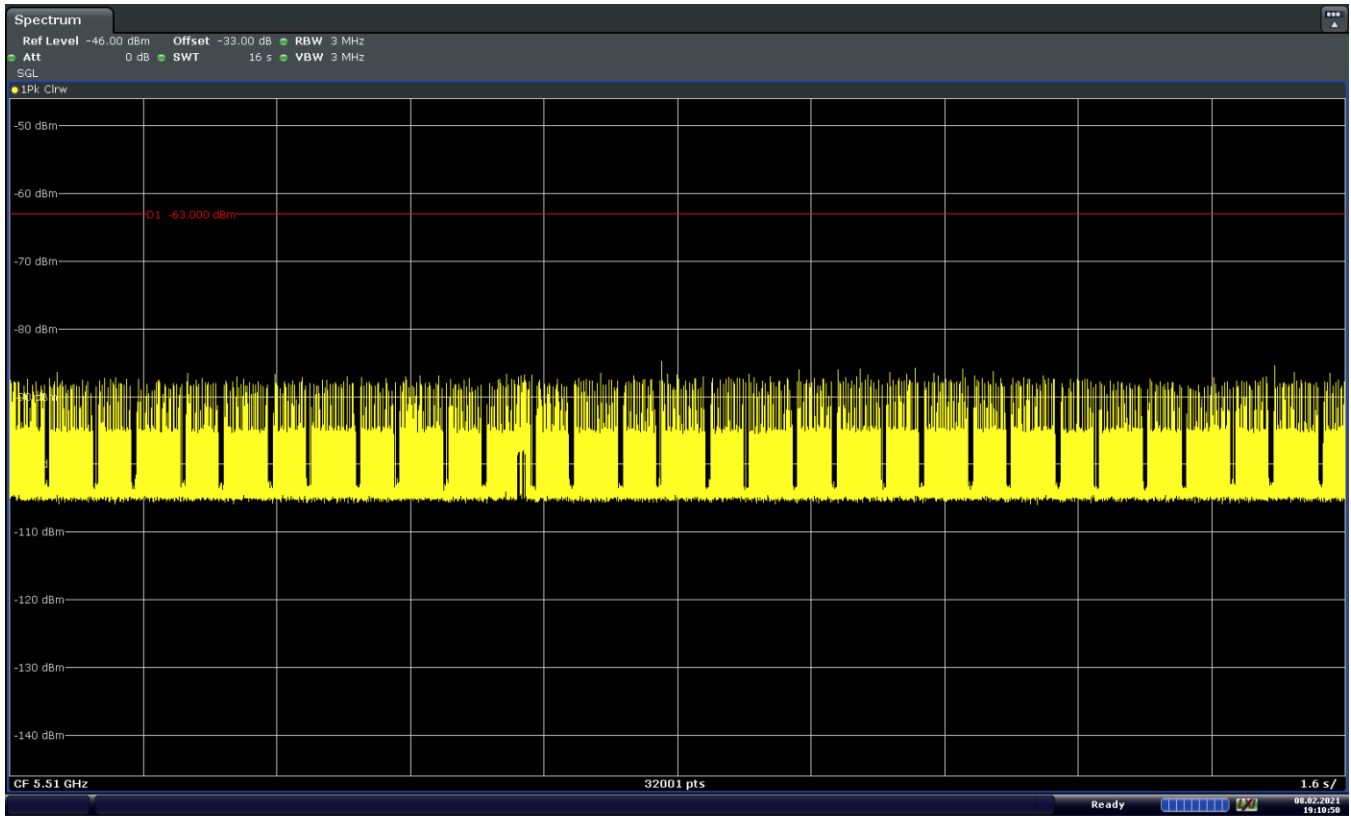
Figure 9-15. 5510MHz - Channel Loading - Mode 3 (40MHz)
