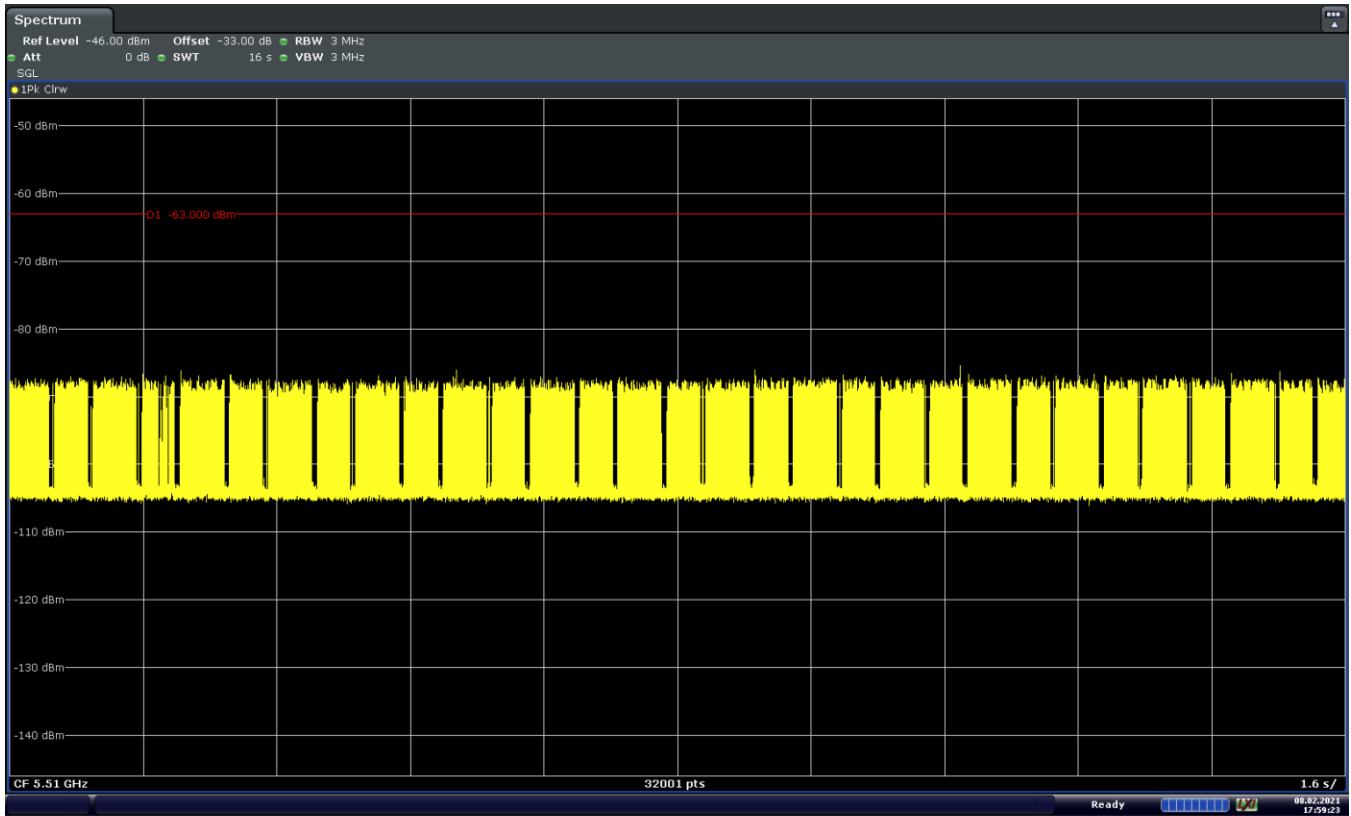
Figure 9-21. 5510MHz - Channel Loading - Mode 4 (40MHz)
