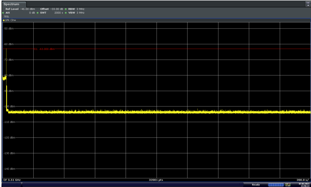
Figure 9-38. 5510MHz - Non-Occupancy Period (30 Minutes) - Mode 1 (40MHz)
