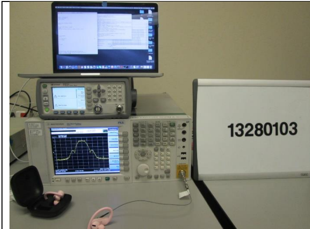
RF CONDUCTED
