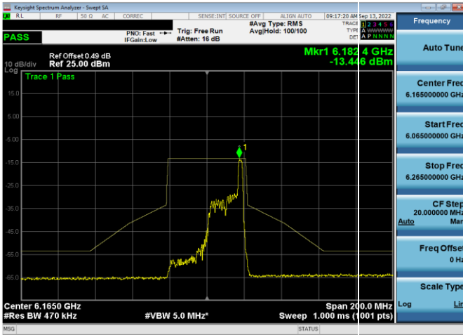
Plot 7-391. In-Band Emission Plot Antenna 5b (40MHz 802.11ax RU26 (UNII Band 5) – Ch. 43)
