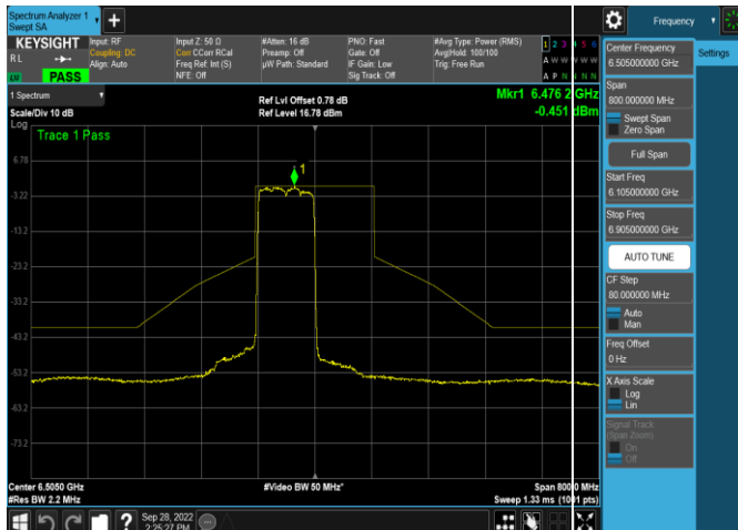
Plot 7-416. In-Band Emission Plot Antenna 5b (160MHz 802.11ax RU996x2 (UNII Band 6) – Ch. 111)
