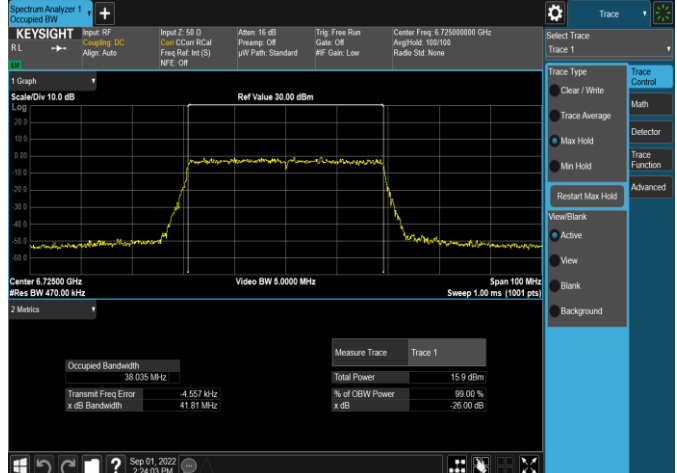
Plot 7-40. 26dB & 99% Bandwidth Plot Antenna 5b (40MHz 802.11ax RU48 (UNII Band 7) – Ch. 155)
