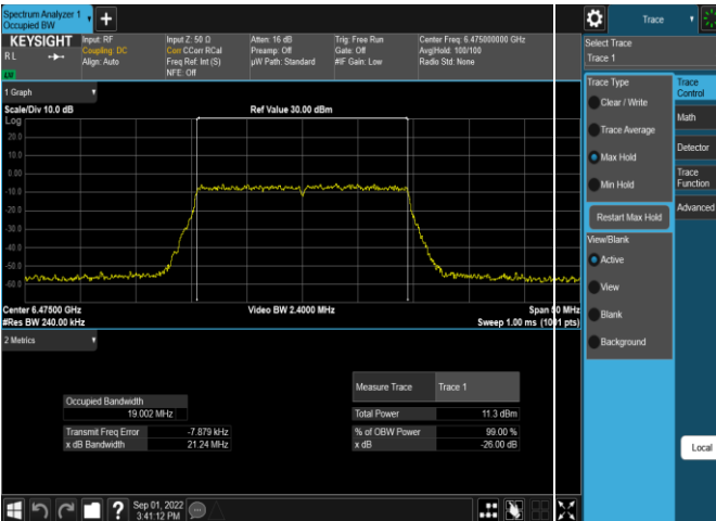
Plot 7-20. 26dB & 99% Bandwidth Plot Antenna 5b (20MHz 802.11ax RU242 (UNII Band 6) – Ch. 105)
