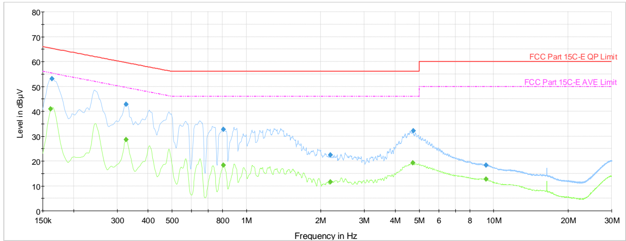
Plot 7-752. AC Line Conducted Plot with 802.11ax SDM – Ch.1 (L1), with AC/DC adapter
