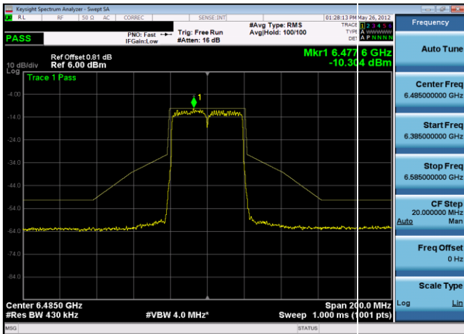
Plot 7-388. In-Band Emission Plot Antenna 5b (40MHz 802.11ax (UNII Band 6) – Ch. 107, MCS11)
