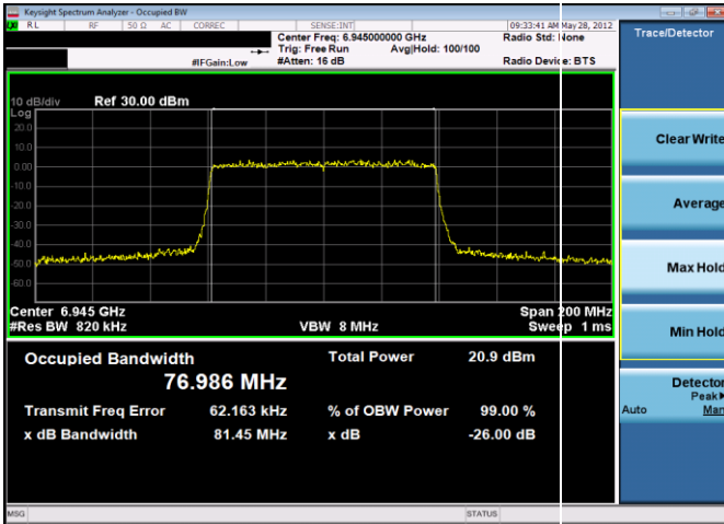
Plot 7-59. 26dB & 99% Bandwidth Plot Antenna 5b (80MHz 802.11ax (UNII Band 8) – Ch. 199, MCS11)
