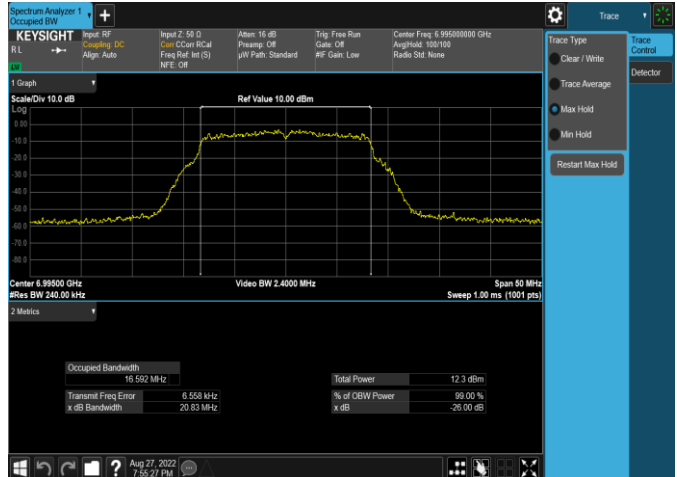
Plot 7-76. 26dB & 99% Bandwidth Plot Antenna 4a (20MHz 802.11a (UNII Band 8) – Ch. 209, MCS2)
