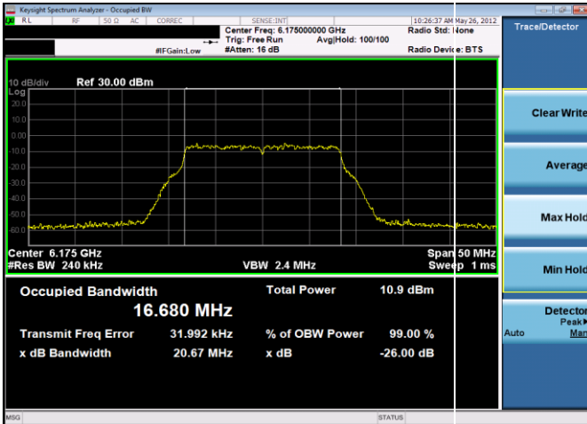
Plot 7-101. 26dB & 99% Bandwidth Plot Antenna 4a (20MHz 802.11a (UNII Band 5) – Ch. 45, MCS11)
