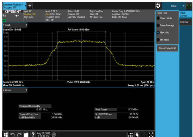
Plot 7-66. 26dB & 99% Bandwidth Plot Antenna 4a (20MHz 802.11a (UNII Band 6) – Ch. 105, MCS2)
