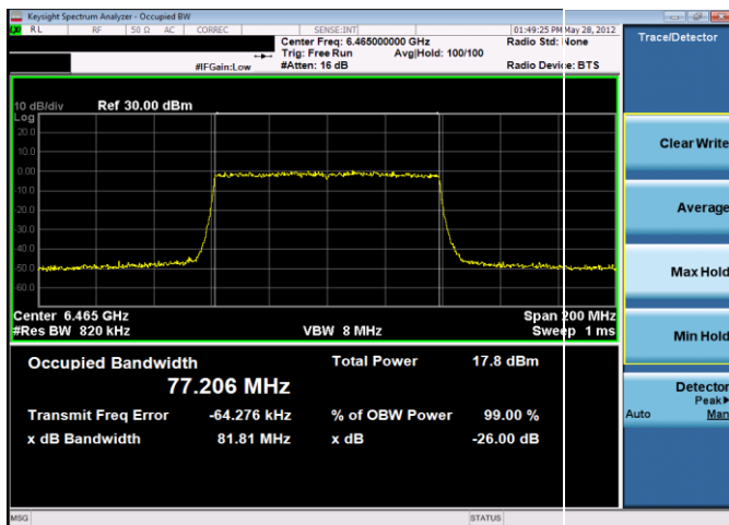
Plot 7-69. 26dB & 99% Bandwidth Plot Antenna 4a (80MHz 802.11ax (UNII Band 6) – Ch. 103, MCS2)
