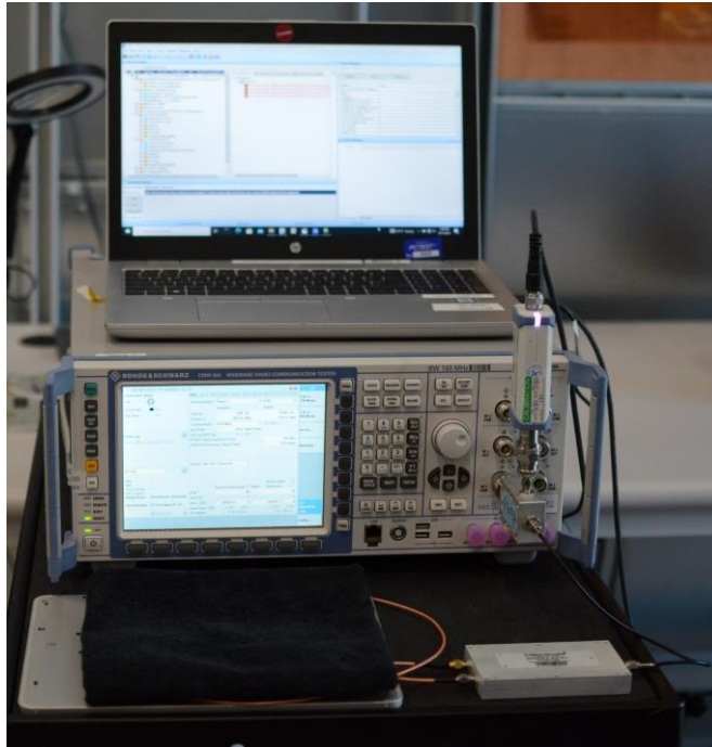
Test Setup Photo 4 – Conducted Test Setup (Figure 5-1b)
