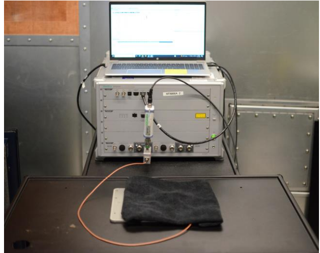
Test Setup Photo 2 – Conducted Test Setup (Figure 5-1a)
