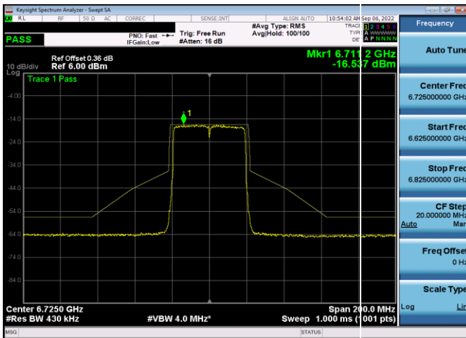
Plot 7-591. In-Band Emission Plot SDM Antenna WF5b (40MHz 802.11ax RU484 (UNII Band 7) – Ch. 155)
