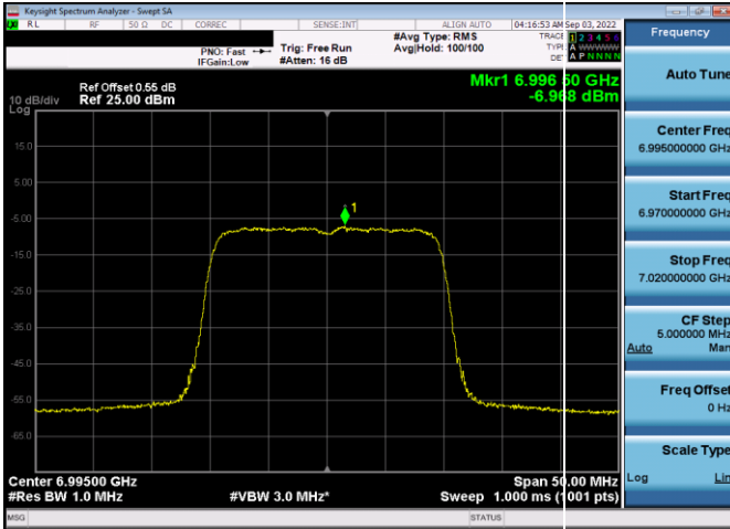
Plot 7-329. Power Spectral Density Plot SDM Antenna WF5t (20MHz 802.11ax (UNII Band 8) – Ch. 209, MCS11)
