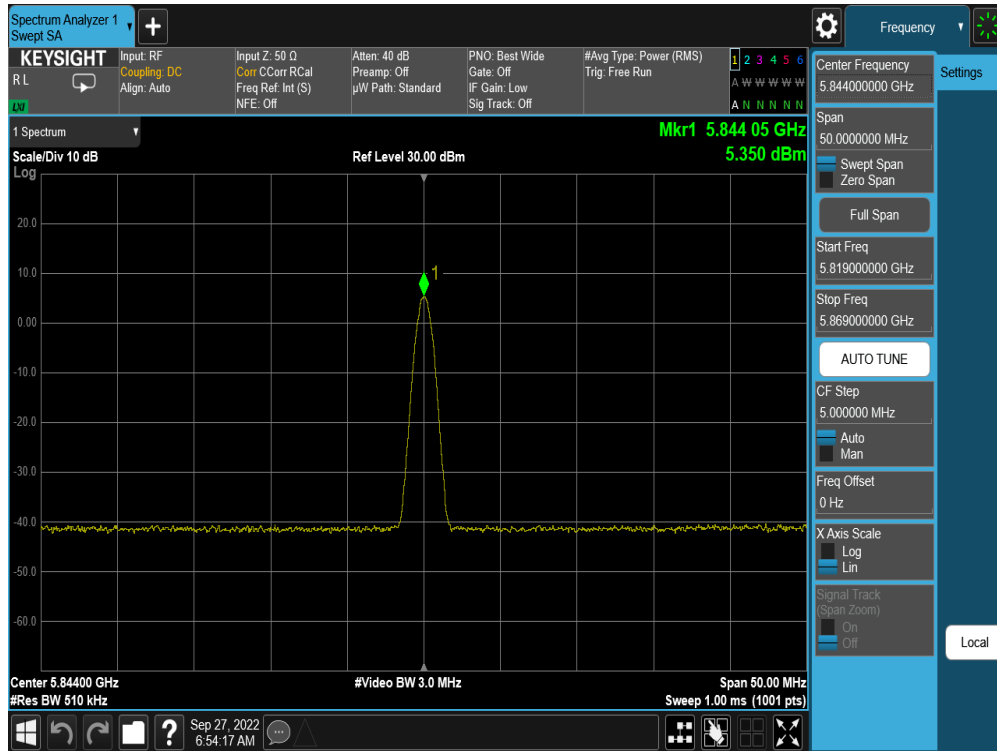
Plot 7-59. PSD TxBF Antenna WF5T (BDR GFSK, iPA – 5844MHz)
