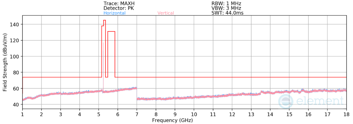
Plot 7-63. RSE 1-18GHz Antenna WF5T (BDR GFSK ePA – 5245MHz)
