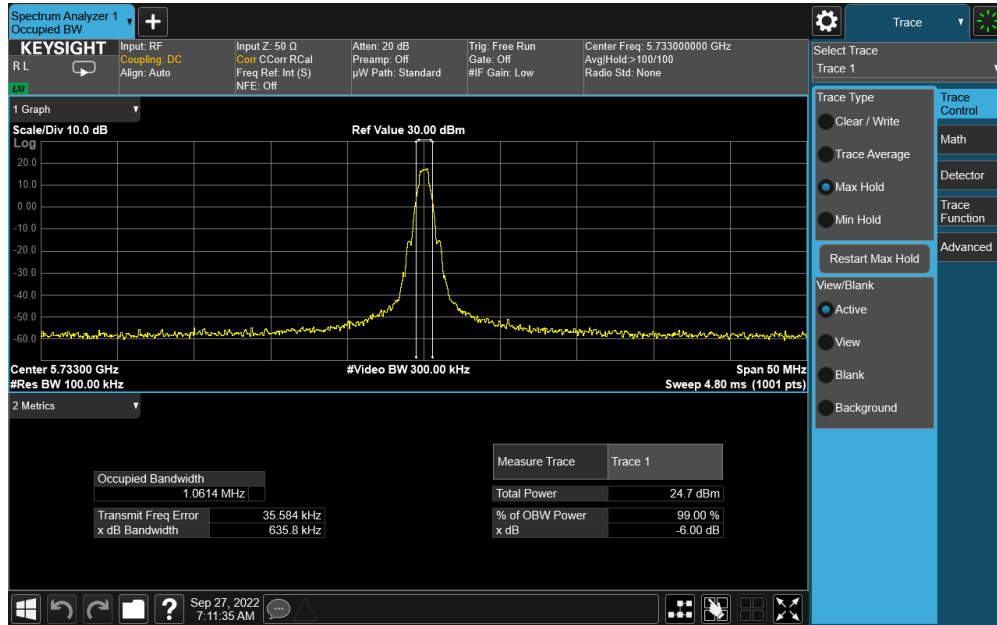
Plot 7-10. 6dB BW & 99% OBW Antenna WF5B (BDR GFSK, ePA – 5733MHz)
