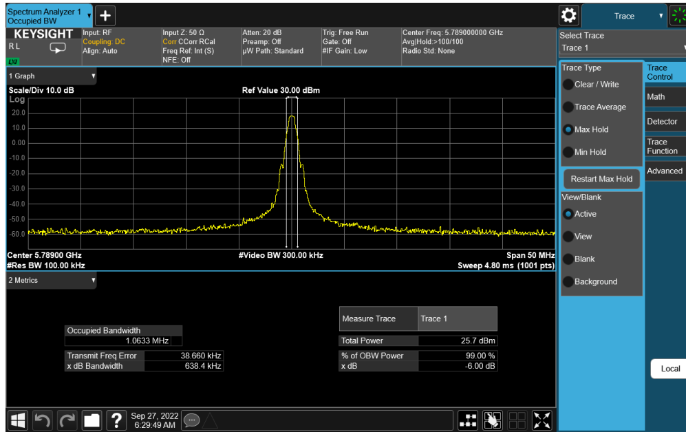
Plot 7-8. 6dB BW & 99% OBW Antenna WF5T (BDR GFSK, ePA – 5789MHz)
