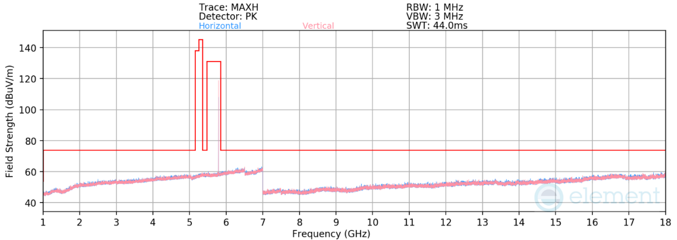
Plot 7-65. RSE 1-18GHz Antenna WF5T (BDR GFSK ePA – 5789MHz)
