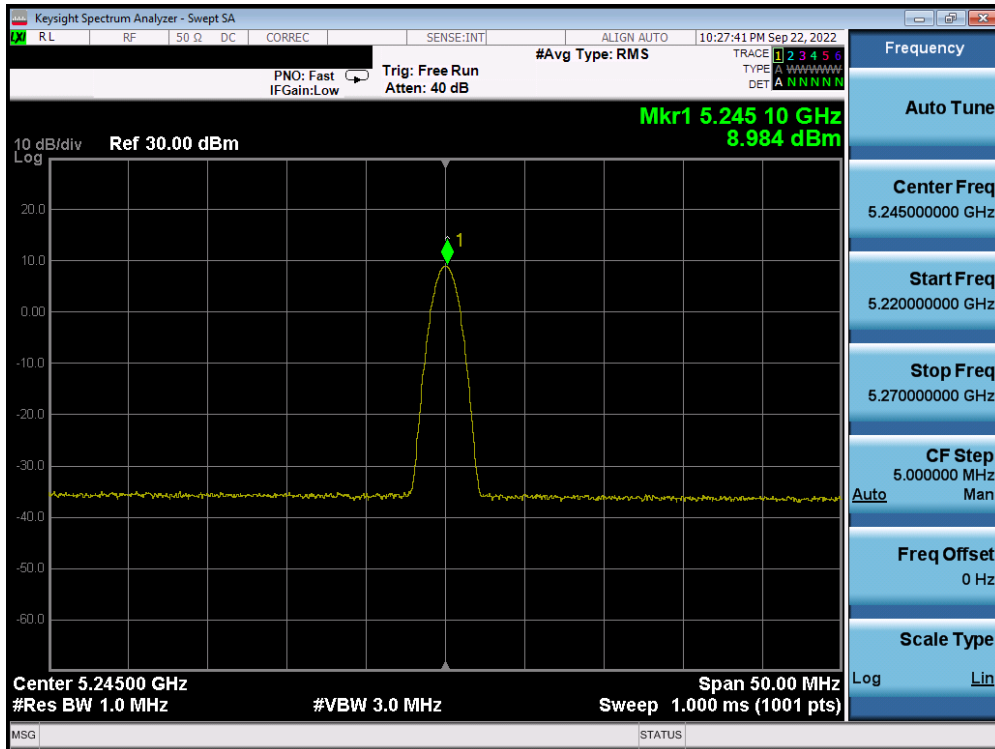
Plot 7-27. PSD Antenna WF5B (BDR GFSK, ePA – 5245MHz)
