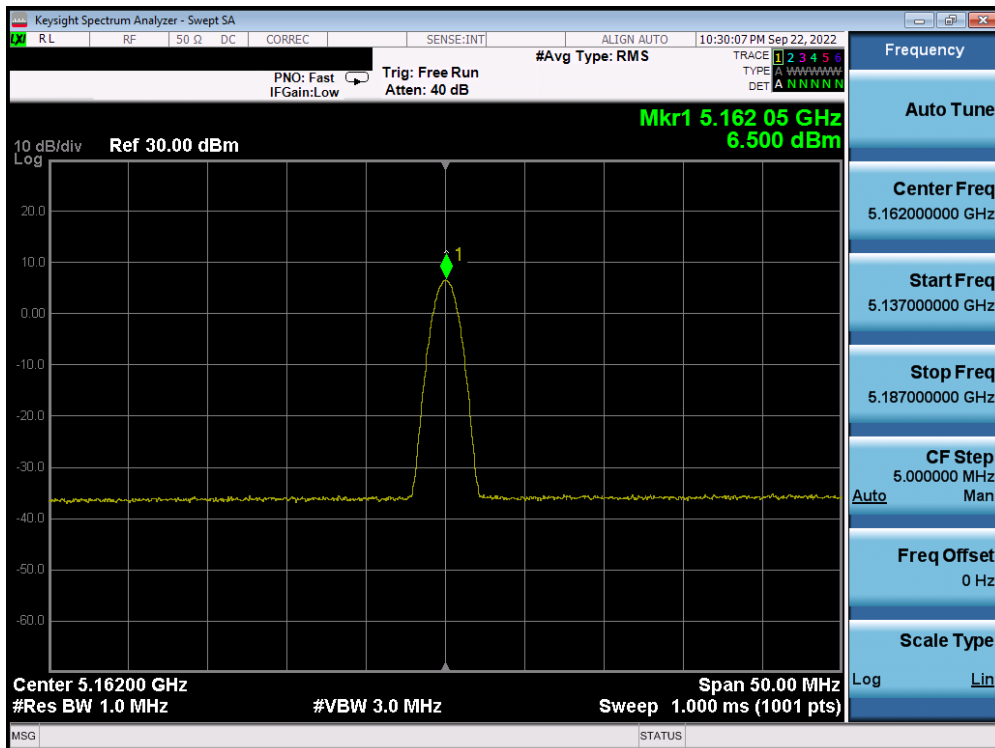
Plot 7-28. PSD Antenna WF5B (BDR GFSK, iPA – 5162MHz)
