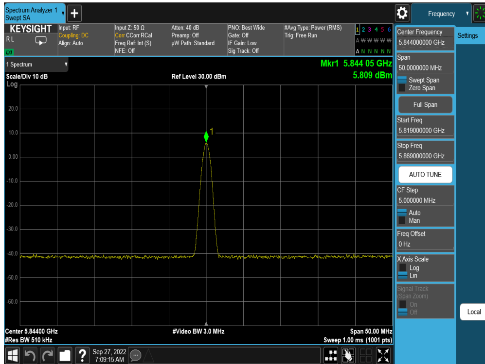
Plot 7-60. PSD TxBF Antenna WF5B (BDR GFSK, iPA – 5844MHz)
