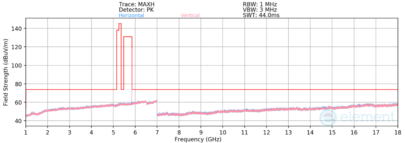
Plot 7-66. RSE 1-18GHz Antenna WF5T (BDR GFSK ePA – 5844MHz)
