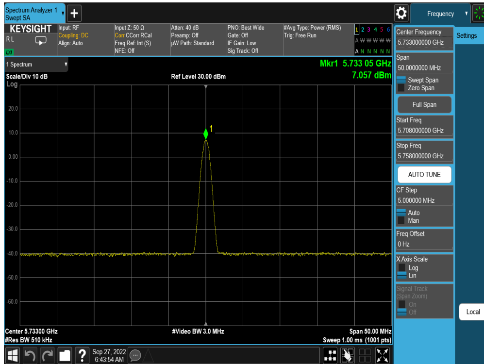
Plot 7-22. PSD Antenna WF5T (BDR GFSK, iPA – 5733MHz)
