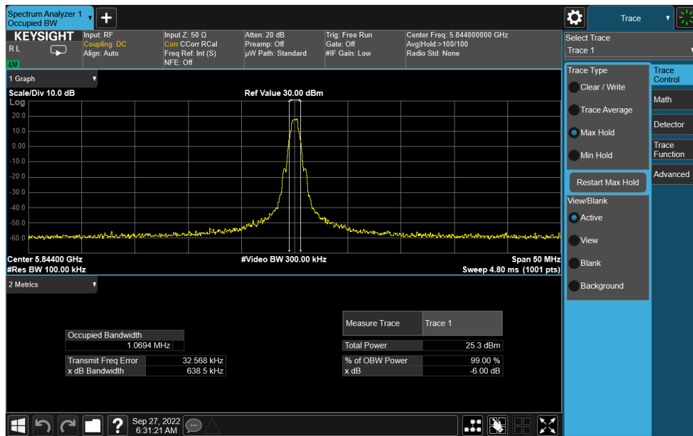
Plot 7-9. 6dB BW & 99% OBW Antenna WF5T (BDR GFSK, ePA – 5844MHz)
