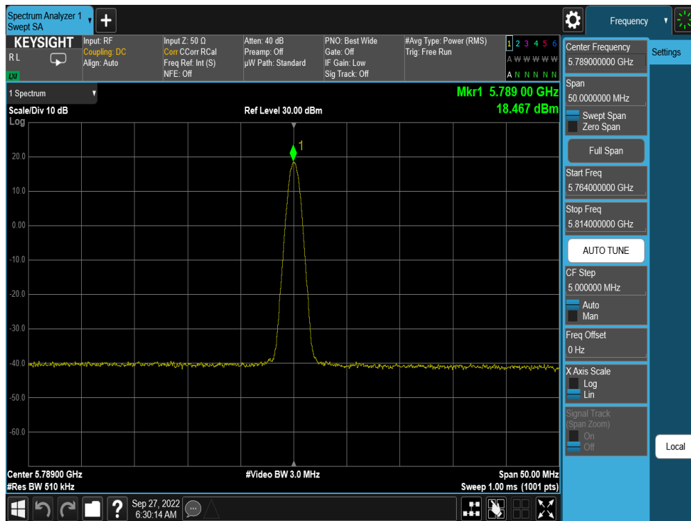
Plot 7-20. PSD Antenna WF5T (BDR GFSK, ePA – 5789MHz)
