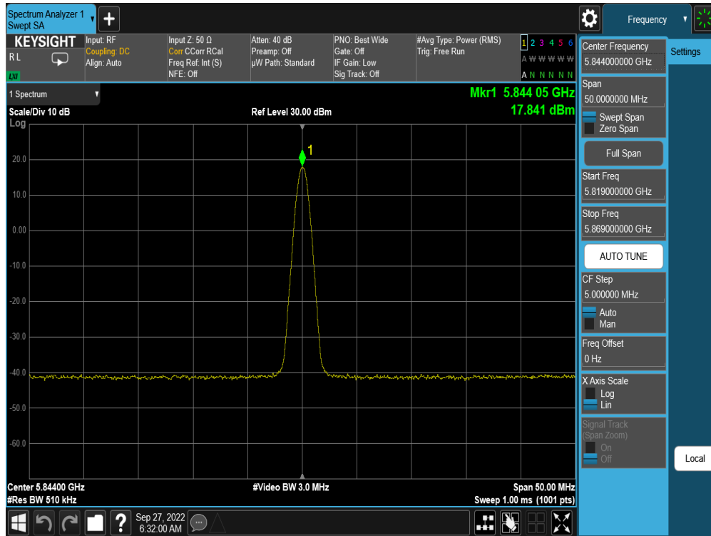
Plot 7-21. PSD Antenna WF5T (BDR GFSK, ePA – 5844MHz)
