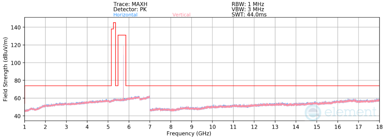
Plot 7-64. RSE 1-18GHz Antenna WF5T (BDR GFSK ePA – 5733MHz)
