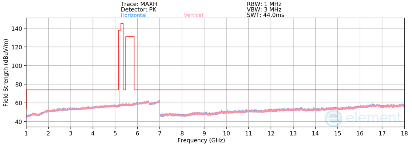
Plot 7-62. RSE 1-18GHz Antenna WF5T (BDR GFSK ePA – 5204MHz)
