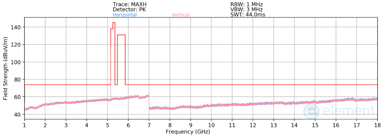
Plot 7-61. RSE 1-18GHz Antenna WF5T (BDR GFSK ePA – 5162MHz)
