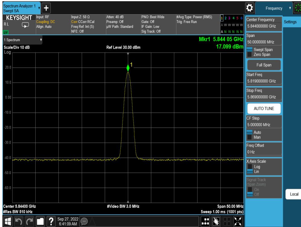
Plot 7-53. PSD TxBF Antenna WF5T (BDR GFSK, ePA – 5844MHz)
