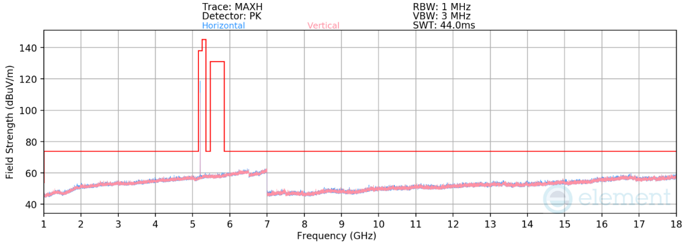
Plot 7-68. RSE 1-18GHz Antenna WF5B (BDR GFSK ePA – 5204MHz)
