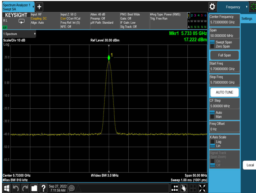
Plot 7-31. PSD Antenna WF5B (BDR GFSK, ePA – 5733MHz)
