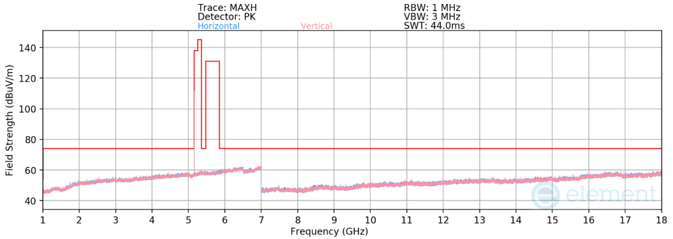
Plot 7-67. RSE 1-18GHz Antenna WF5B (BDR GFSK ePA – 5162MHz)
