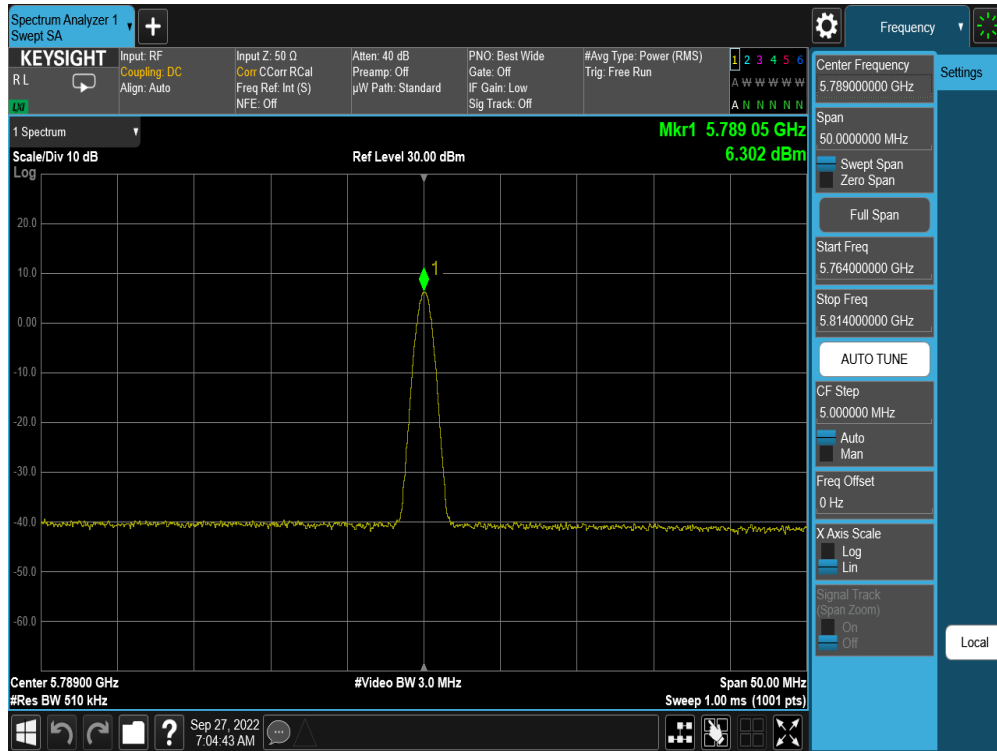
Plot 7-35. PSD Antenna WF5B (BDR GFSK, iPA – 5789MHz)
