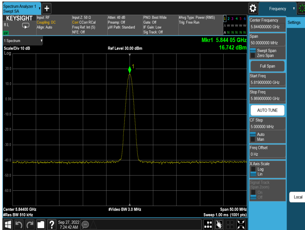
Plot 7-54. PSD TxBF Antenna WF5B (BDR GFSK, ePA – 5844MHz)
