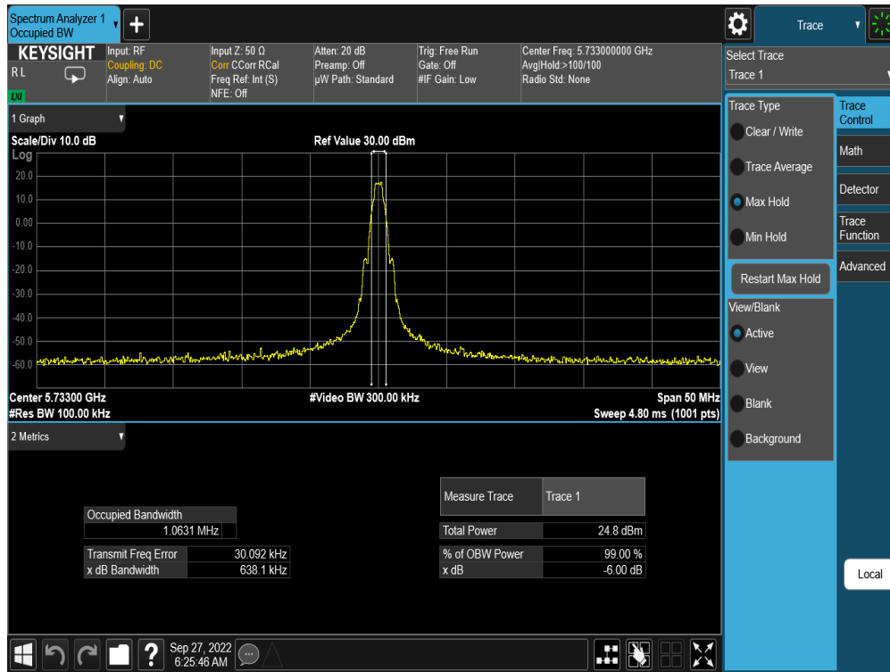
Plot 7-7. 6dB BW & 99% OBW Antenna WF5T (BDR GFSK, ePA – 5733MHz)
