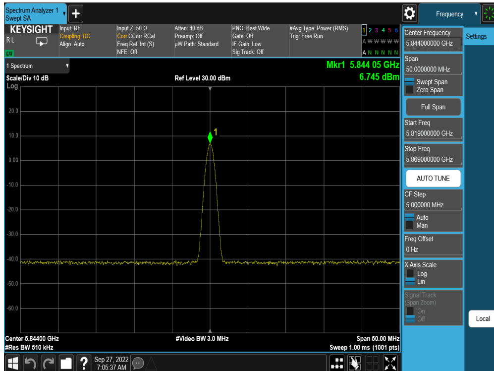
Plot 7-36. PSD Antenna WF5B (BDR GFSK, iPA – 5844MHz)
