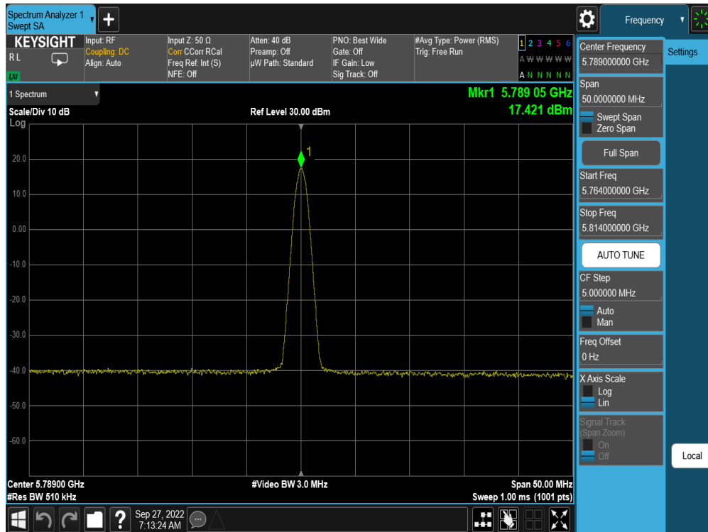
Plot 7-32. PSD Antenna WF5B (BDR GFSK, ePA – 5789MHz)
