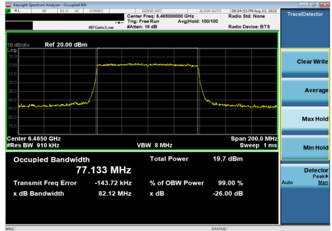
Plot 7-28. 26dB & 99% Bandwidth Plot Antenna 5b (80MHz 802.11ax RU96 (UNII Band 6) – Ch. 103)
