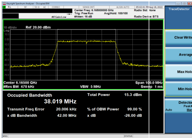
Plot 7-8. 26dB & 99% Bandwidth Plot Antenna 5b (40MHz 802.11ax RU484 (UNII Band 5) – Ch. 43)
