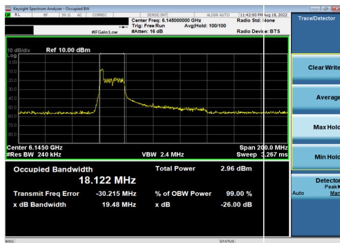
Plot 7-9. 26dB & 99% Bandwidth Plot Antenna 5b (80MHz 802.11ax RU26 (UNII Band 5) – Ch. 39)
