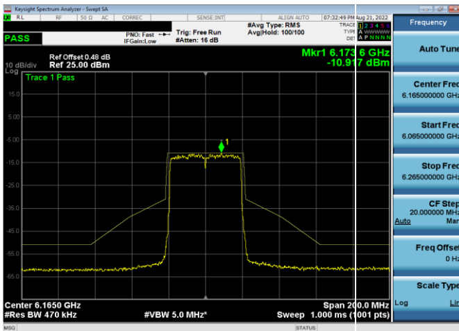
Plot 7-419. In-Band Emission Plot Antenna 4a (40MHz 802.11ax (UNII Band 5) – Ch. 43, MCS4)
