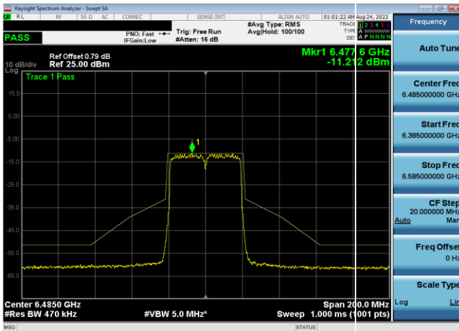
Plot 7-440. In-Band Emission Plot Antenna 4a (40MHz 802.11ax (UNII Band 6) – Ch. 107, MCS11)
