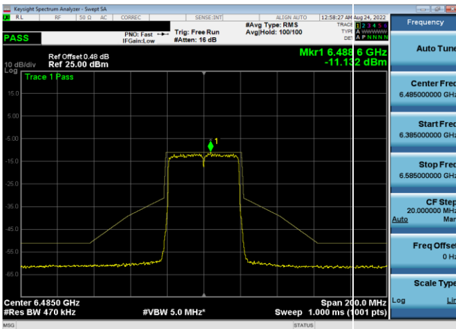
Plot 7-424. In-Band Emission Plot Antenna 4a (40MHz 802.11ax (UNII Band 6) – Ch. 107, MCS4)
