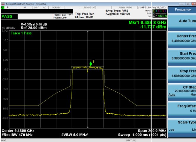
Plot 7-364. In-Band Emission Plot Antenna 5b (40MHz 802.11ax (UNII Band 6) – Ch. 107, MCS4)
