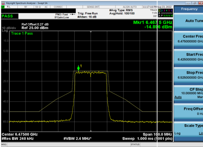
Plot 7-363. In-Band Emission Plot Antenna 5b (20MHz 802.11ax (UNII Band 6) – Ch. 105, MCS4)
