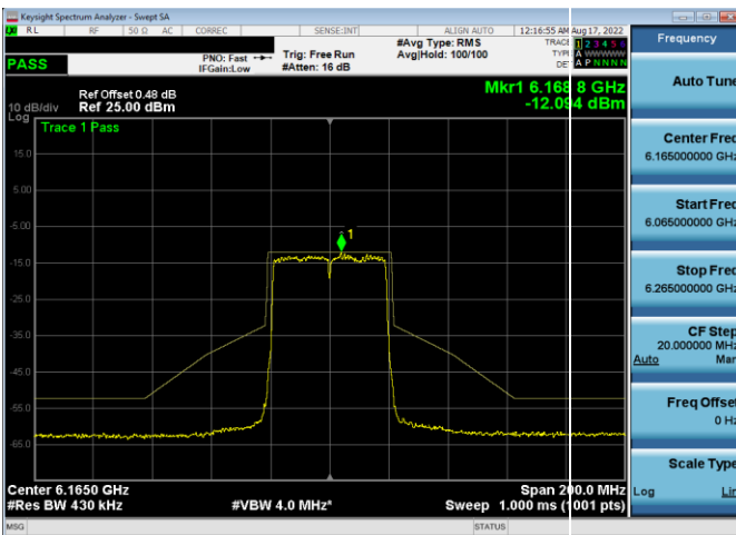
Plot 7-359. In-Band Emission Plot Antenna 5b (40MHz 802.11ax (UNII Band 5) – Ch. 43, MCS4)
