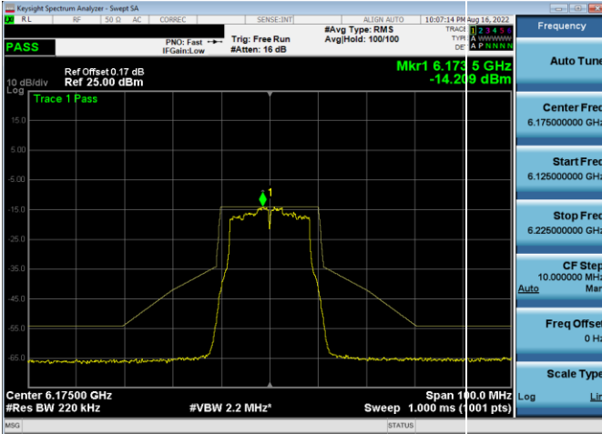
Plot 7-357. In-Band Emission Plot Antenna 5b (20MHz 802.11a (UNII Band 5) – Ch. 45, 24Mbps)
