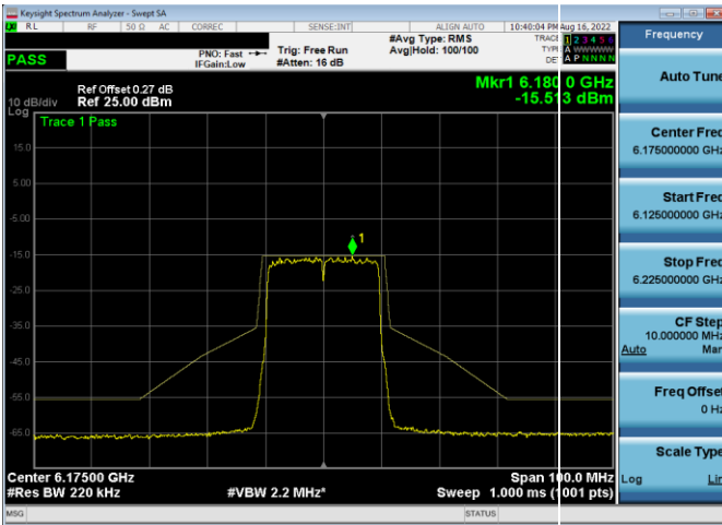
Plot 7-358. In-Band Emission Plot Antenna 5b (20MHz 802.11ax (UNII Band 5) – Ch. 45, MCS4)
