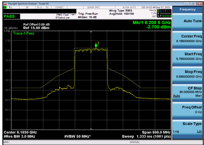
Plot 7-361. In-Band Emission Plot Antenna 5b (160MHz 802.11ax (UNII Band 5) – Ch. 47, MCS4)
