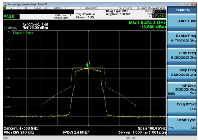
Plot 7-362. In-Band Emission Plot Antenna 5b (20MHz 802.11a (UNII Band 6) – Ch. 105, 24Mbps)
