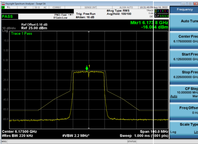
Plot 7-338. In-Band Emission Plot Antenna 5b (20MHz 802.11ax (UNII Band 5) – Ch. 45, MCS2)
