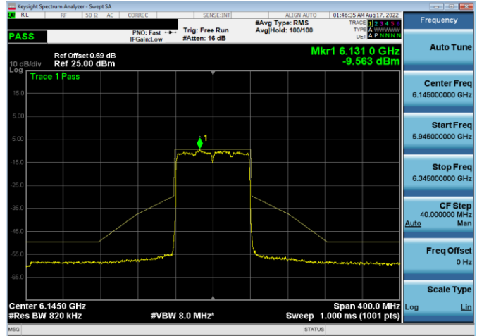
Plot 7-360. In-Band Emission Plot Antenna 5b (80MHz 802.11ax (UNII Band 5) – Ch. 39, MCS4)
