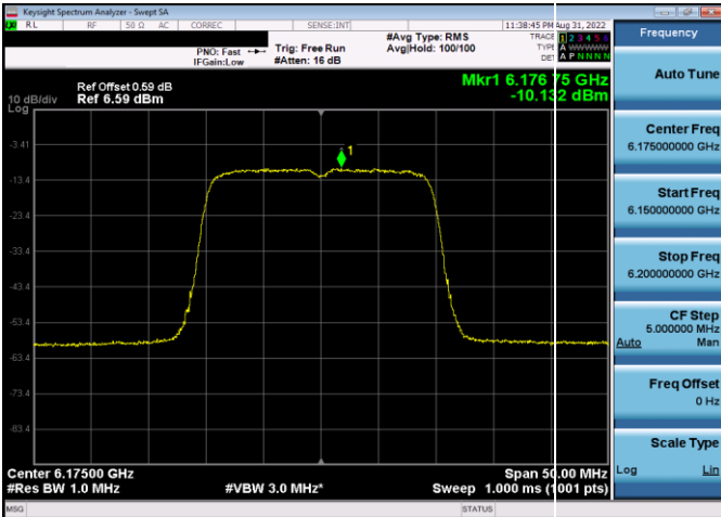
Plot 7-305. Power Spectral Density Plot SDM Antenna 5b (20MHz 802.11ax (UNII Band 5) – Ch. 45, MCS11)
