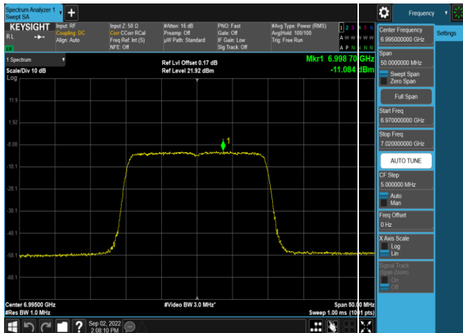
Plot 7-266. Power Spectral Density Plot SDM Antenna 4a (20MHz 802.11ax (UNII Band 8) – Ch. 209, MCS2)
