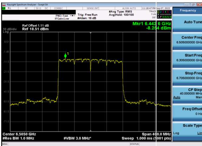
Plot 7-319. Power Spectral Density Plot SDM Antenna 5b (160MHz 802.11ax (UNII Band 6) – Ch. 111, MCS11)
