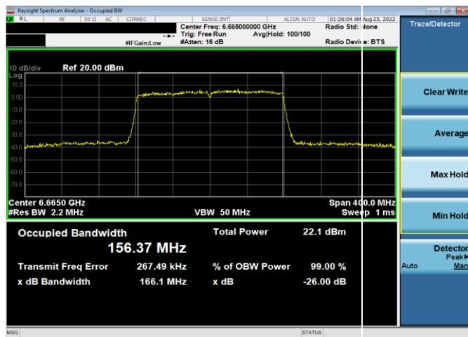
Plot 7-15. 26dB & 99% Bandwidth Plot Antenna 5b (160MHz 802.11ax (UNII Band 7) – Ch. 143, MCS2)
