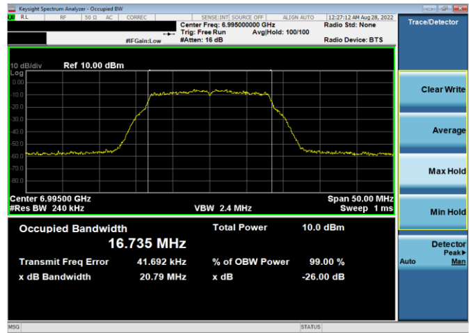
Plot 7-16. 26dB & 99% Bandwidth Plot Antenna 5b (20MHz 802.11a (UNII Band 8) – Ch. 209, 12Mbps)
