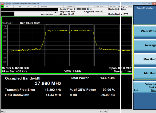
Plot 7-43. 26dB & 99% Bandwidth Plot Antenna 5b (40MHz 802.11ax (UNII Band 5) – Ch. 43, MCS11)
