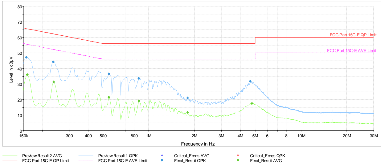
Plot 7-745. AC Line Conducted Plot with 802.11ax SDM – Ch. 1 (N), with AC/DC adapter
