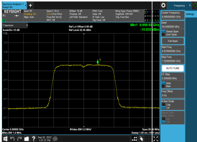
Plot 7-330. Power Spectral Density Plot SDM Antenna 4a (20MHz 802.11ax (UNII Band 8) – Ch. 209, MCS11)
