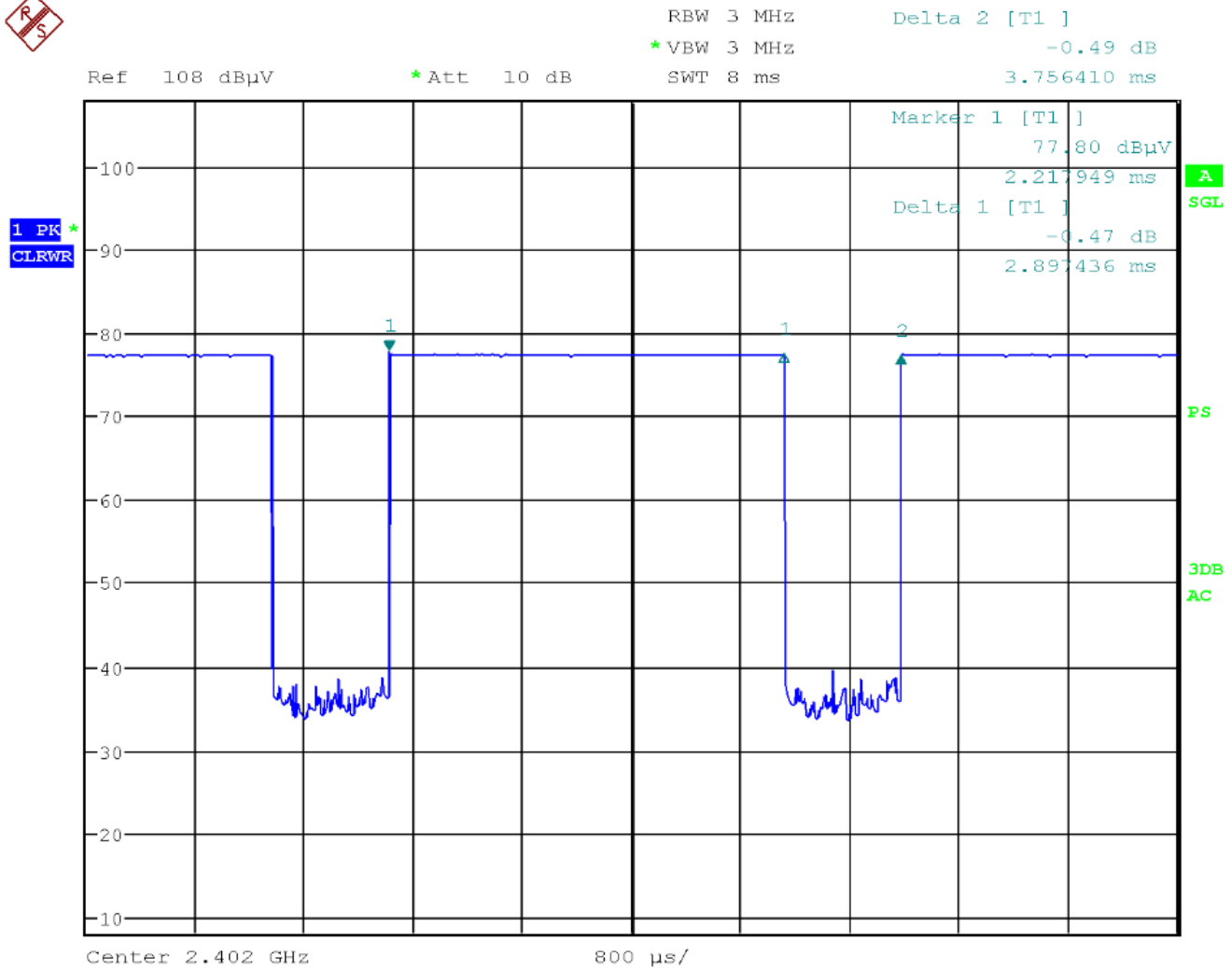
Figure 8-5 Bluetooth Transmission Plot & Duty Cycle Calculation – Antenna A Variant 1
