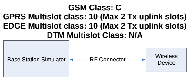
Figure 8-1 Power Measurement Setup
