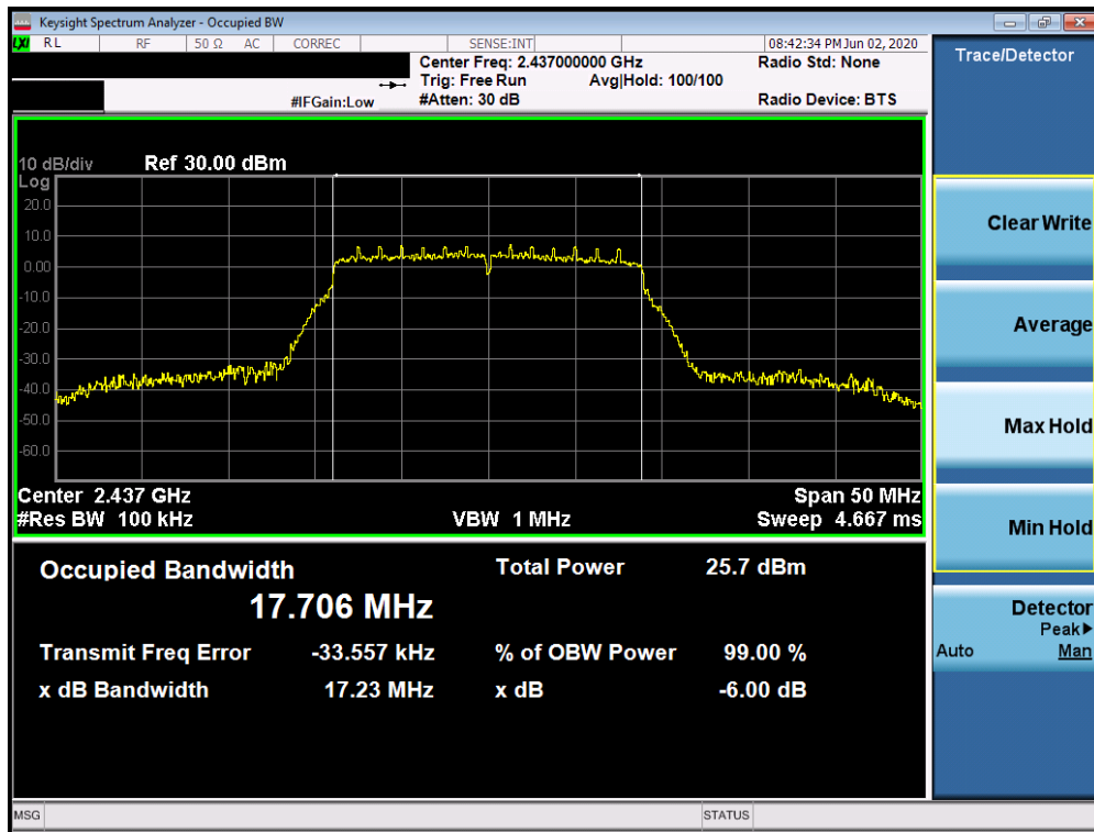
Plot 7-8. 6dB Bandwidth Plot SISO CORE 0 (802.11n (2.4GHz) – Ch. 6)
