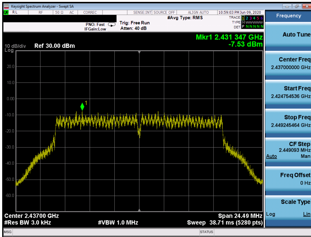
Plot 7-39. Power Spectral Density Plot CDD CORE 0 (802.11g – Ch. 6)
