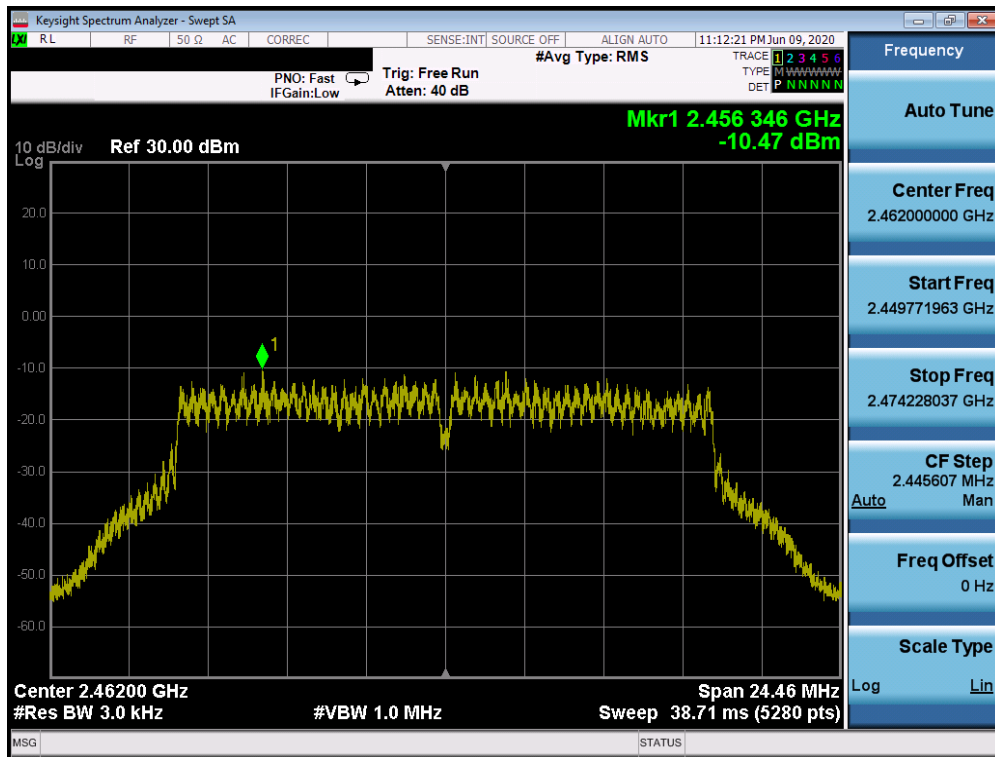
Plot 7-42. Power Spectral Density Plot CDD CORE 1 (802.11g – Ch. 11)
