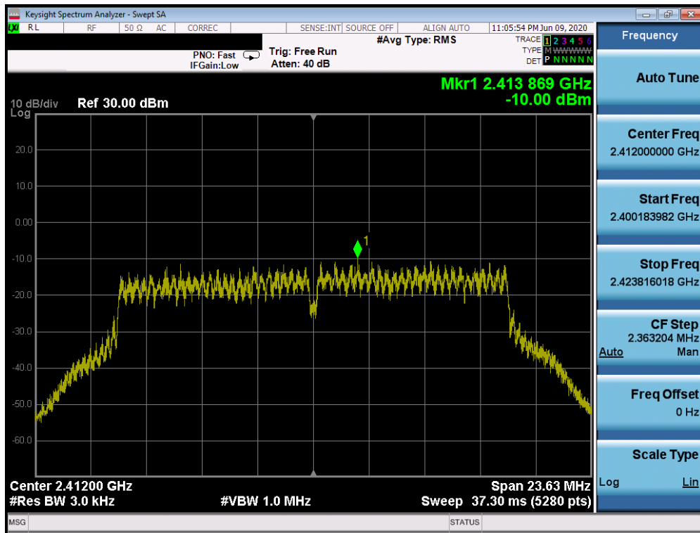
Plot 7-38. Power Spectral Density Plot CDD CORE 1 (802.11g – Ch. 1)
