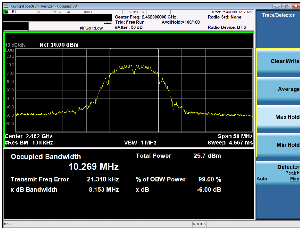
Plot 7-12. 6dB Bandwidth Plot SISO CORE 1 (802.11b – Ch. 11)
