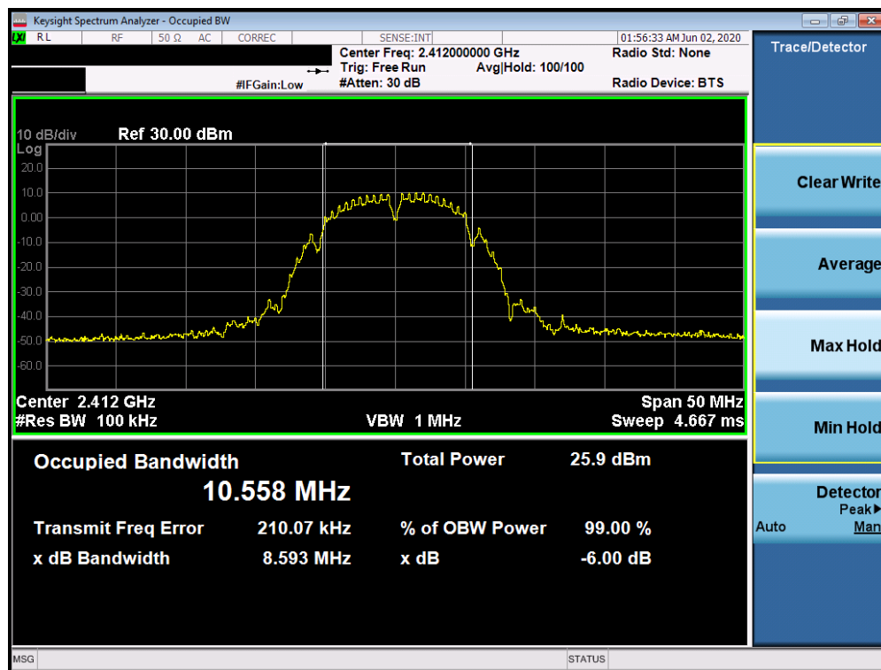
Plot 7-10. 6dB Bandwidth Plot SISO CORE 1 (802.11b – Ch. 1)
