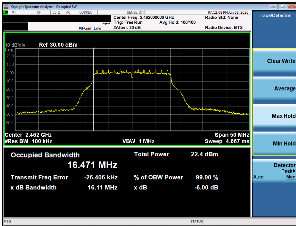
Plot 7-6. 6dB Bandwidth Plot SISO CORE 0 (802.11g – Ch. 11)
