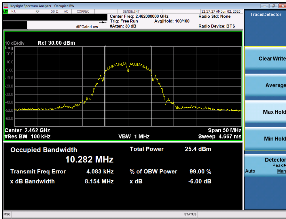
Plot 7-3. 6dB Bandwidth Plot SISO CORE 0 (802.11b – Ch. 11)
