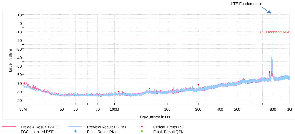
Plot 7-45. Radiated Spurious Emissions Below 1GHz (Band 14)
