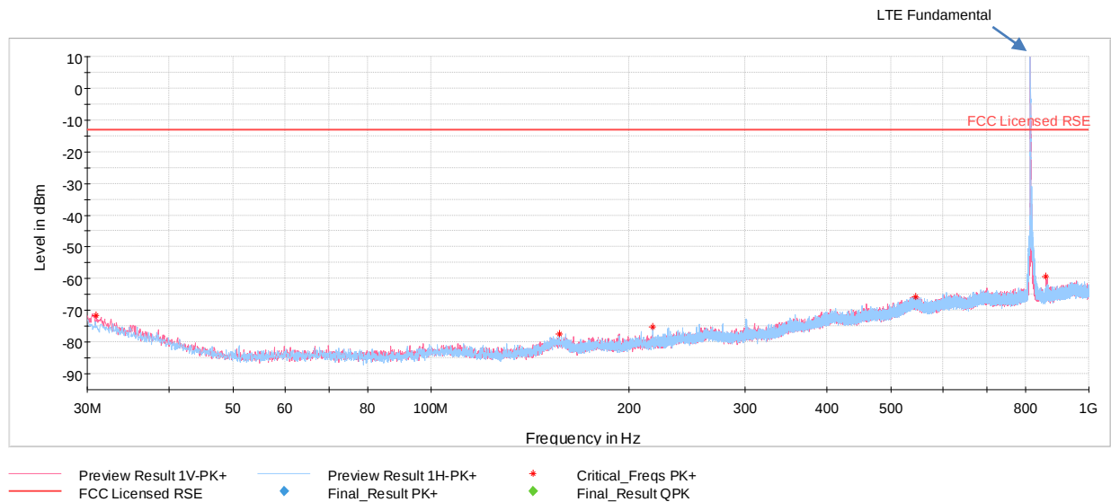
Plot 7-43. Radiated Spurious Emissions Below 1GHz (Band 26)
